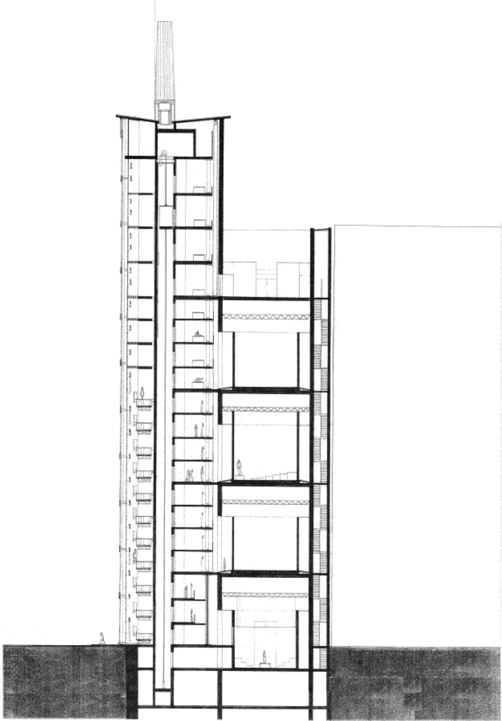
cross section through elevator
