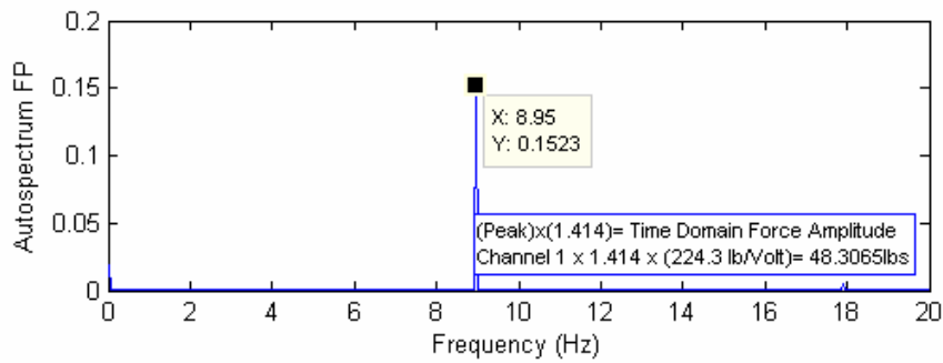
Time History and Autospectrum of Accelerometer Data
