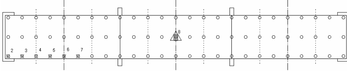
Three Span Floor- Stage 4- Interior Bottom Chord Extensions Re-installed- Test 127
