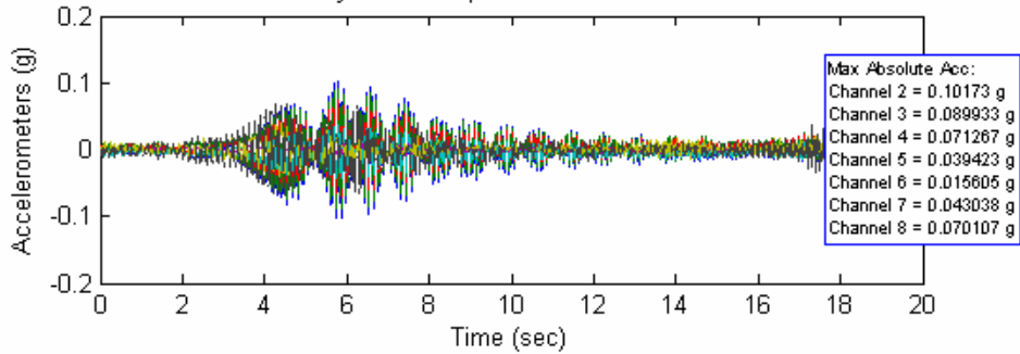
Time History and Autospectrum of Accelerometer Data
