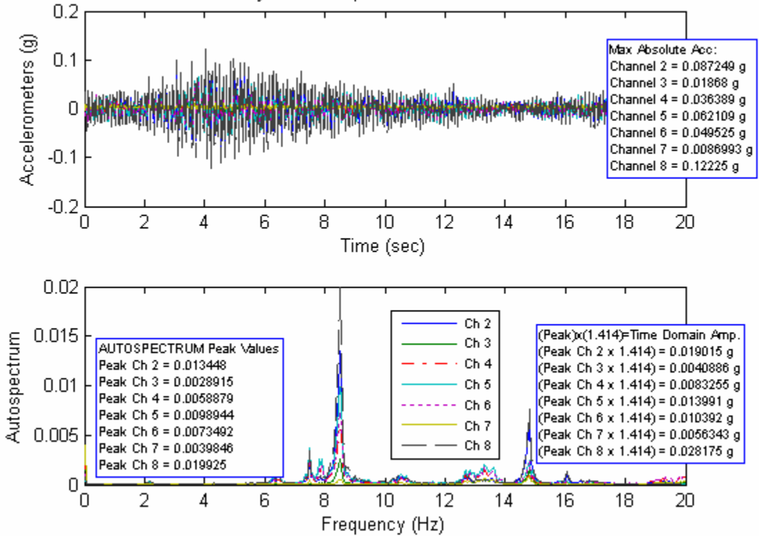
Time History and Autospectrum of Accelerometer Data
