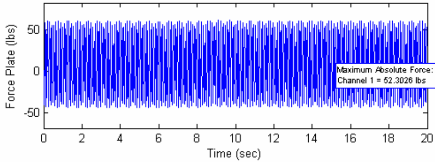
Force Plate Time History and Autospectrum
