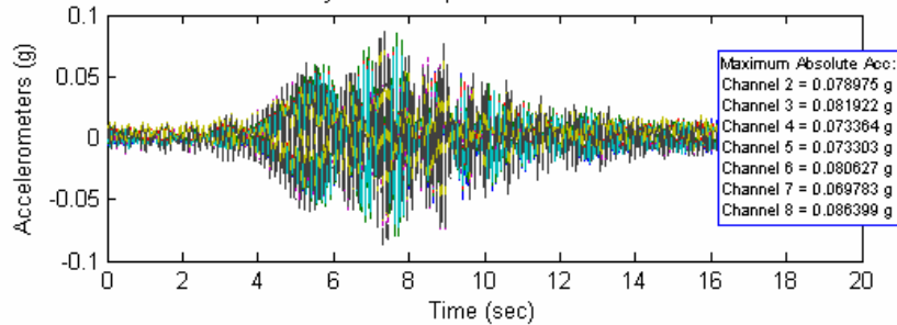
Time History and Autospectrum of Accelerometer Data
