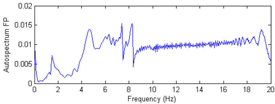
Time History and Autospectrum of Accelerometer Data
