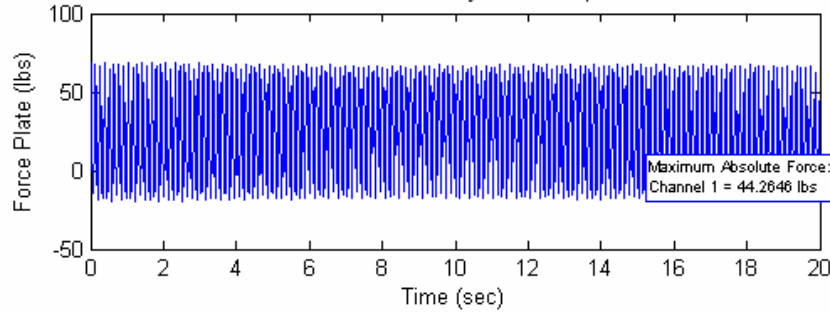
Force Plate Time History and Autospectrum
