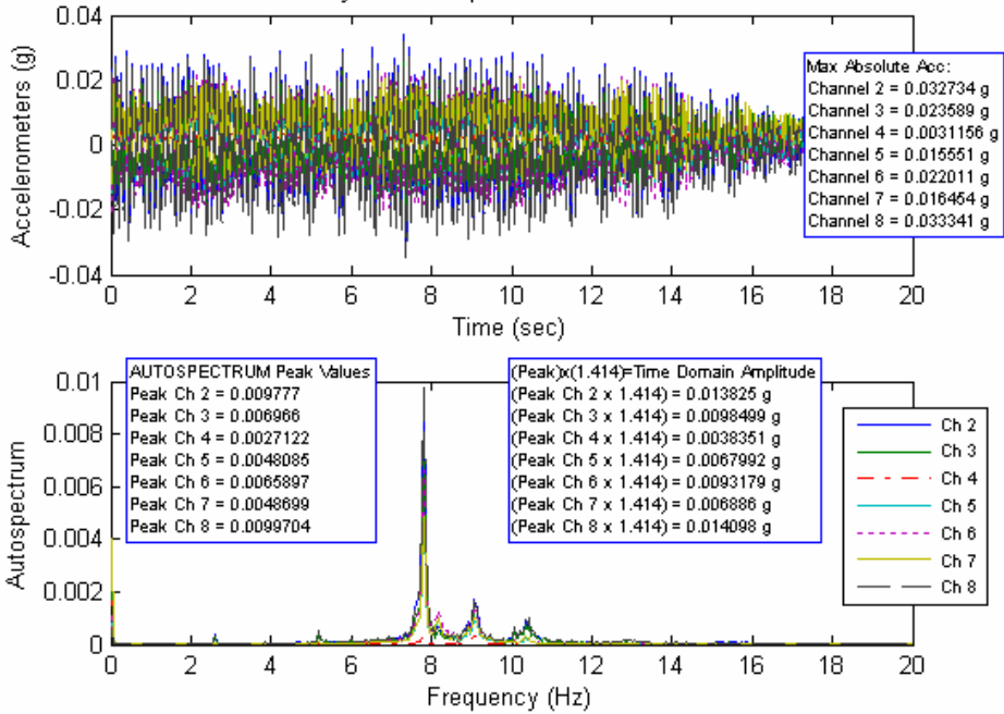
Time History and Autospectrum of Accelerometer Data
