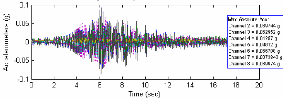
Time History and Autospectrum of Accelerometer Data
