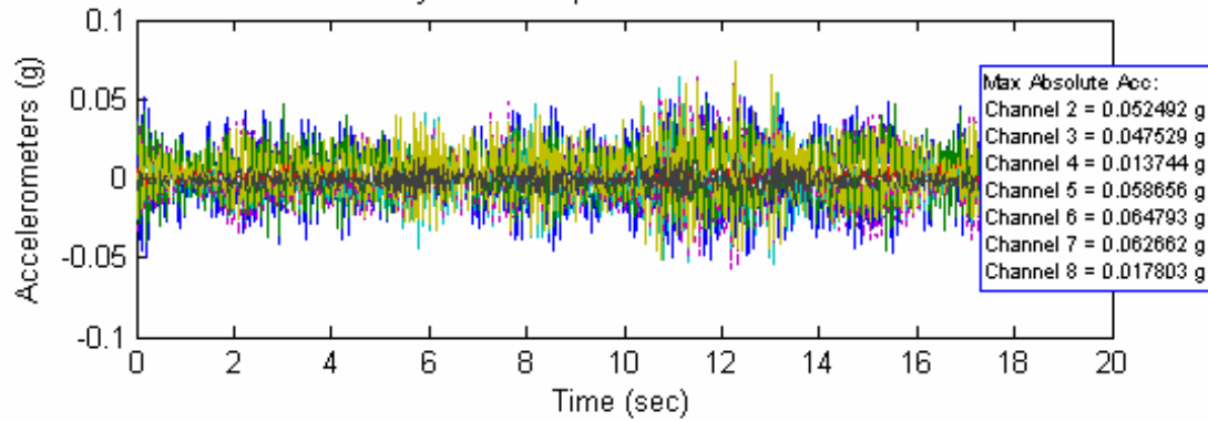
Time History and Autospectrum of Accelerometer Data
