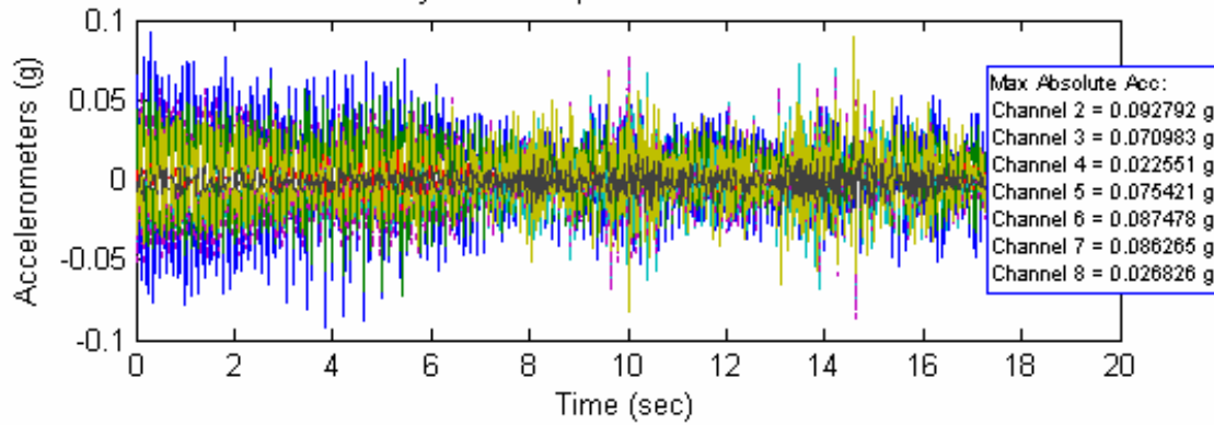
Time History and Autospectrum of Accelerometer Data
