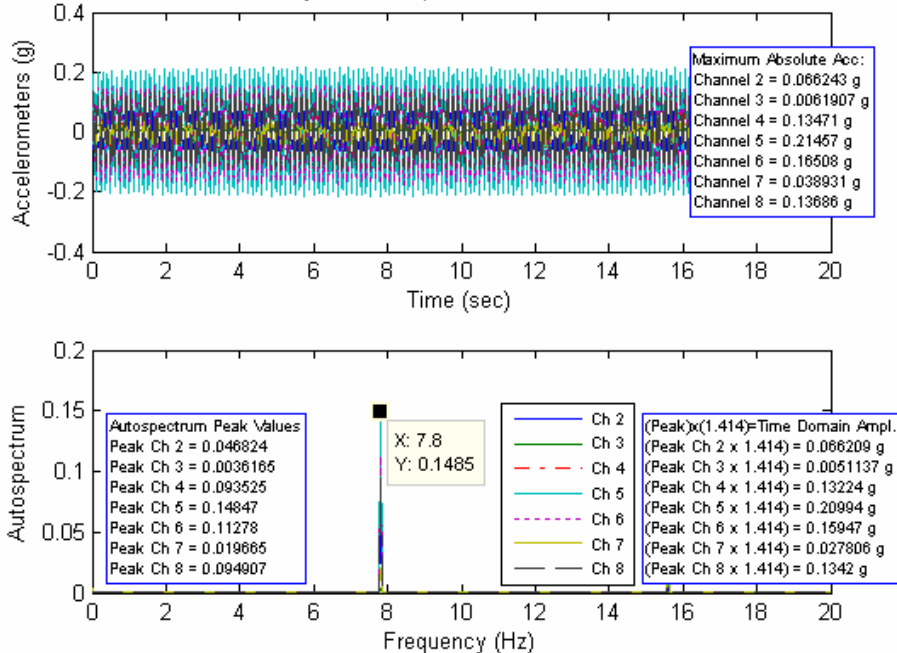
Time History and Autospectrum of Accelerometer Data
