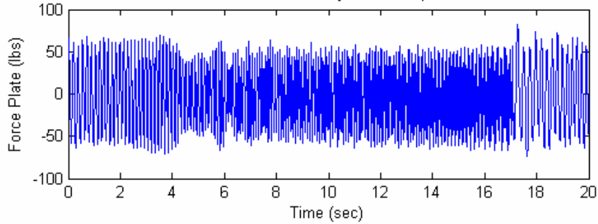
Force Plate Time History and Autospectrum
