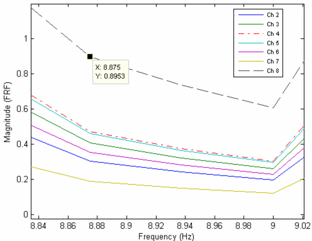
Frequency Response Functions: Magnitude
