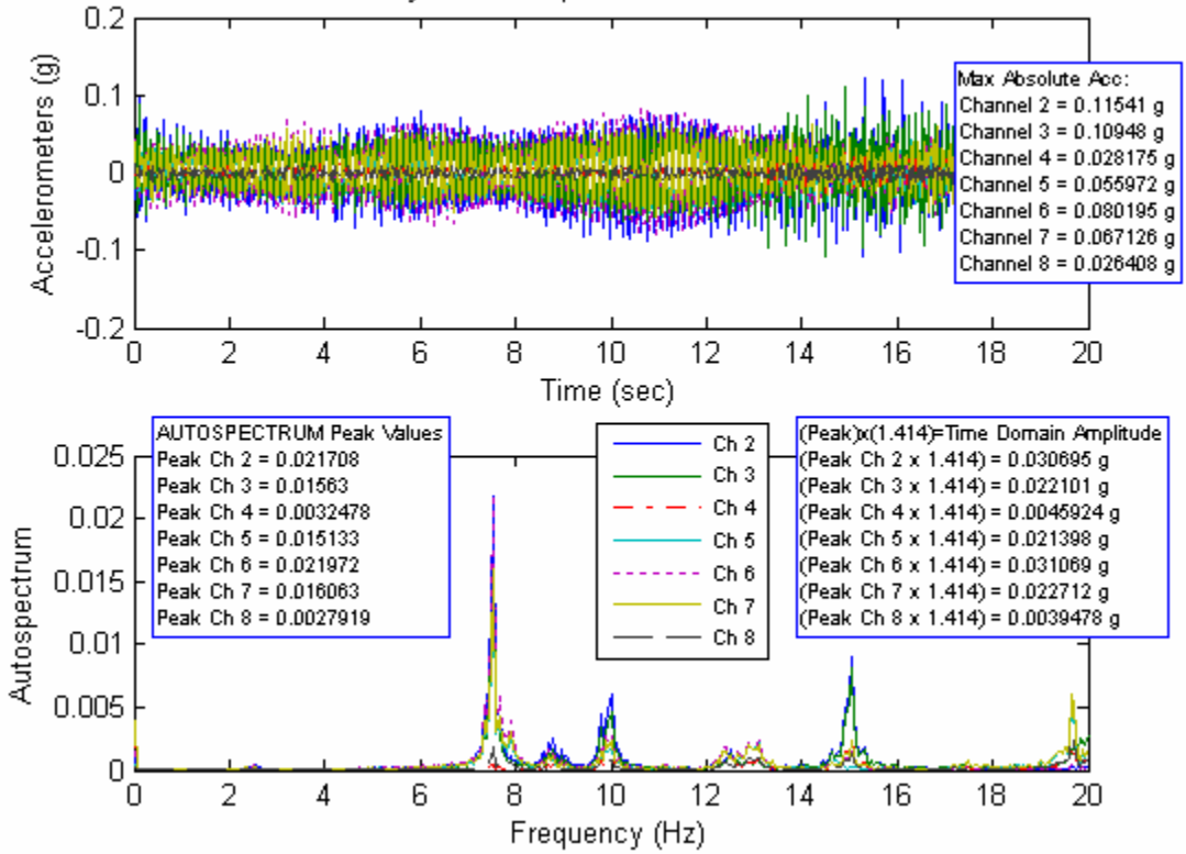
Time History and Autospectrum of Accelerometer Data
