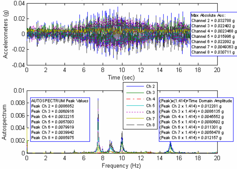
Time History and Autospectrum of Accelerometer Data
