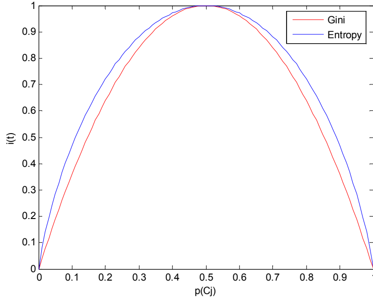
Figure 3-4. Comparison between Gini and Entropy impurity functions. Both functions reach a maximum when classes are equally mixed and achieve a minimum when only one class is present.
