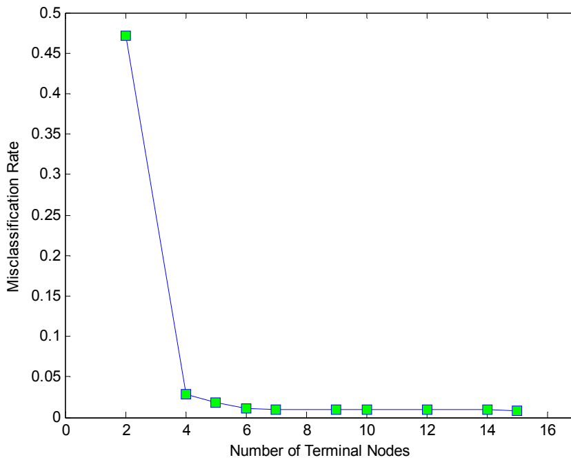
Figure 5-14. Misclassification rate for the sequence of subtrees.
