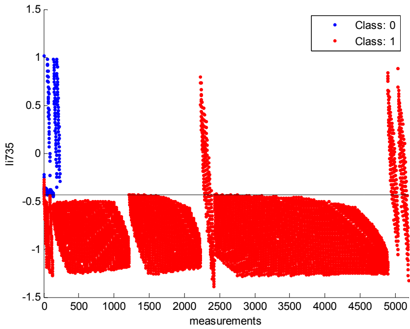
Figure B-11. Split at node 3.
