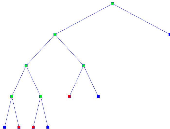
Figure 3-7. Optimal subtree T_5 . The tree achieves the minimum error rate.
