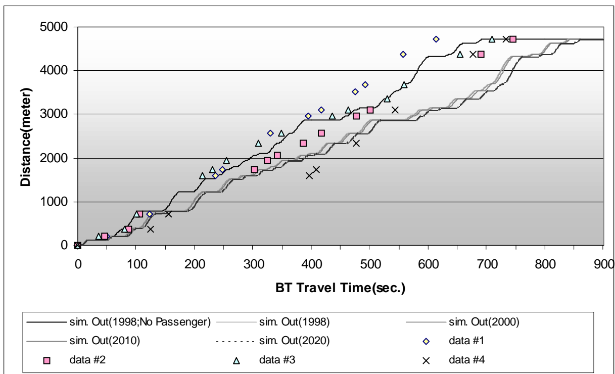
Figure E.15 Comparison Between Observed Data and Model Output (Section 1).
