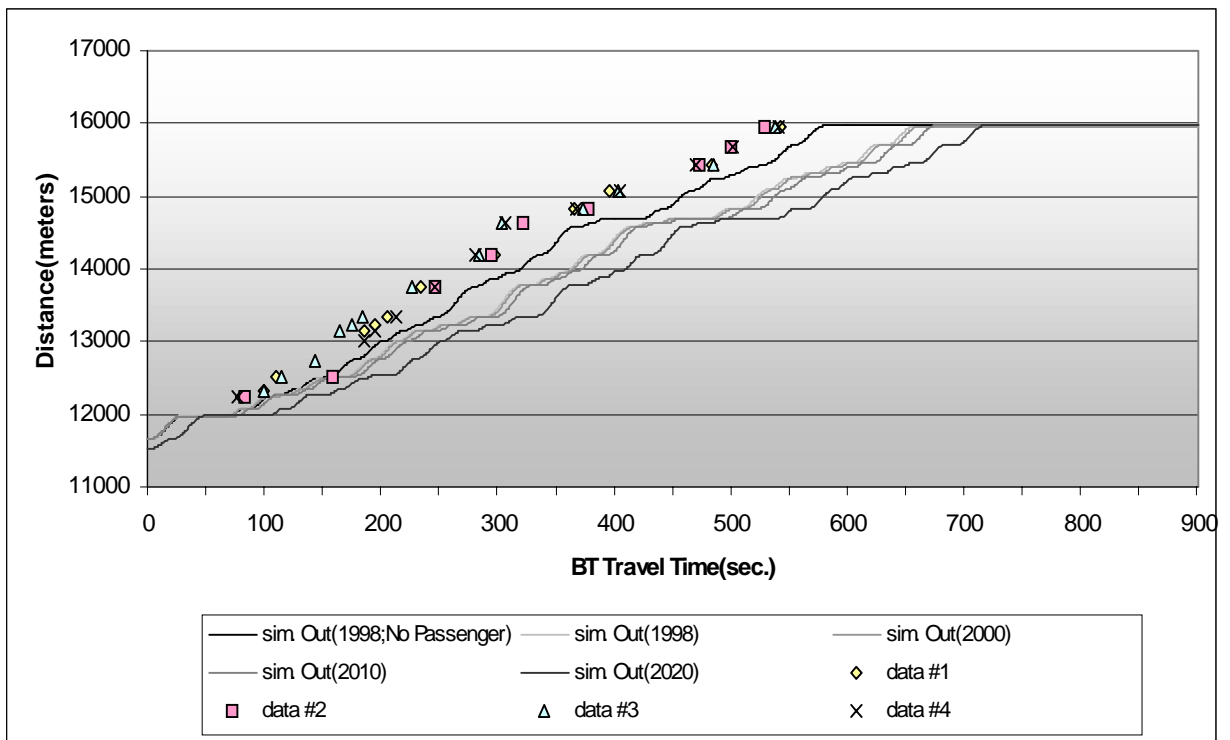
Figure E.18 Comparison Between Observed Data and Model Output (Section 4).
