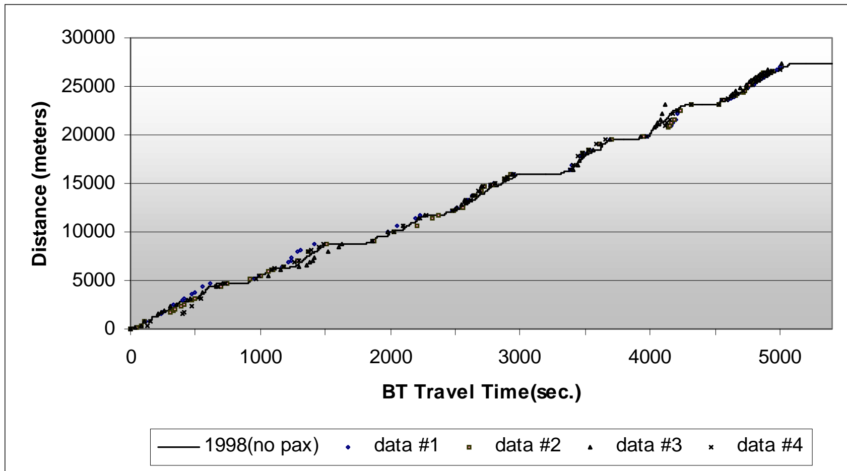
Figure E.13 Graphical Comparison between On-Board Observation Data and Model Output.
