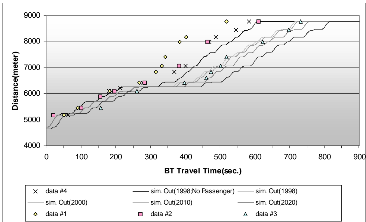
Figure E.16 Comparison Between Observed Data and Model Output (Section 2).
