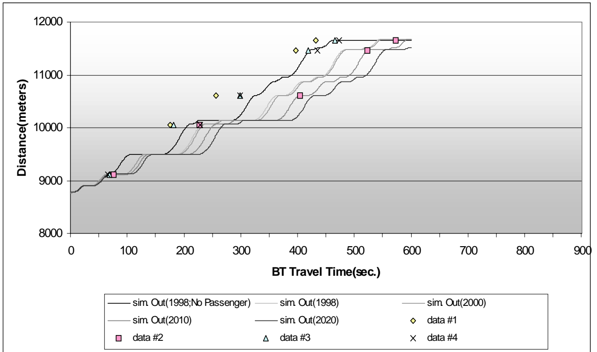
Figure E.17 Comparison Between Observed Data and Model Output (Section 3).
