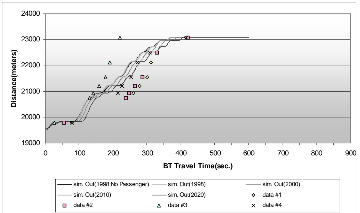
Figure E.20 Comparison Between Observed Data and Model Output (Section 6).
