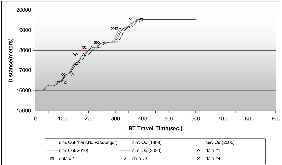
Figure E.19 Comparison Between Observed Data and Model Output (Section 5).
