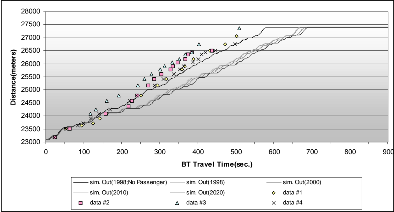
Figure E.21 Comparison Between Observed Data and Model Output (Section 7).
