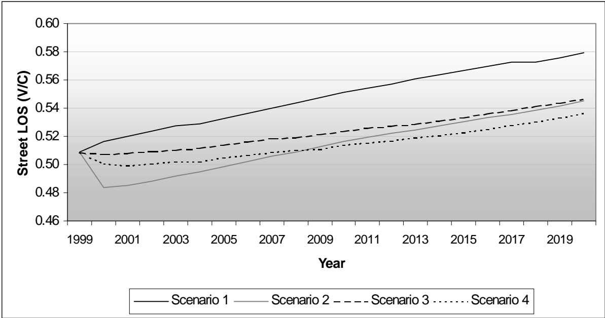
Figure F.1 Trends of Street LOS for Each Scenario.
