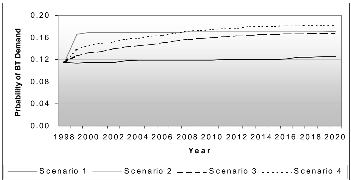
Figure F.4 Trends of BT Mode Choice Probability.
