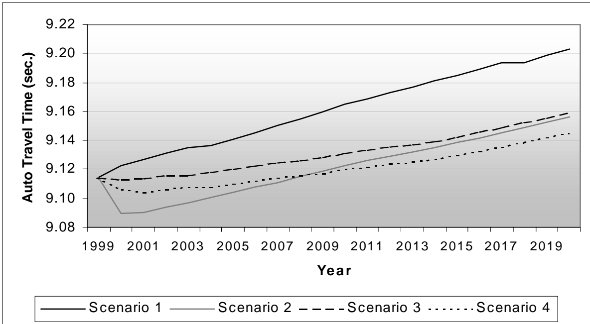
Figure F.2 Trends of Auto Travel Time for Each Scenario.
