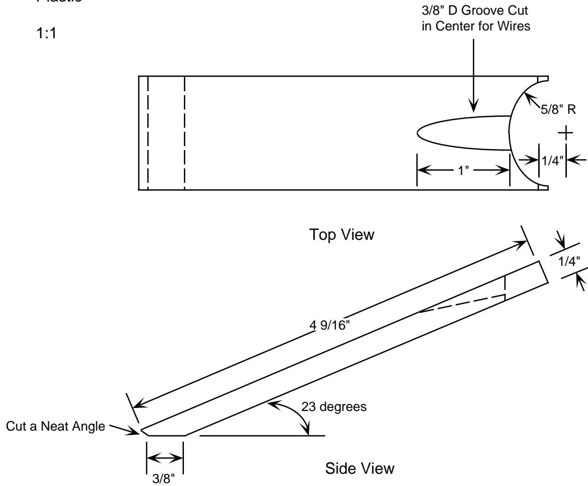
Figure A-10. Steering bar cover.
