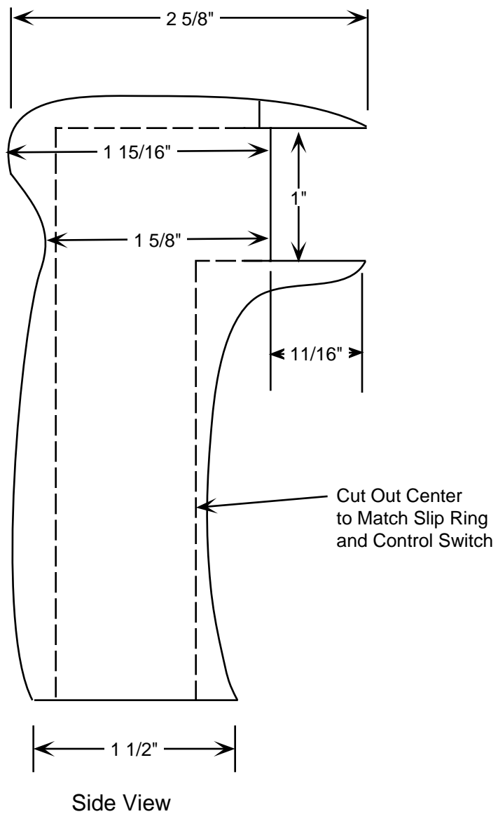
Figure A-11. Handle.
