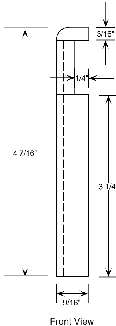
Figure A-11. Handle.
