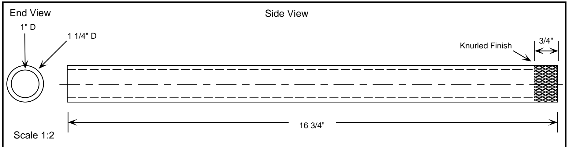
Figure A-14. Outer column tube.
