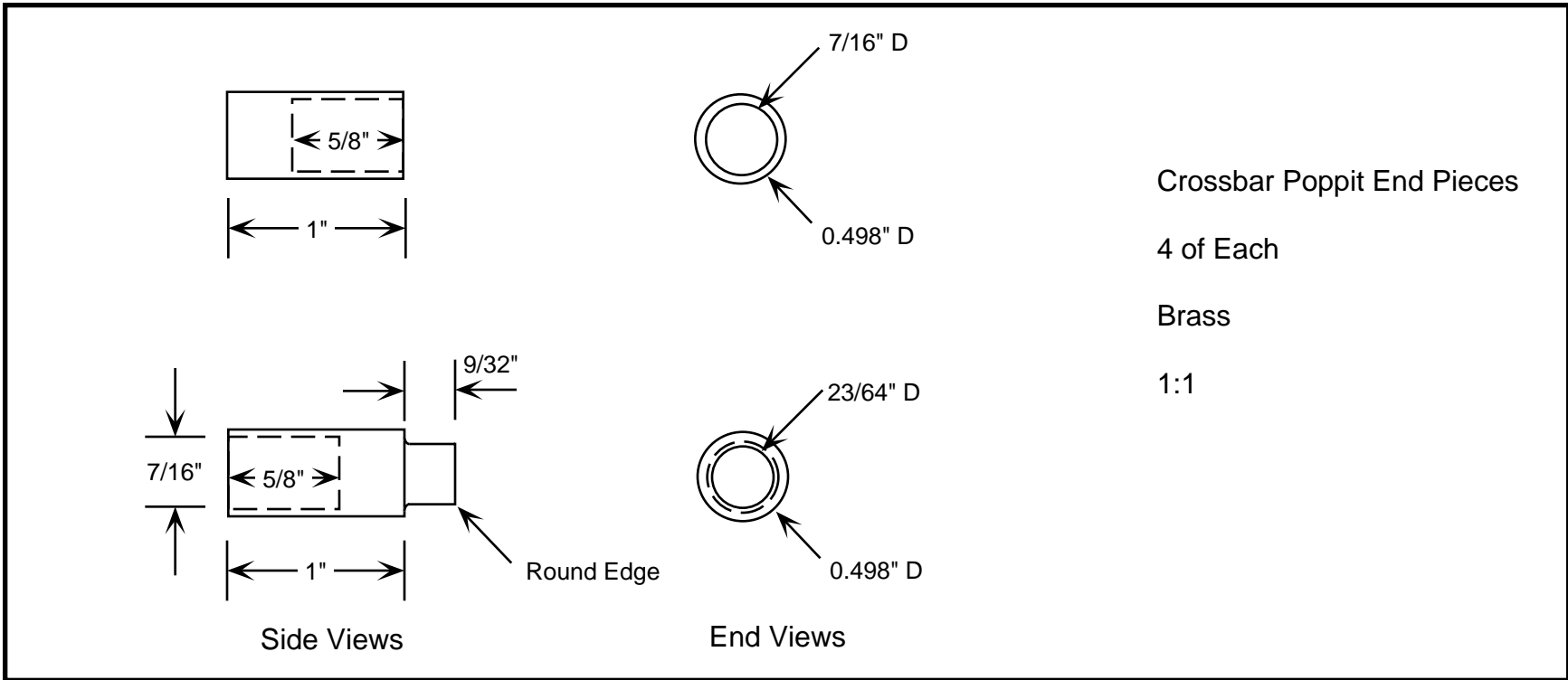
Figure A-16. Crossbar poppit inserts.
