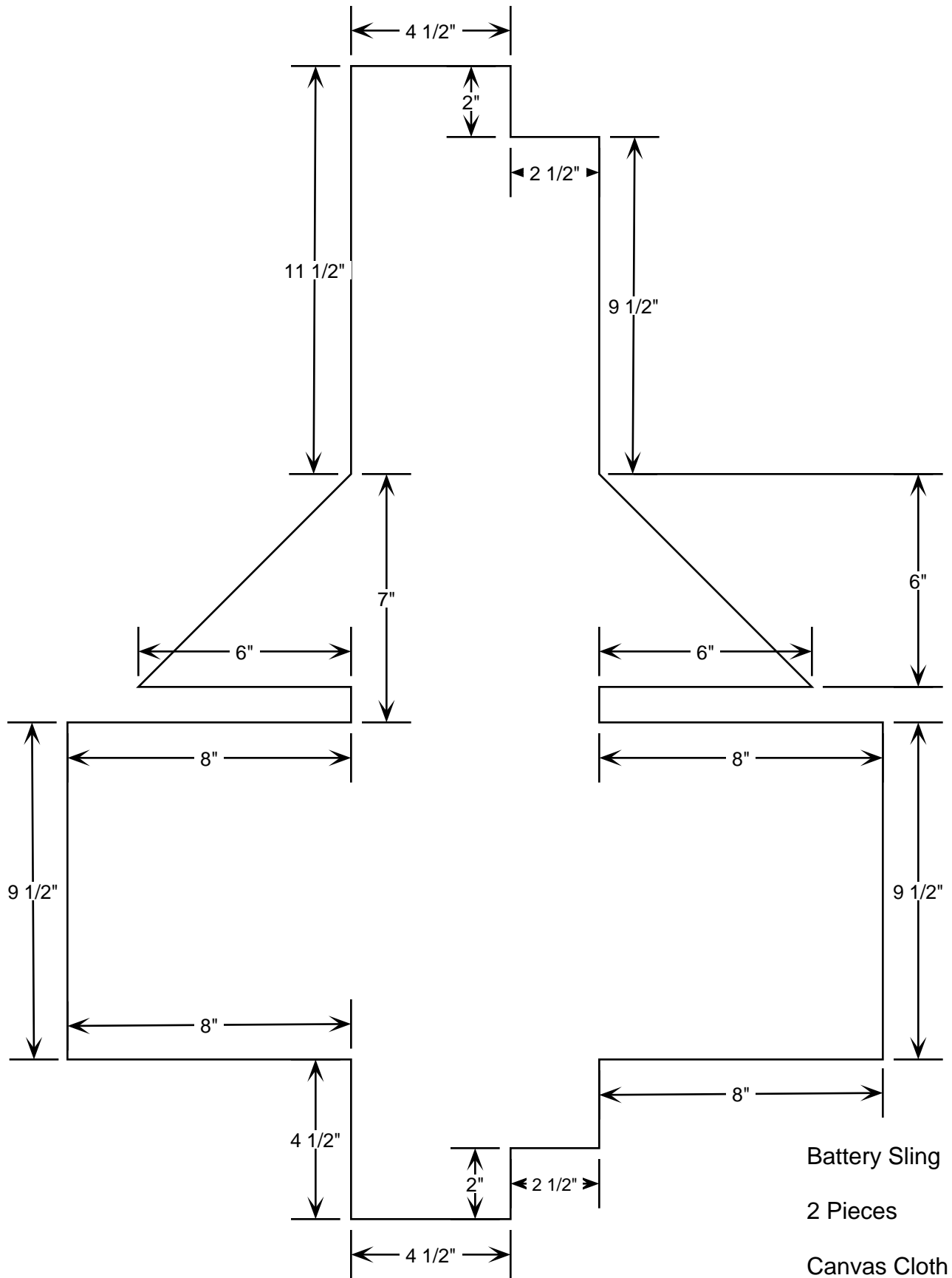
Figure A-31. Cloth pattern for battery sling.
