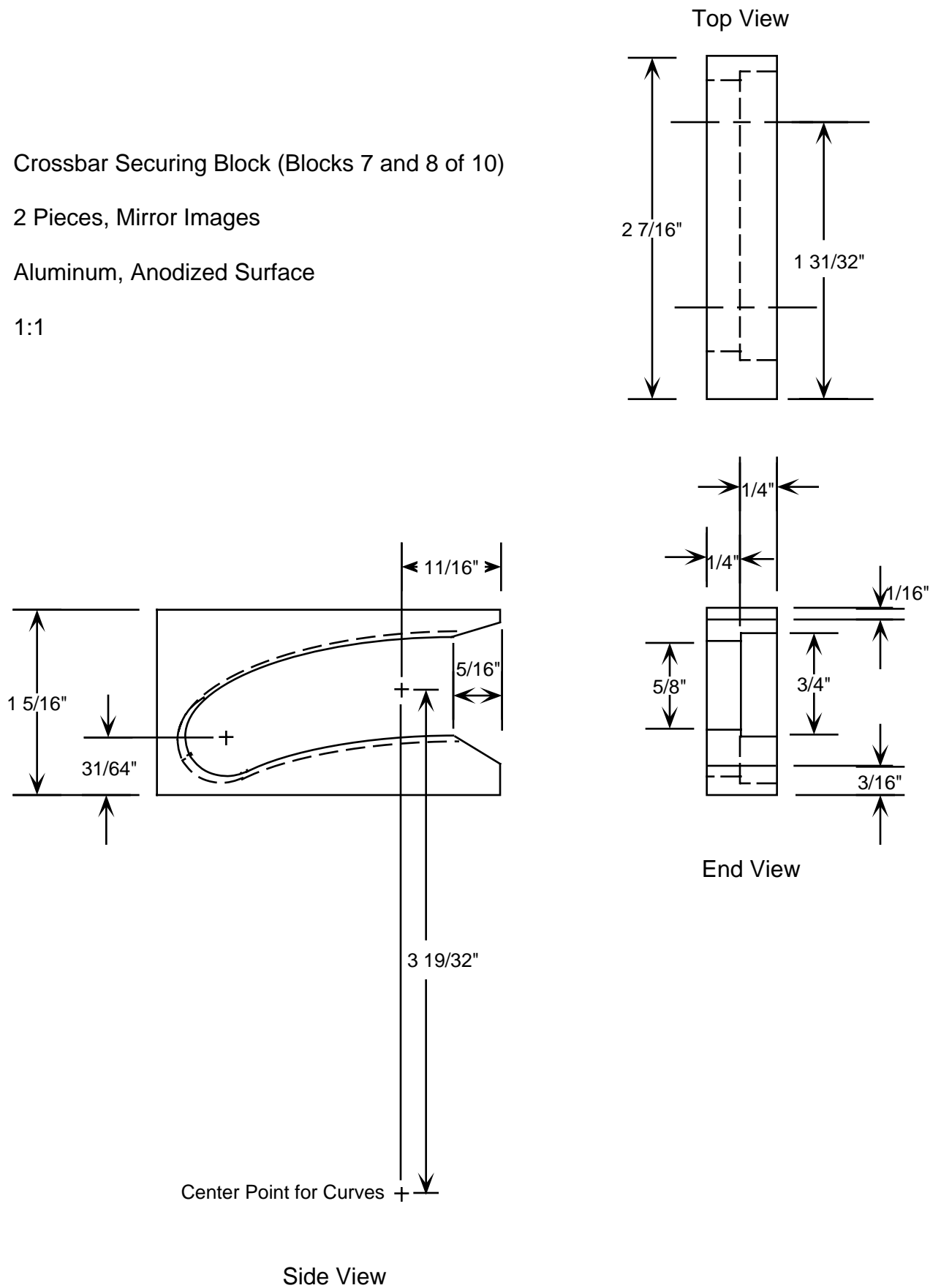
Figure A-7. Crossbar securing block (blocks 7 and 8 of 10).
