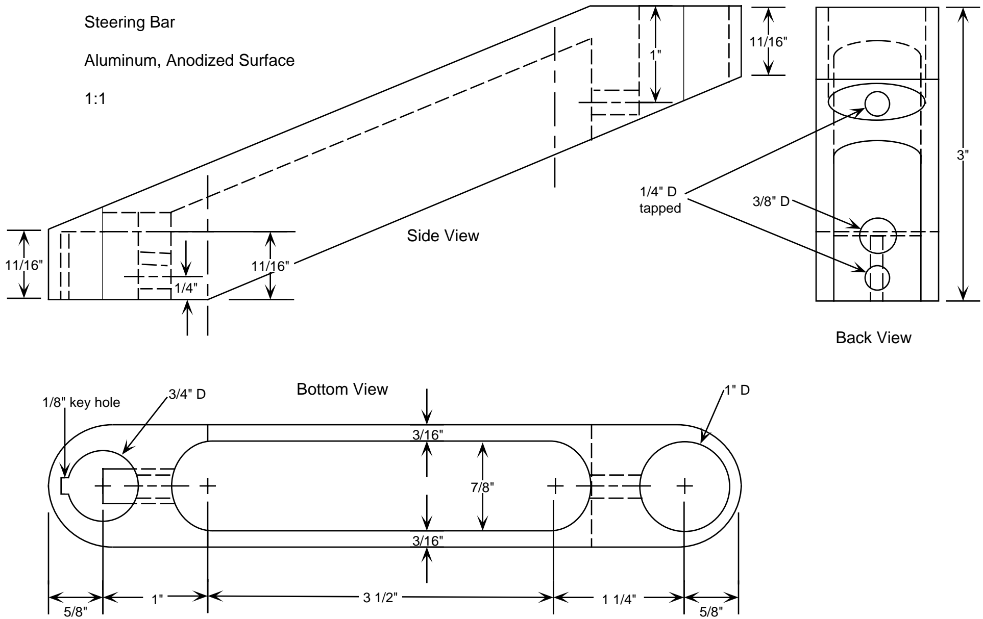
Figure A-9. Steering bar.
