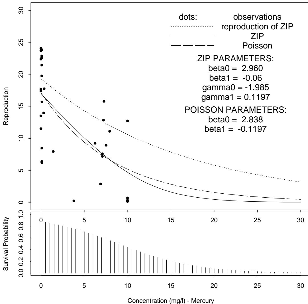
Figure 3.2. Survival probability/reproduction vs. Toxicant concentration
