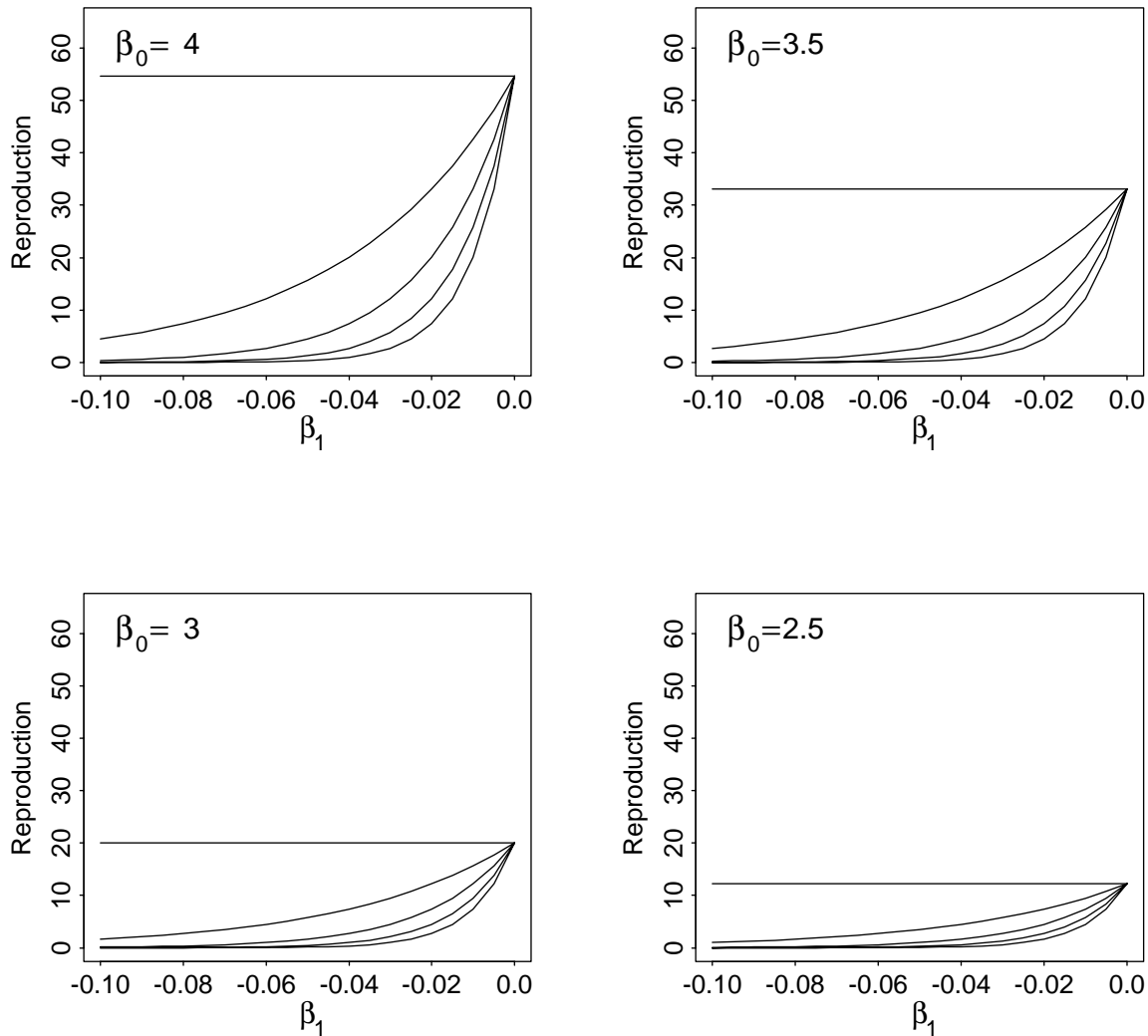
Figure 3.4. The mean response of the Poisson part of the ZIP model at different values of beta0 and beta1
