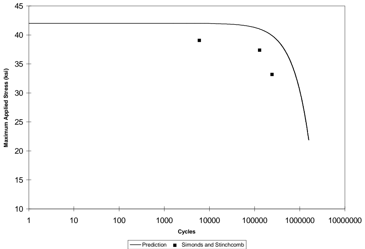
Figure 3.8. Comparison between predicted and measured remaining strength for quasi-isotropic APC-2 based on the data of Simonds and Stinchcomb [56].
