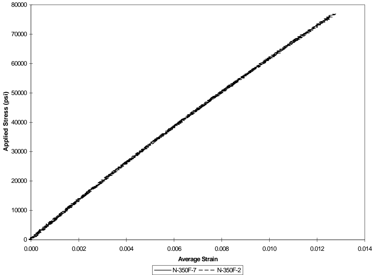
Figure 5.10. Stress-strain curves based on stroke measurements at 350°F (177°C) for [0/\pm 45]_{2s} IM7/K3B laminates containing a center hole.
