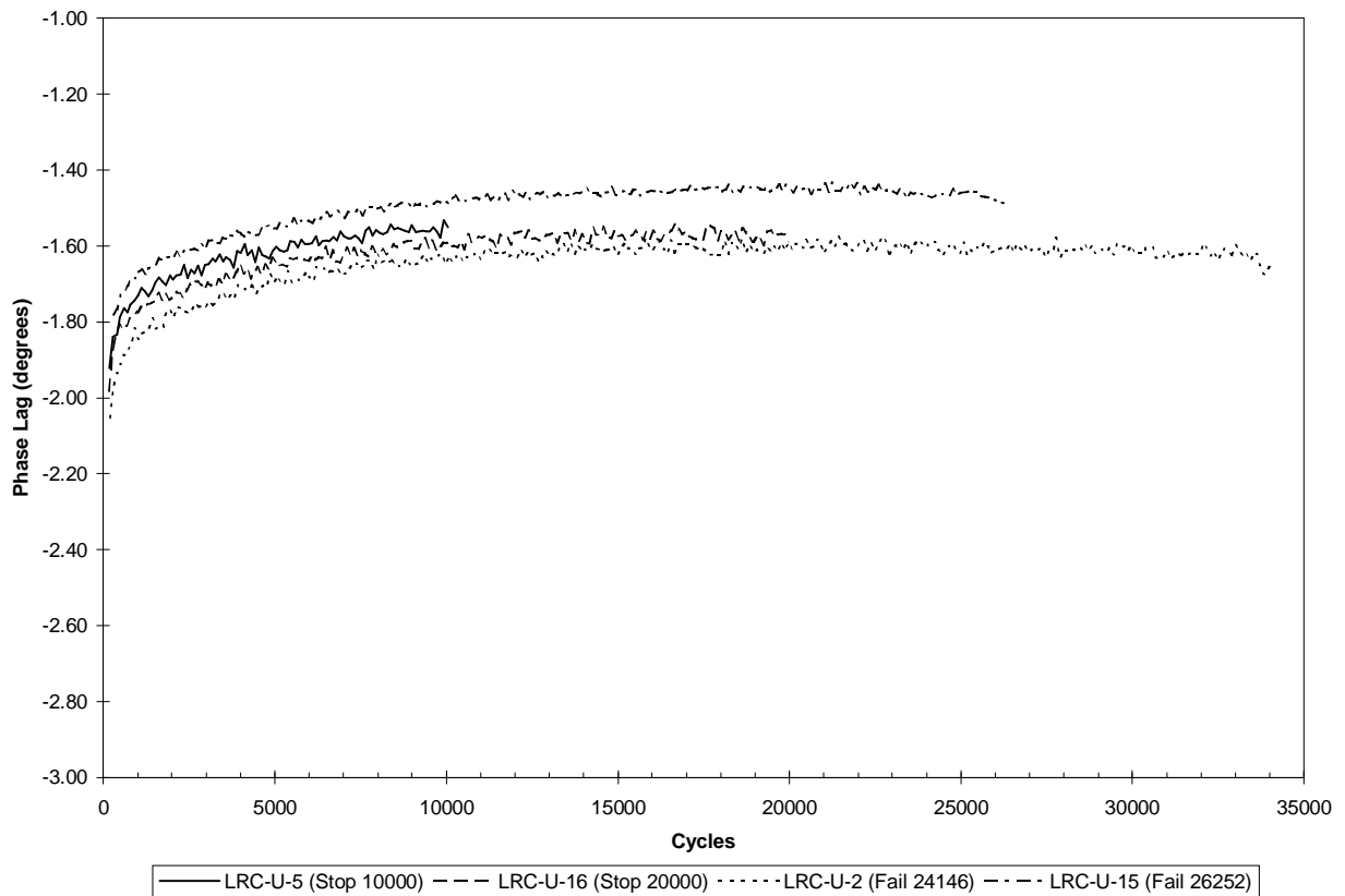
Figure 5.36. Phase lag measurements for room temperature fatigue tests at 65% of ultimate strength for [45/0/-45/90]_{2s} IM7/K3B laminates without a center hole.
