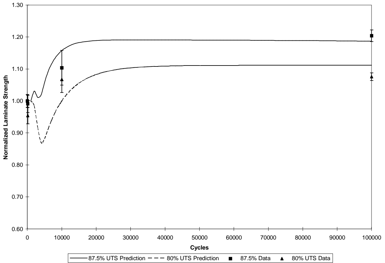
Figure 4.15. Comparison between predicted and measured remaining strength of cross-ply APC-2 laminates as a function of number of cycles.
