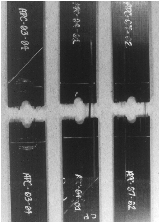
Figure 4.2. Failed cross-ply APC-2 quasi-static specimens.
