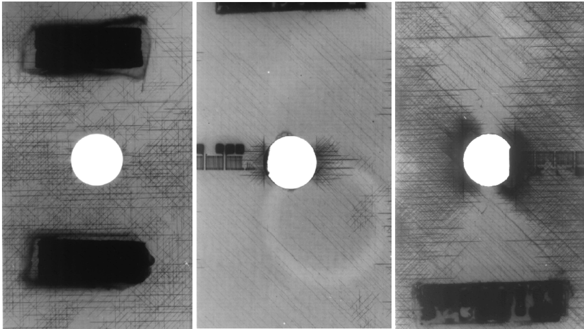
Figure 5.55. Penetrant-enhanced radiographs of notched [45/0/-45/90]_{2s} laminates of IM7/K3B fatigued at room temperature at 70% of ultimate tensile strength after 1000 cycles (left), 10000 cycles (center) and 100000 cycles (right).
