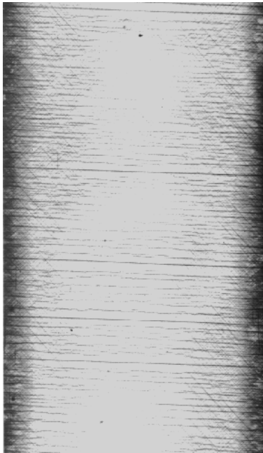
Figure 5.52. Penetrant-enhanced radiograph of an unnotched [45/0/-45/90]_2 laminate of IM7/K3B fatigued at room temperature at 70% of ultimate tensile strength after 10000 cycles.
