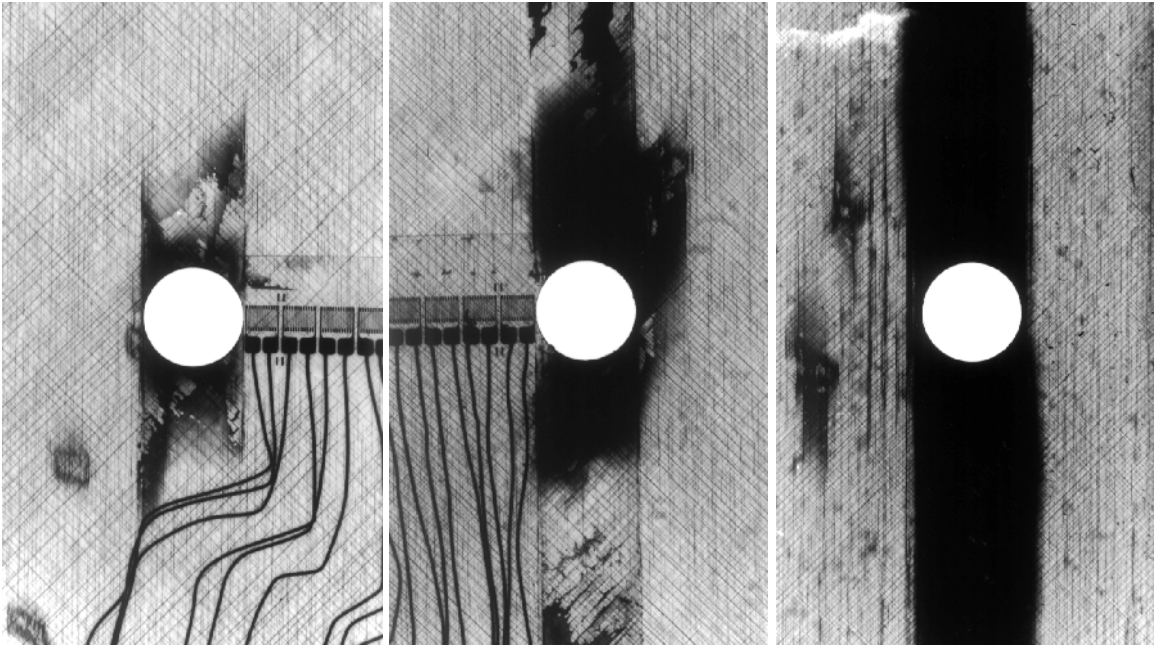
Figure 5.17. Penetrant-enhanced radiographs of [0/\pm 45]_{2s} laminates of IM7/K3B fatigued at 350°F (177°C) at 80% of ultimate tensile strength after 10000 cycles (left), 75000 cycles (center) and 224500 cycles (right).
