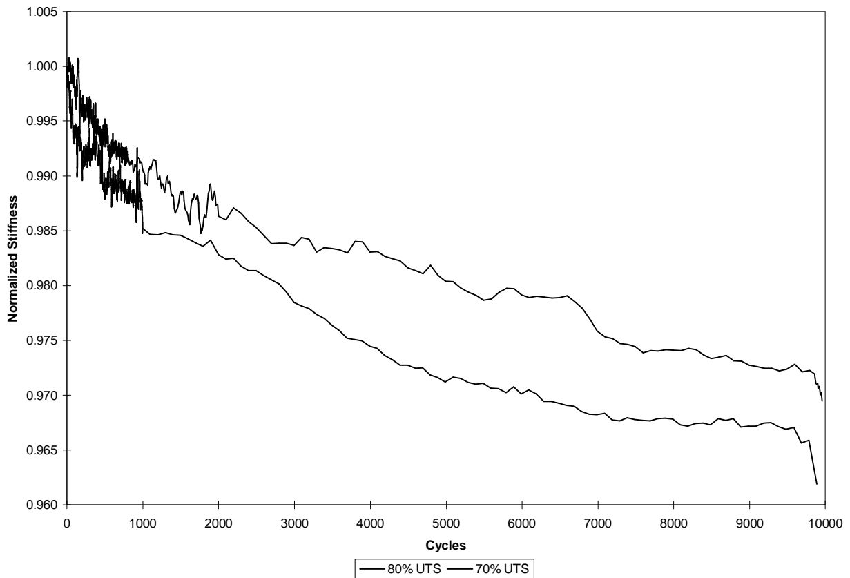
Figure 5.13. Fatigue stiffness reduction curves based on stroke measurements at 350°F (177°C) for [0/\pm 45]_{2s} IM7/K3B laminates containing a center hole.
