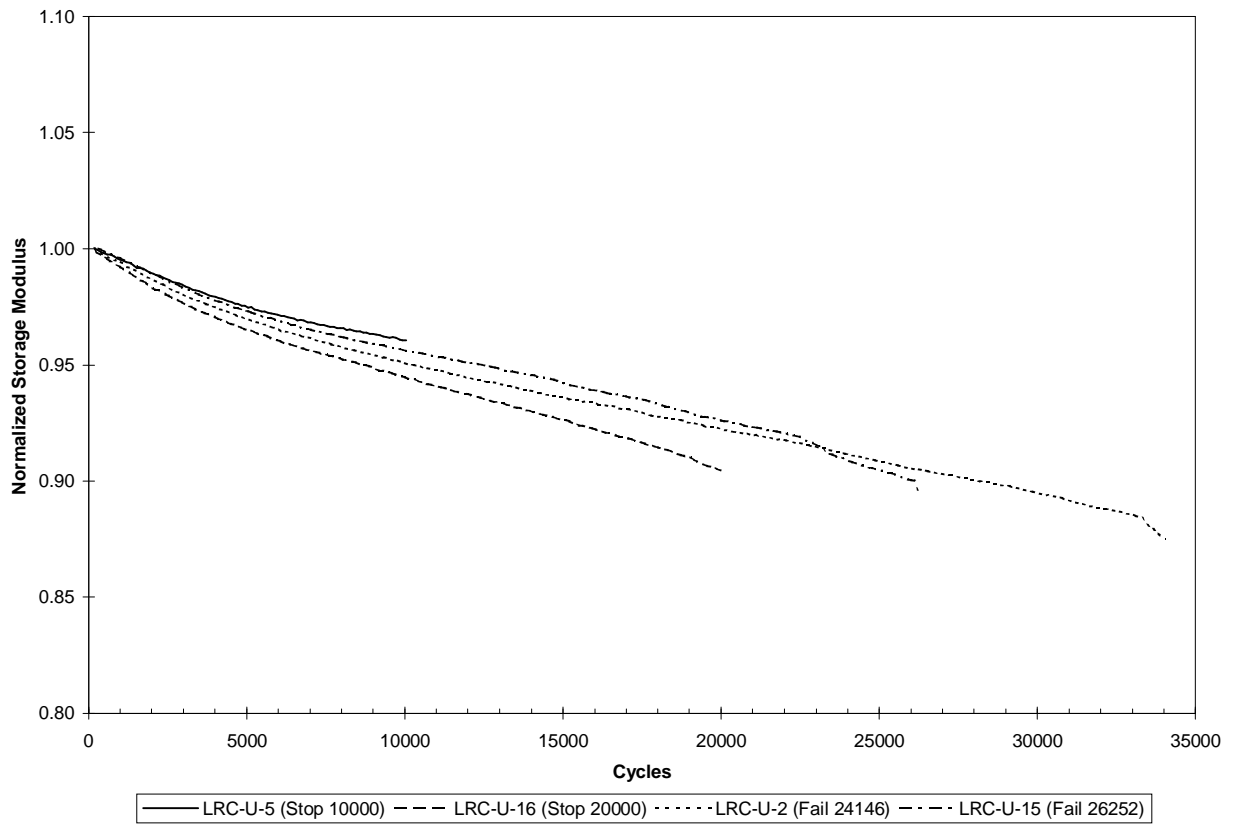
Figure 5.35. Normalized dynamic storage modulus measurements for room temperature fatigue tests at 65% of ultimate strength for [45/0/-45/90]_{2s} IM7/K3B laminates without a center hole.
