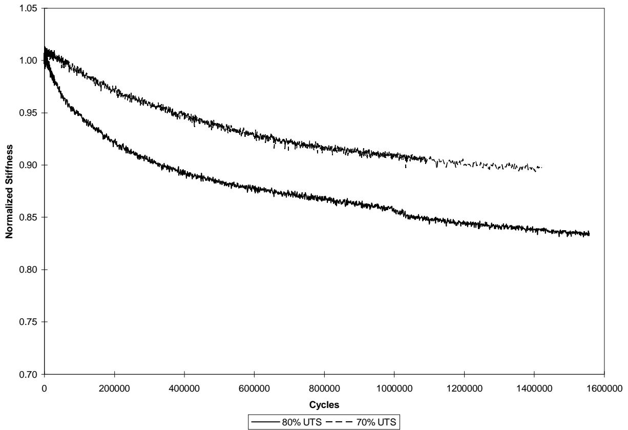
Figure 5.12. Fatigue stiffness reduction curves based on stroke measurements at room temperature for [0/\pm 45]_{2s} IM7/K3B laminates containing a center hole.
