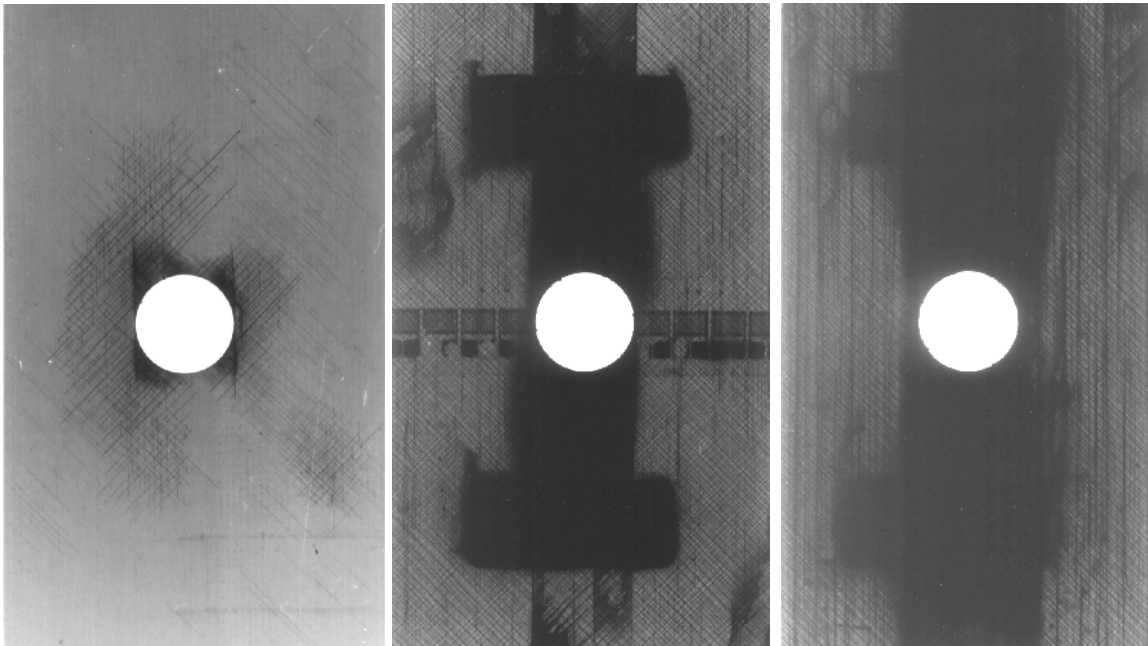
Figure 5.15. Penetrant-enhanced radiographs of [0/\pm 45]_{2s} laminates of IM7/K3B fatigued at room temperature at 80% of ultimate tensile strength after 10000 cycles (left), 280000 cycles (center) and 1560401 cycles (right).
