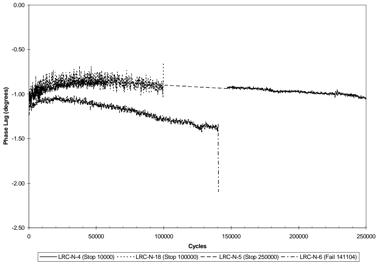
Figure 5.48. Phase lag measurements for 350°F (177°C) fatigue tests at 70% of ultimate strength for [45/0/-45/90]_{2s} IM7/K3B laminates with a center hole.
