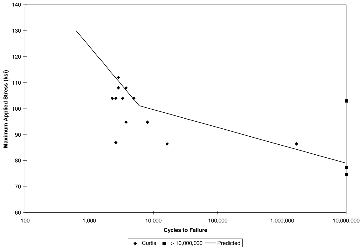
Figure 3.6. Comparison between predicted and measured fatigue lives for cross-ply APC-2 based on the data of Curtis [55].
