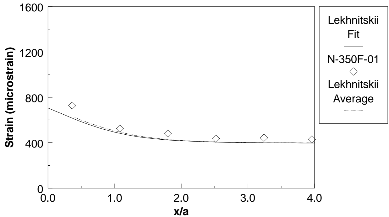
Figure 5.25. Comparison between the strip-strain gage measurements and the predictions based on the effective hole size for a specimen fatigued 10000 cycles at 350°F (177°C) at 80% of ultimate strength.
