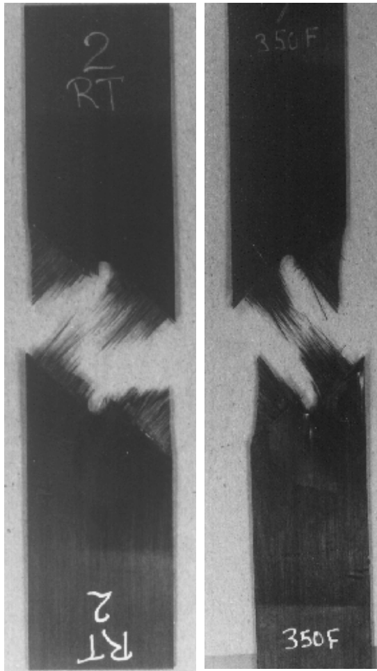
Figure 5.8. Failed notched [0/\pm 45]_{2s} tensile specimens from room temperature (left) and 350°F (177°C) (right) tests.
