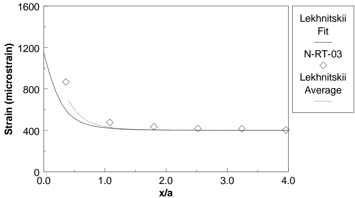
Figure 5.19. Comparison between the strip-strain gage measurements and the predictions based on the effective hole size for a specimen fatigued 10000 cycles at room temperature at 70% of ultimate strength.
