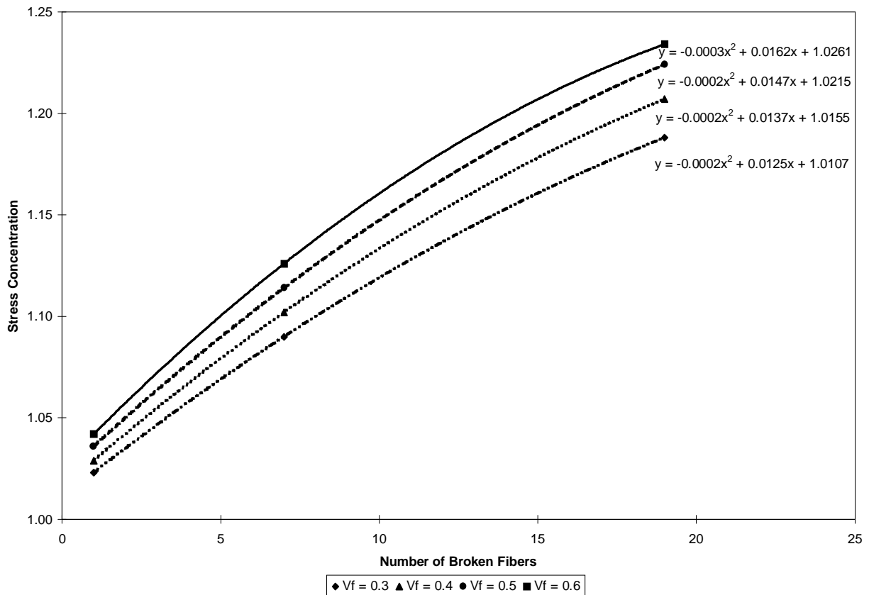
Figure 2.13. Center stress concentration as a function of fiber volume fraction and number of broken fibers.
