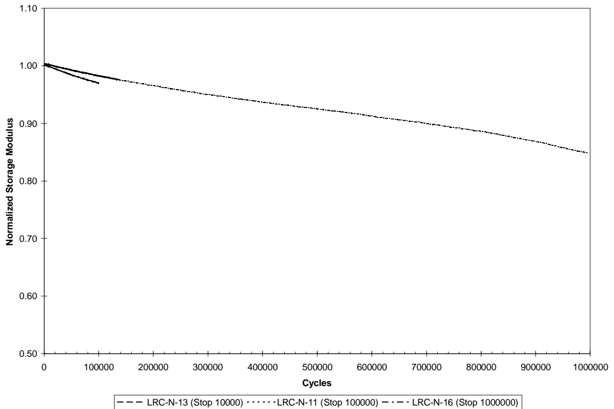
Figure 5.43. Normalized dynamic storage modulus measurements for room temperature fatigue tests at 70% of ultimate strength for [45/0/-45/90]_{2s} IM7/K3B laminates with a center hole.
