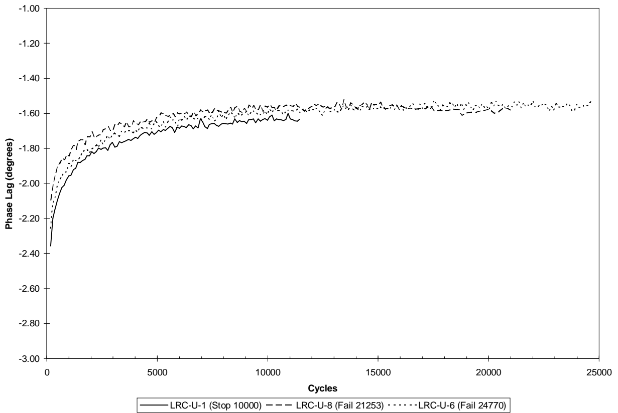
Figure 5.38. Phase lag measurements for room temperature fatigue tests at 70% of ultimate strength for [45/0/-45/90]_{2s} IM7/K3B laminates without a center hole.
