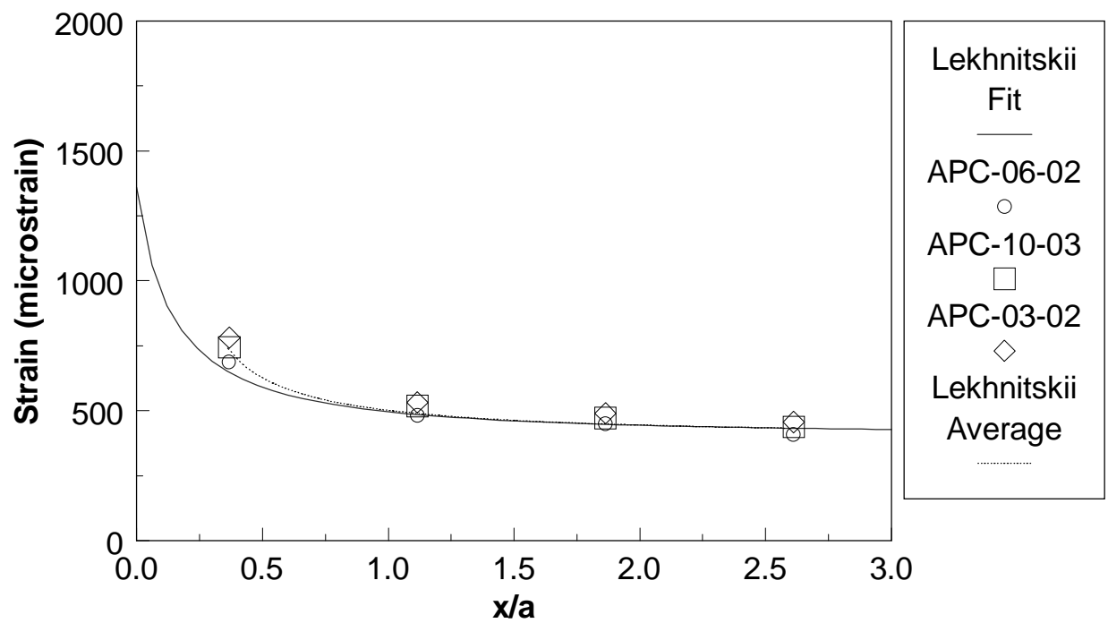
Figure 4.10. Comparison between the strip-strain gage measurements and the predictions based on the effective hole size for specimens fatigued 10000 cycles at 80% of the ultimate strength.
