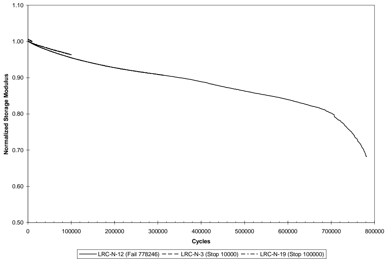
Figure 5.45. Normalized dynamic storage modulus measurements for room temperature fatigue tests at 80% of ultimate strength for [45/0/-45/90]_{2s} IM7/K3B laminates with a center hole.
