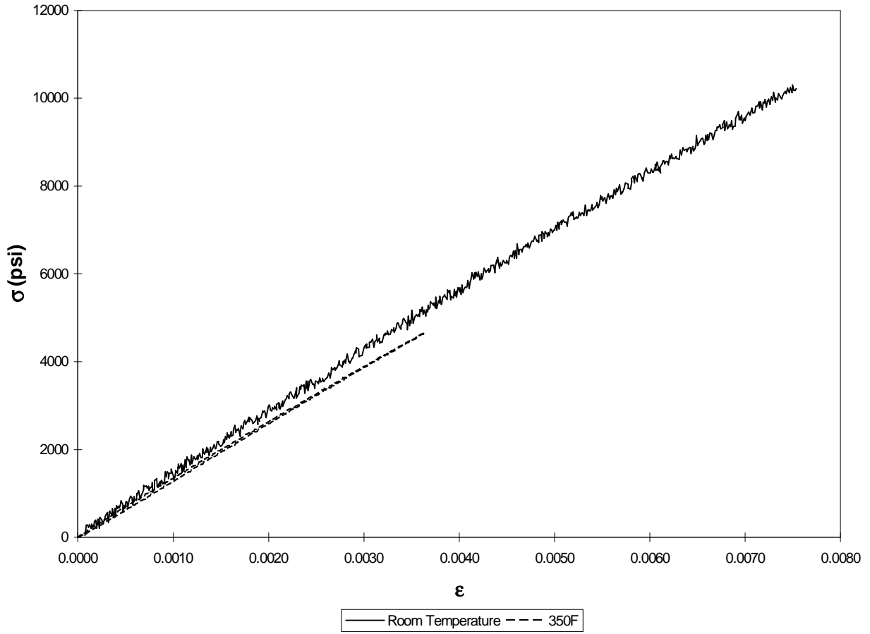
Figure 5.5. Stress-strain curves for [90]_{12} laminates of IM7/K3B at room temperature and 350°F (177°C).
