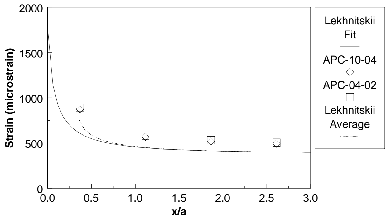
Figure 4.12. Comparison between the strip-strain gage measurements and the predictions based on the effective hole size for specimens fatigued 100 cycles at 87.5% of the ultimate strength.
