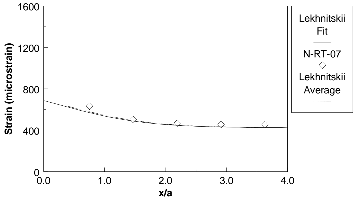
Figure 5.22. Comparison between the strip-strain gage measurements and the predictions based on the effective hole size for a specimen fatigued 280000 cycles at room temperature at 80% of ultimate strength.
