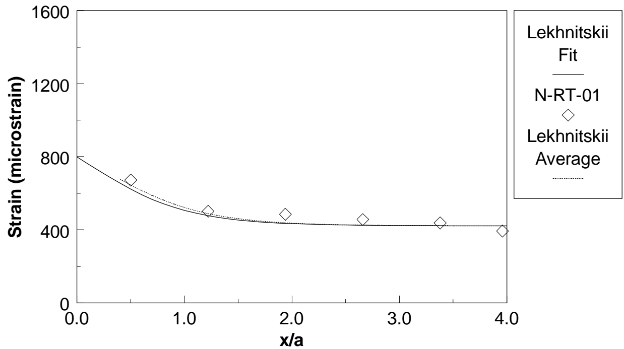
Figure 5.20. Comparison between the strip-strain gage measurements and the predictions based on the effective hole size for a specimen fatigued 260000 cycles at room temperature at 70% of ultimate strength.
