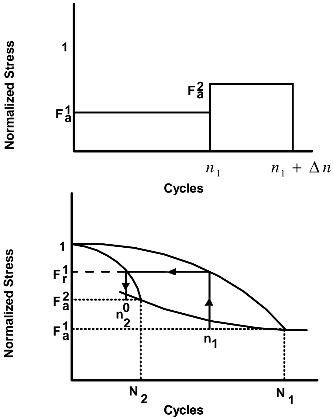
Figure 3.2. Calculation of equivalent ("pseudo") cycles for block loading.
