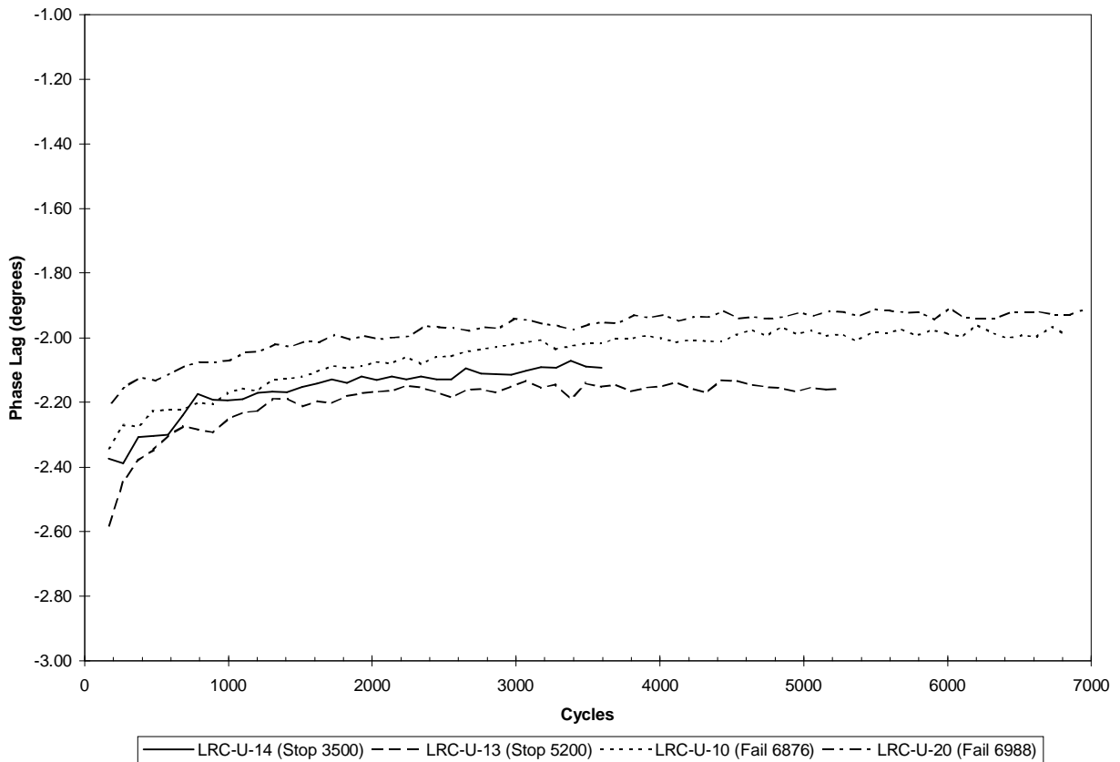
Figure 5.42. Phase lag measurements for 350°F (177°C) fatigue tests at 70% of ultimate strength for [45/0/-45/90]_{2s} IM7/K3B laminates without a center hole.
