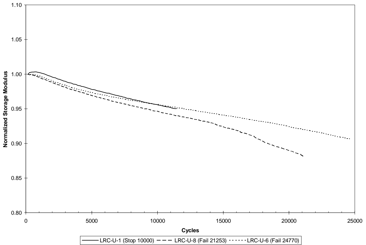
Figure 5.37. Normalized dynamic storage modulus measurements for room temperature fatigue tests at 70% of ultimate strength for [45/0/-45/90]_{2s} IM7/K3B laminates without a center hole.
