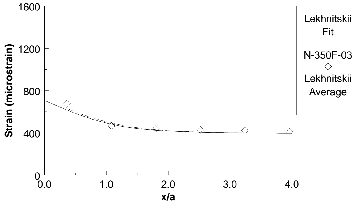
Figure 5.23. Comparison between the strip-strain gage measurements and the predictions based on the effective hole size for a specimen fatigued 10000 cycles at 350°F (177°C) at 70% of ultimate strength.
