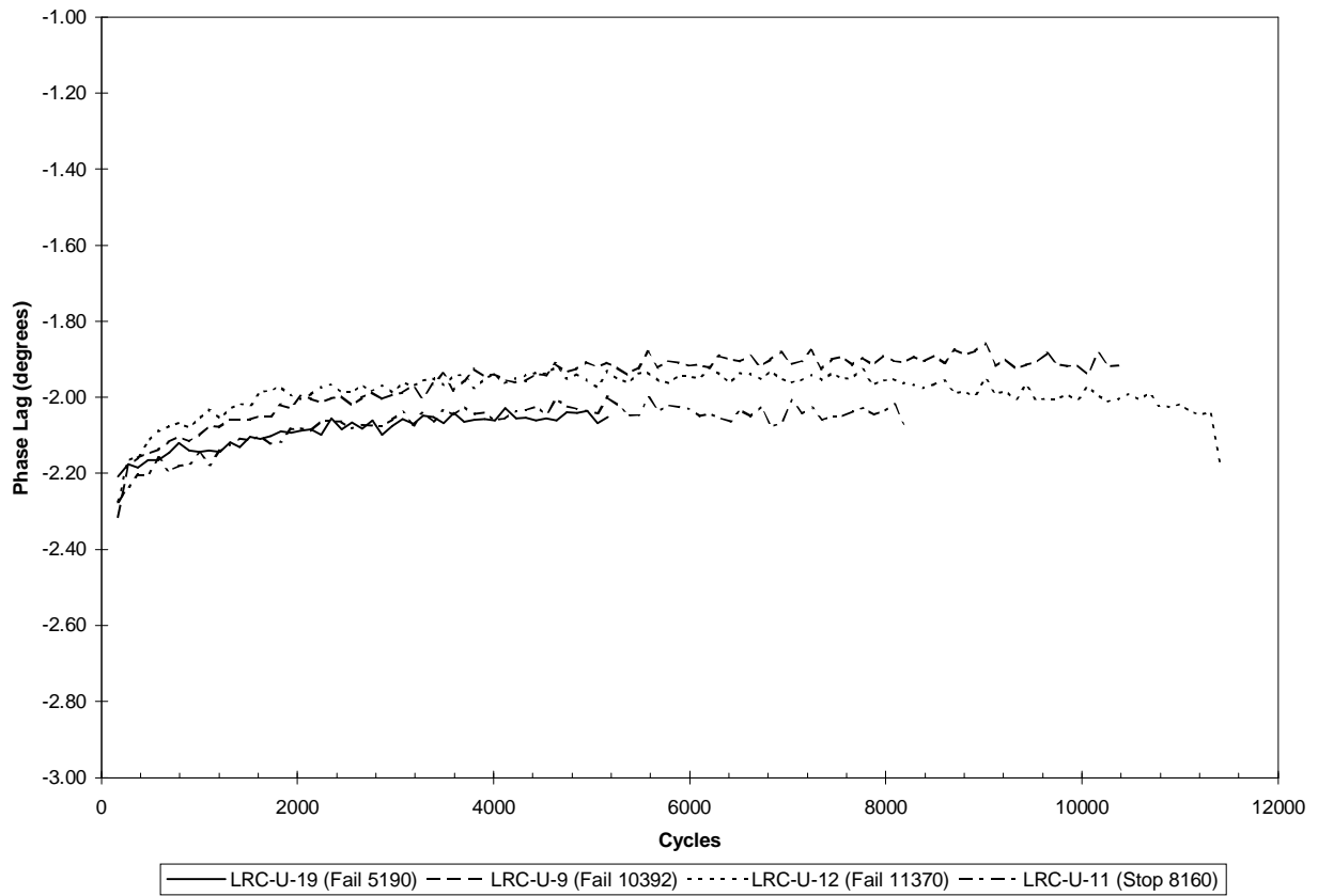
Figure 5.40. Phase lag measurements for room temperature fatigue tests at 65% of ultimate strength for [45/0/-45/90]_{2s} IM7/K3B laminates without a center hole.
