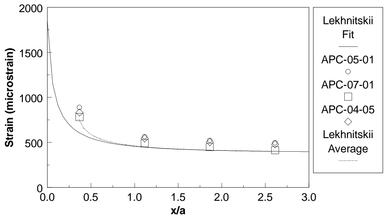
Figure 4.9. Comparison between the strip-strain gage measurements and the predictions based on the effective hole size for specimens fatigued 100 cycles at 80% of the ultimate strength.
