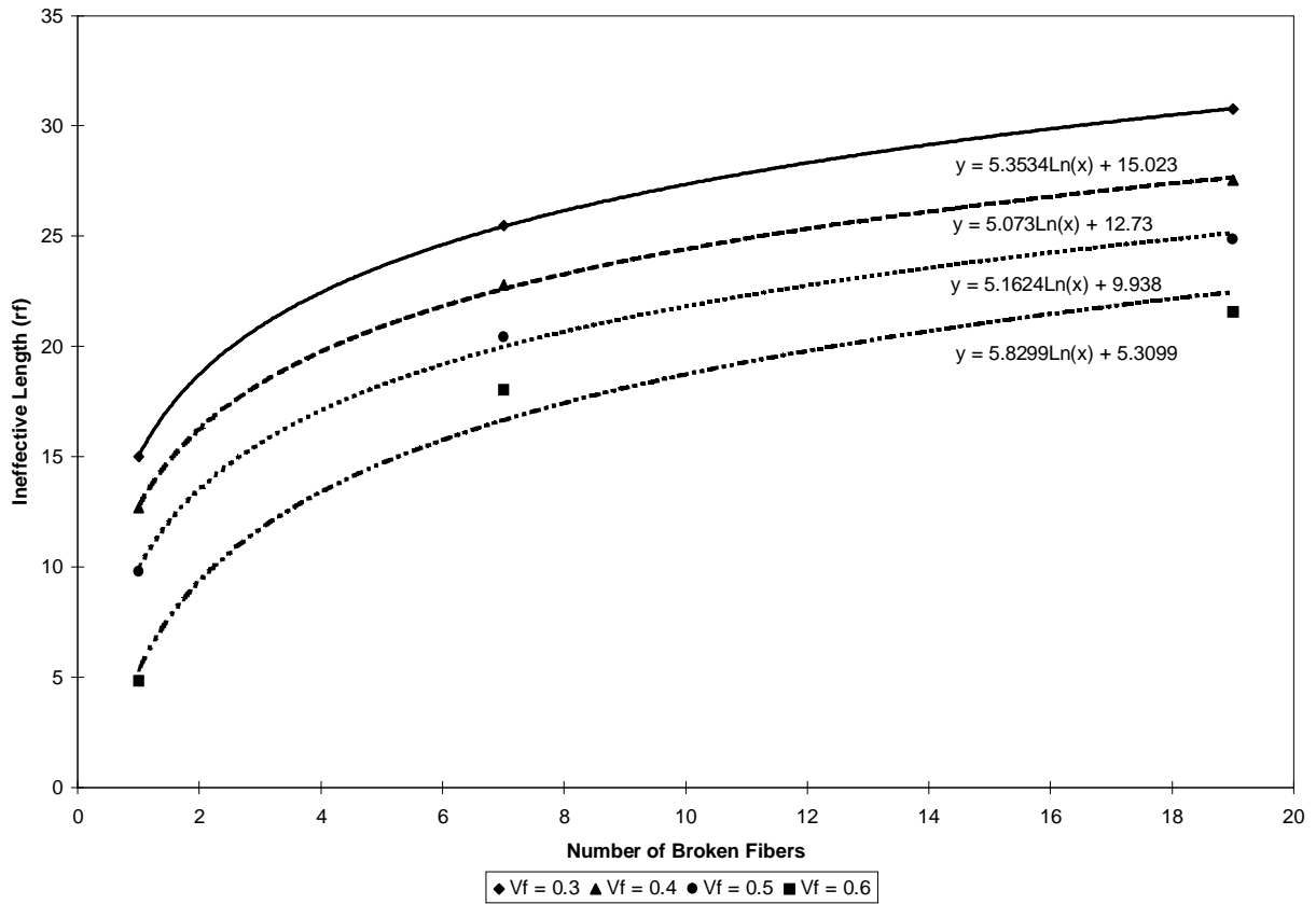
Figure 2.14. Ineffective lengths for glass/epoxy composites of different fiber volume fractions as a function of number of adjacent broken fibers.
