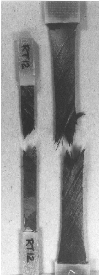
Figure 5.6. Failed [\pm 45]_{3s} tensile specimens from room temperature (left) and 350°F (177°C) tests (right).
