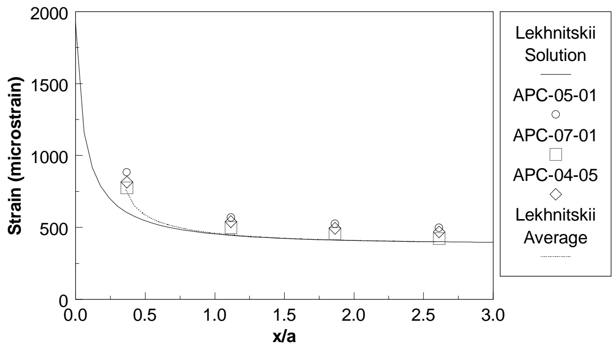
Figure 4.8. Comparison of predicted and measured axial strain as a function of position along the hole axis.
