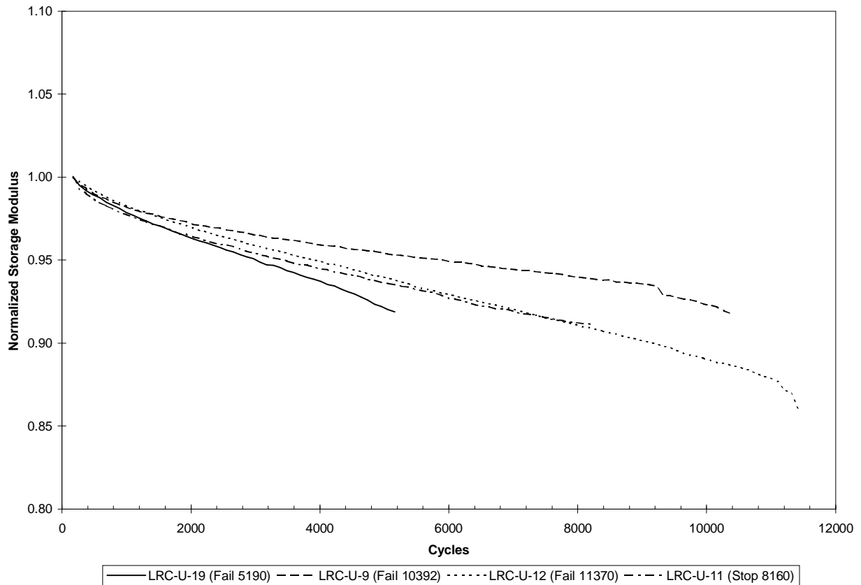
Figure 5.39. Normalized dynamic storage modulus measurements for 350°F (177°C) fatigue tests at 65% of ultimate strength for [45/0/-45/90]_{2s} IM7/K3B laminates without a center hole.
