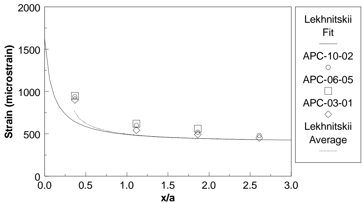
Figure 4.11. Comparison between the strip-strain gage measurements and the predictions based on the effective hole size for specimens fatigued 100000 cycles at 80% of the ultimate strength.
