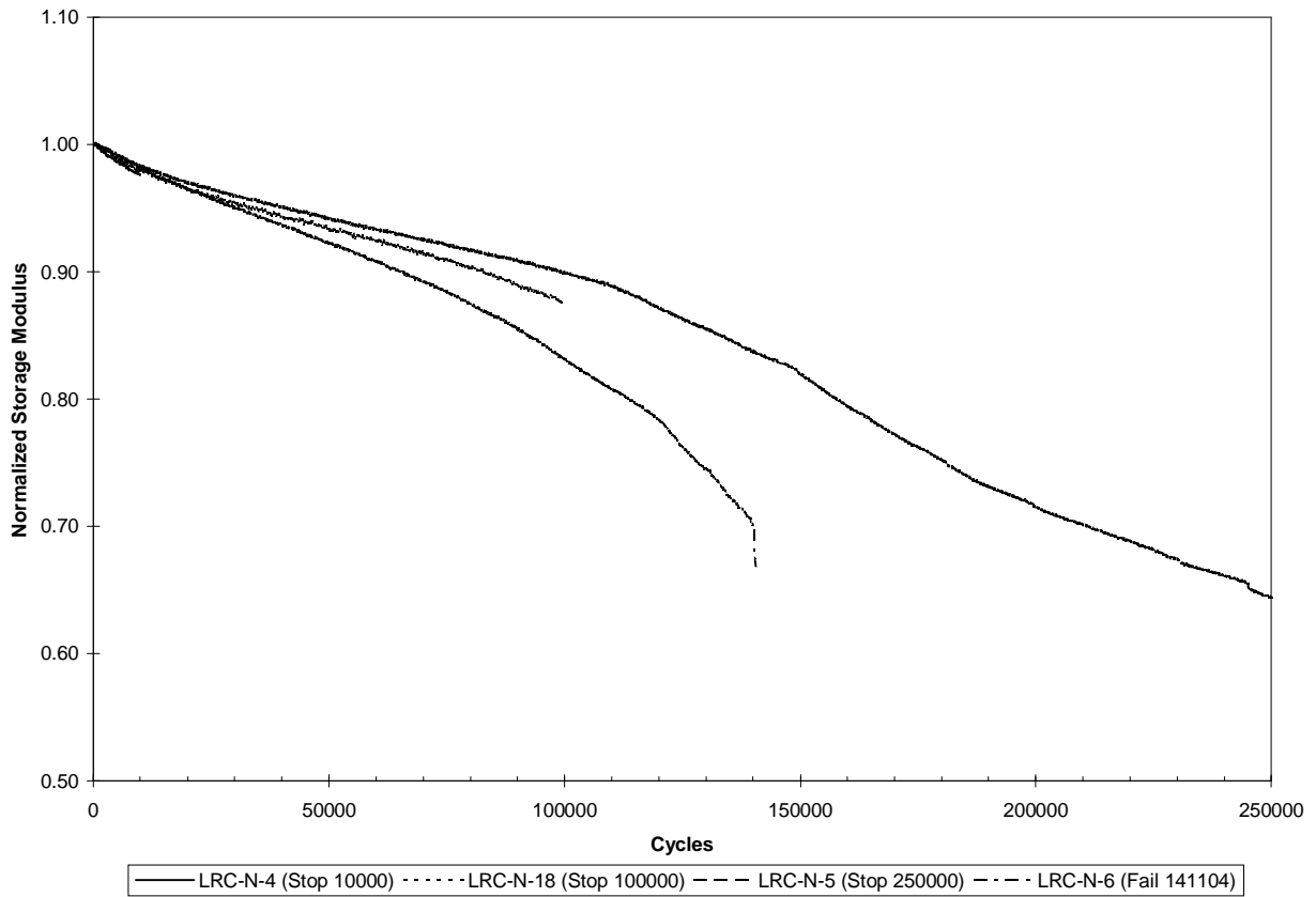
Figure 5.47. Normalized dynamic storage modulus measurements for 350°F (177°C) fatigue tests at 70% of ultimate strength for [45/0/-45/90]_{2s} IM7/K3B laminates with a center hole.
