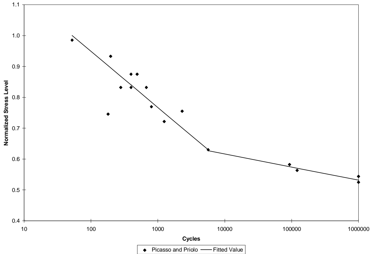
Figure 3.5. Comparison between measured and fitted fatigue lives for unidirectional APC-2 based on the data of Picasso and Priolo [54].
