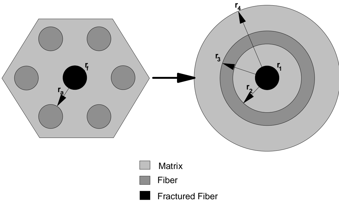
Figure 2.3. Representation of the hexagonal arrangement as an axisymmetric one having the same fiber volume fraction.
