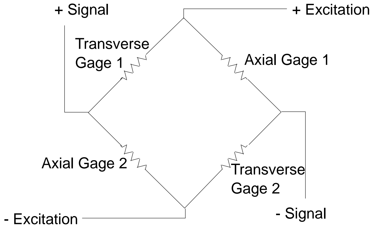
Figure 5.1. Bridge wiring for +/- 45 tensile specimens.
