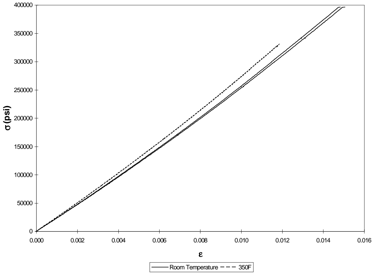
Figure 5.3. Stress-strain curves for [0]_{12} laminates of IM7/K3B at room temperature and 350°F (177°C).
