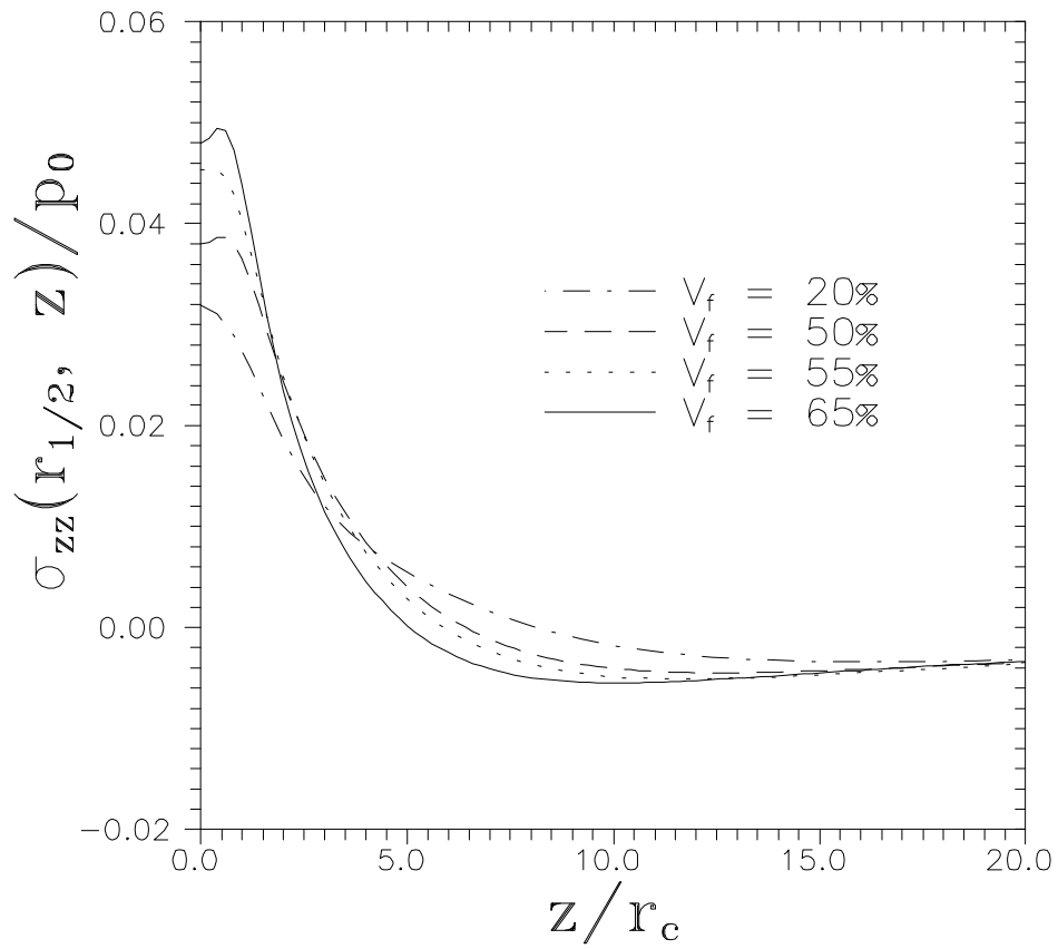
Figure 2.8. Variation of the \sigma_z(r_{1/2}, z)/p_0 stress (at the center of the fiber annular ring) as a function of distance above the crack plane for various fiber volume fractions.
