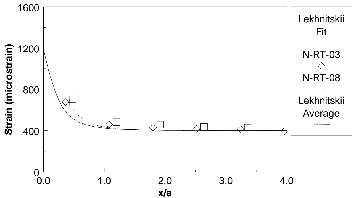
Figure 5.18. Comparison of predicted and measured axial strain as a function of position along the hole axis before fatigue.
