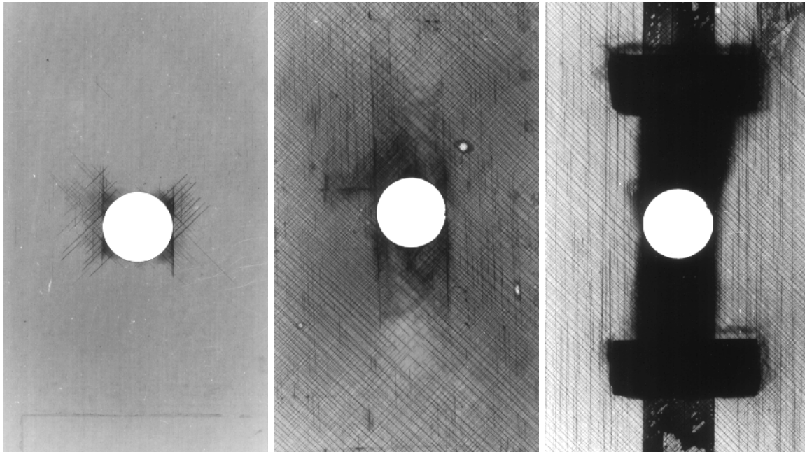
Figure 5.14. Penetrant-enhanced radiographs of [0/\pm 45]_{2s} laminates of IM7/K3B fatigued at room temperature at 70% of ultimate tensile strength after 10000 cycles (left), 260000 cycles (center) and 1430515 cycles (right).
