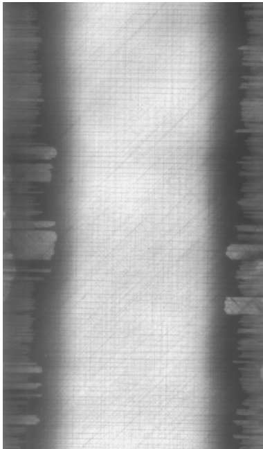
Figure 5.53. Penetrant-enhanced radiograph of an unnotched [45/0/-45/90]_{2s} laminate of IM7/K3B fatigued at 350°F (177°C) at 65% of ultimate tensile strength after 8160 cycles.
