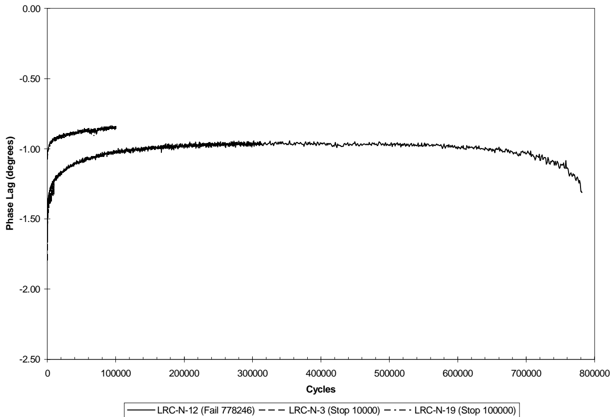
Figure 5.46. Phase lag measurements for room temperature fatigue tests at 80% of ultimate strength for [45/0/-45/90]_{2s} IM7/K3B laminates with a center hole.
