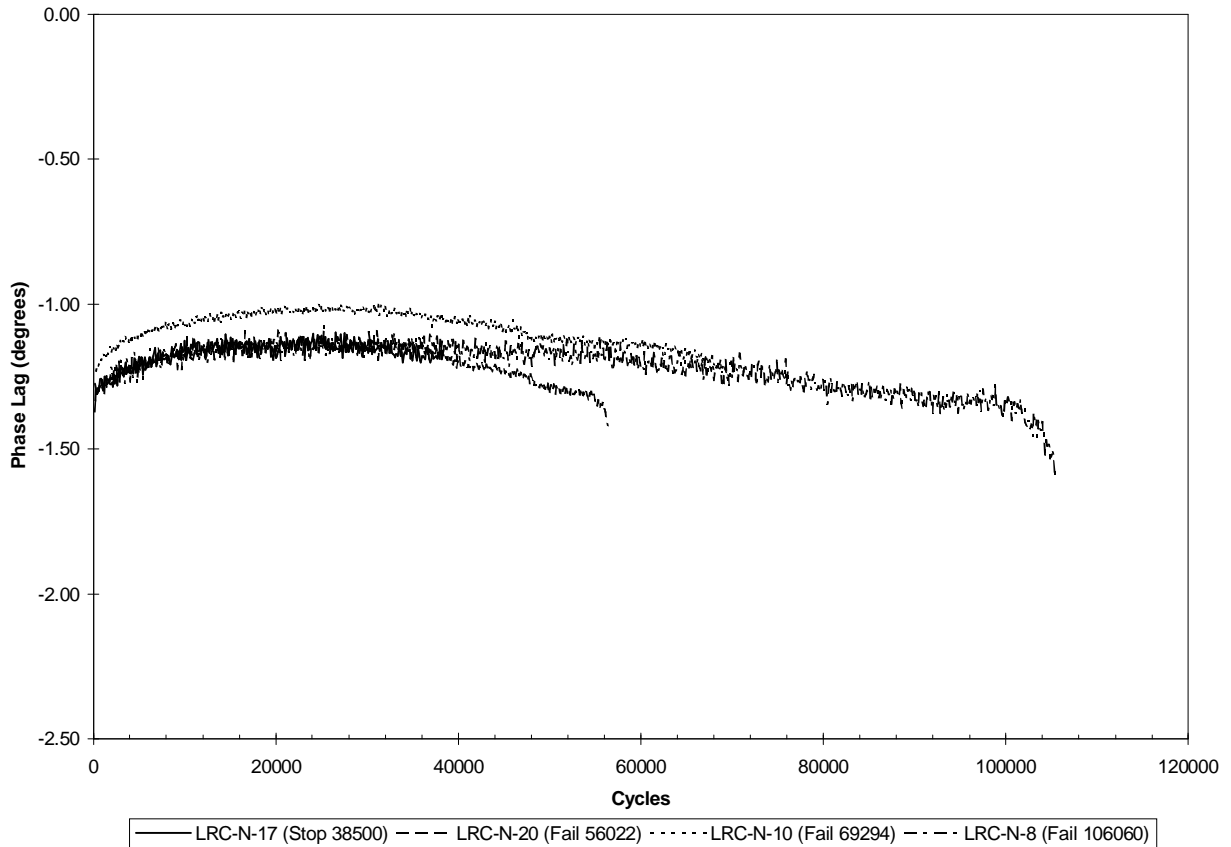
Figure 5.50. Phase lag measurements for 350°F (177°C) fatigue tests at 70% of ultimate strength for [45/0/-45/90]_{2s} IM7/K3B laminates with a center hole.
