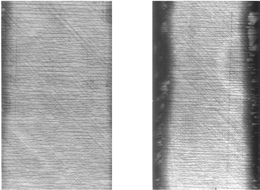
Figure 5.51. Penetrant-enhanced radiographs of unnotched [45/0/-45/90]_{2s} laminates of IM7/K3B fatigued at room temperature at 65% of ultimate tensile strength after 10000 cycles (left) and 20000 cycles (right).
