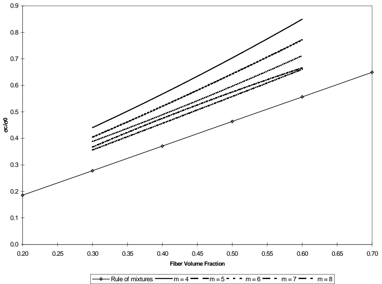
Figure 2.15. Predicted composite strengths as a function of fiber volume fraction and Weibull modulus using the maximum stress concentration values.
