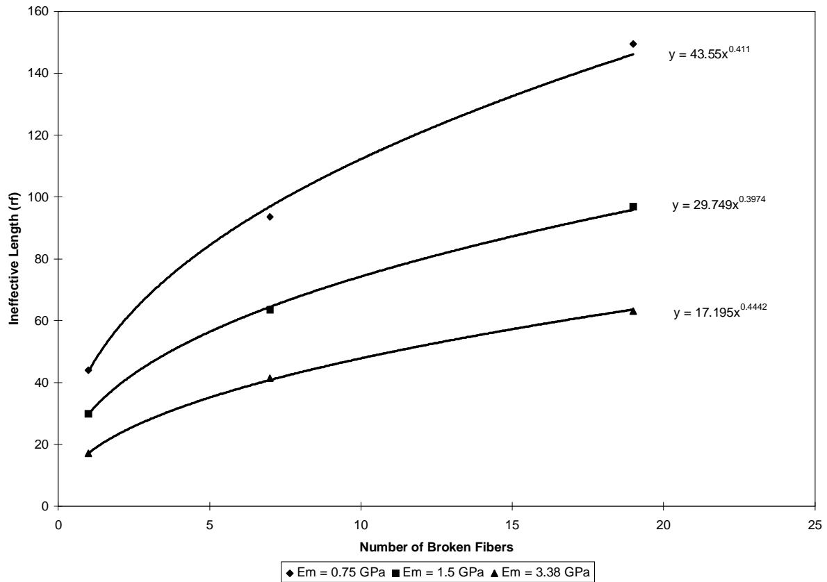
Figure 2.21. Ineffective length as a function of number of broken fibers and matrix stiffness for a graphite/polymeric composite material.
