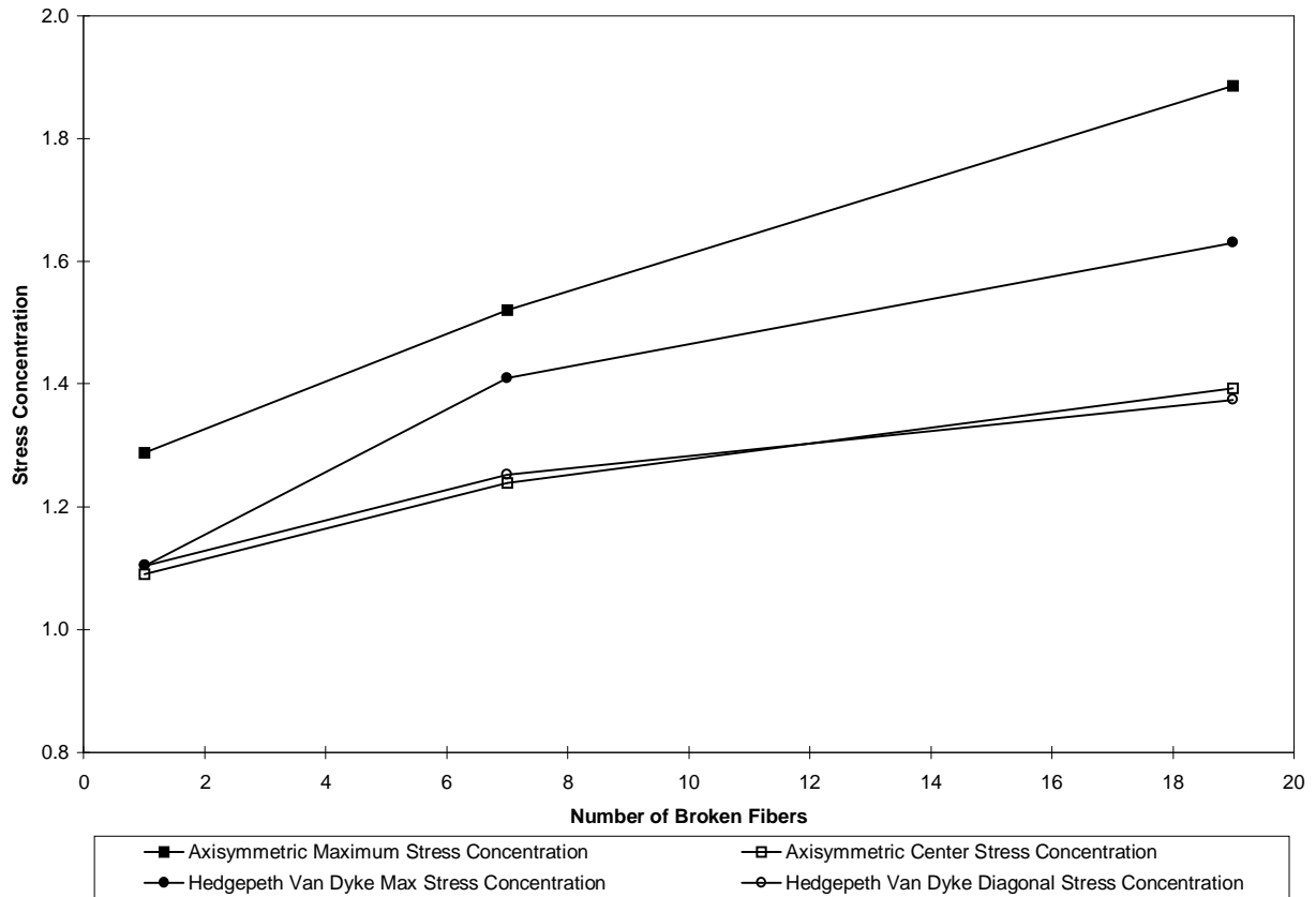
Figure 2.18. Comparison between the predicted stress concentrations using the axisymmetric model [26] and the analysis of Hedgepeth and Van Dyke [20].
