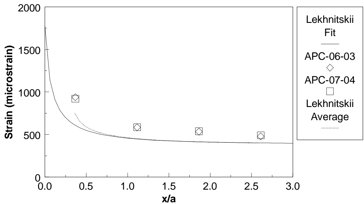
Figure 4.13. Comparison between the strip-strain gage measurements and the predictions based on the effective hole size for specimens fatigued 10000 cycles at 87.5% of the ultimate strength.
