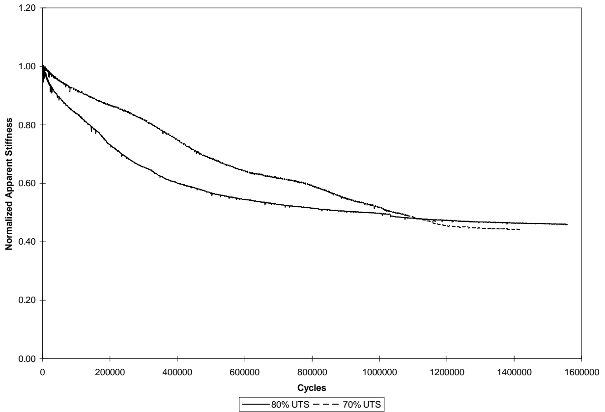
Figure 5.11. Fatigue stiffness reduction curves based on extensometer measurements at room temperature for [0/\pm 45]_{2s} IM7/K3B laminates containing a center hole.
