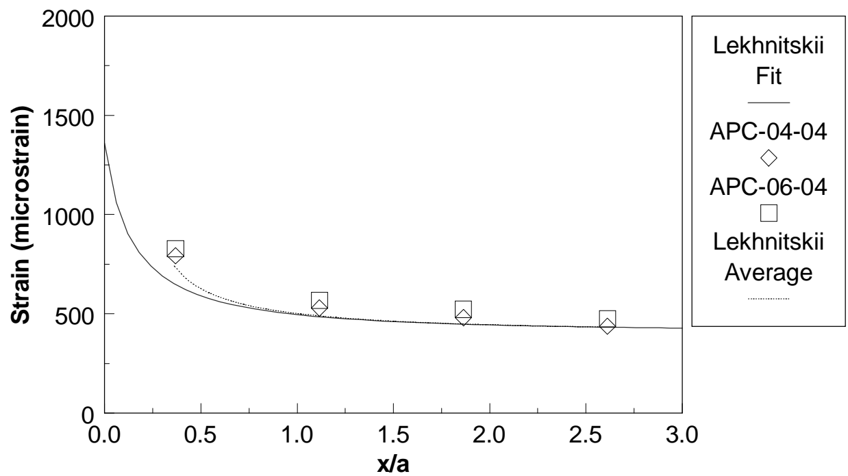
Figure 4.14. Comparison between the strip-strain gage measurements and the predictions based on the effective hole size for specimens fatigued 100000 cycles at 87.5% of the ultimate strength.
