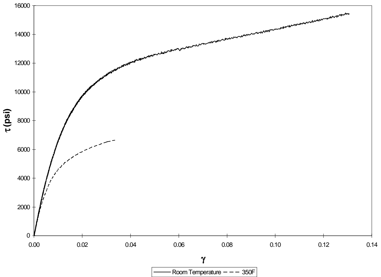
Figure 5.7. Shear stress-shear strain curves for [\pm 45]_{3s} laminates of IM7/K3B at room temperature and 350°F (177°C).
