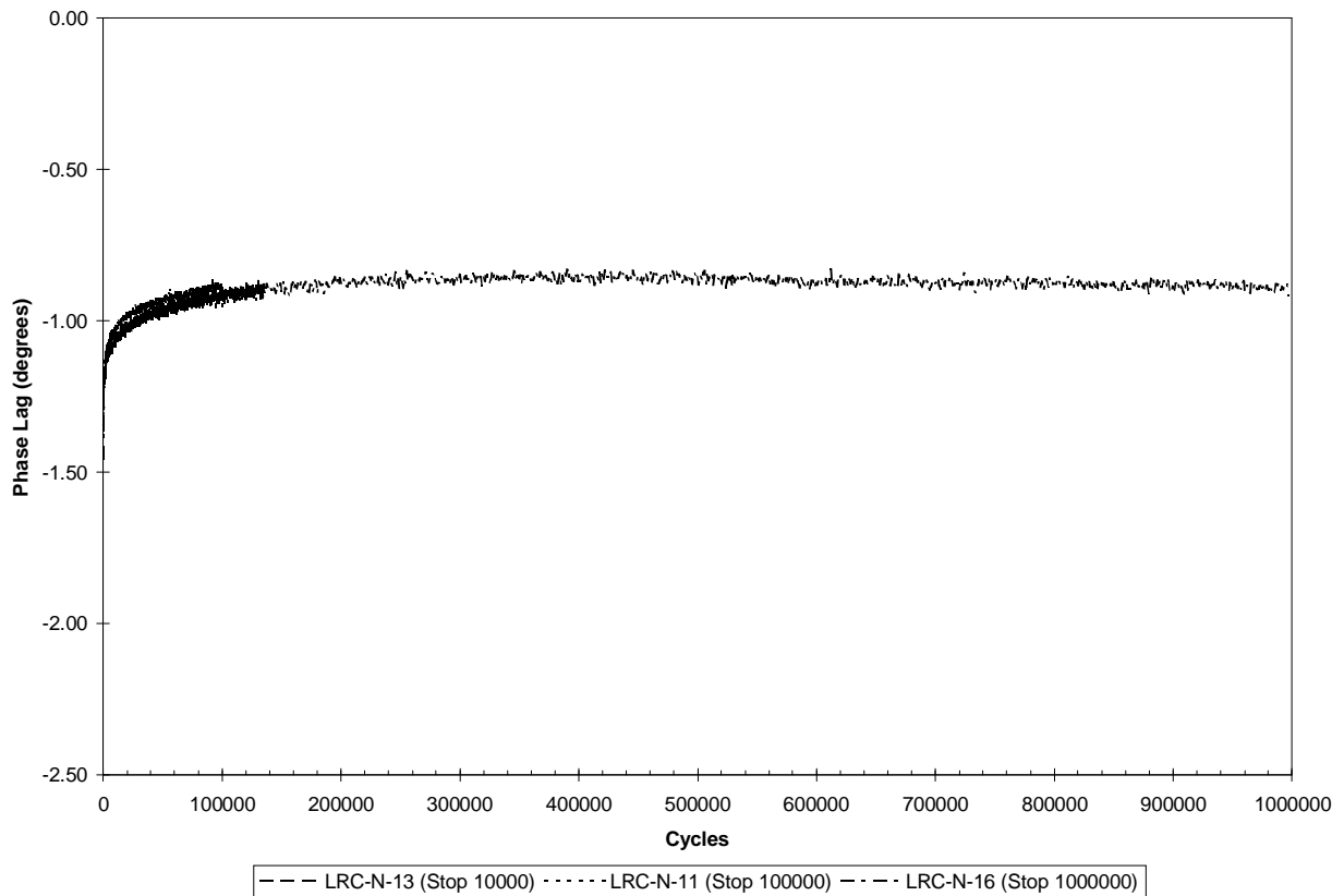
Figure 5.44. Phase lag measurements for room temperature fatigue tests at 70% of ultimate strength for [45/0/-45/90]_{2s} IM7/K3B laminates with a center hole.
