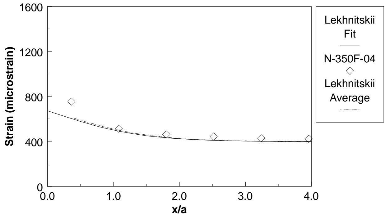
Figure 5.24. Comparison between the strip-strain gage measurements and the predictions based on the effective hole size for a specimen fatigued 10000 cycles at 350°F (177°C) at 80% of ultimate strength.
