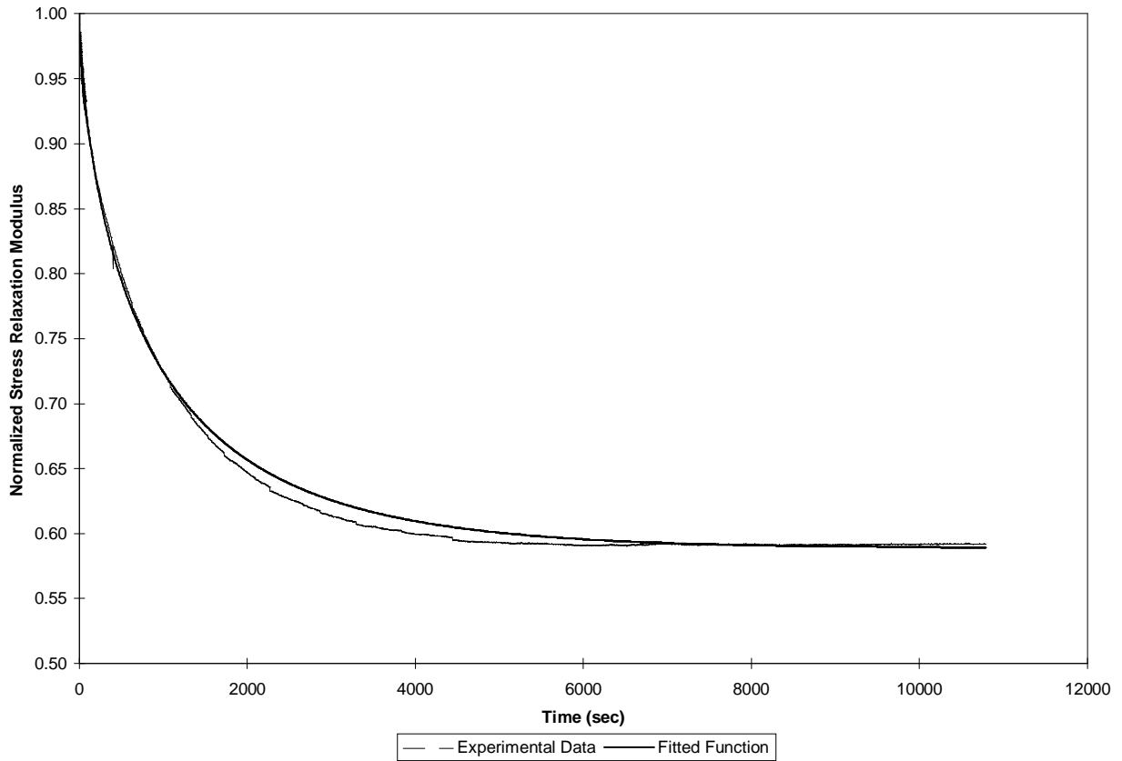
Figure 5.27. Comparison between measured and fitted stress relaxation modulus for [\pm 45]_{3s} IM7/K3B at 350°F (177°C).
