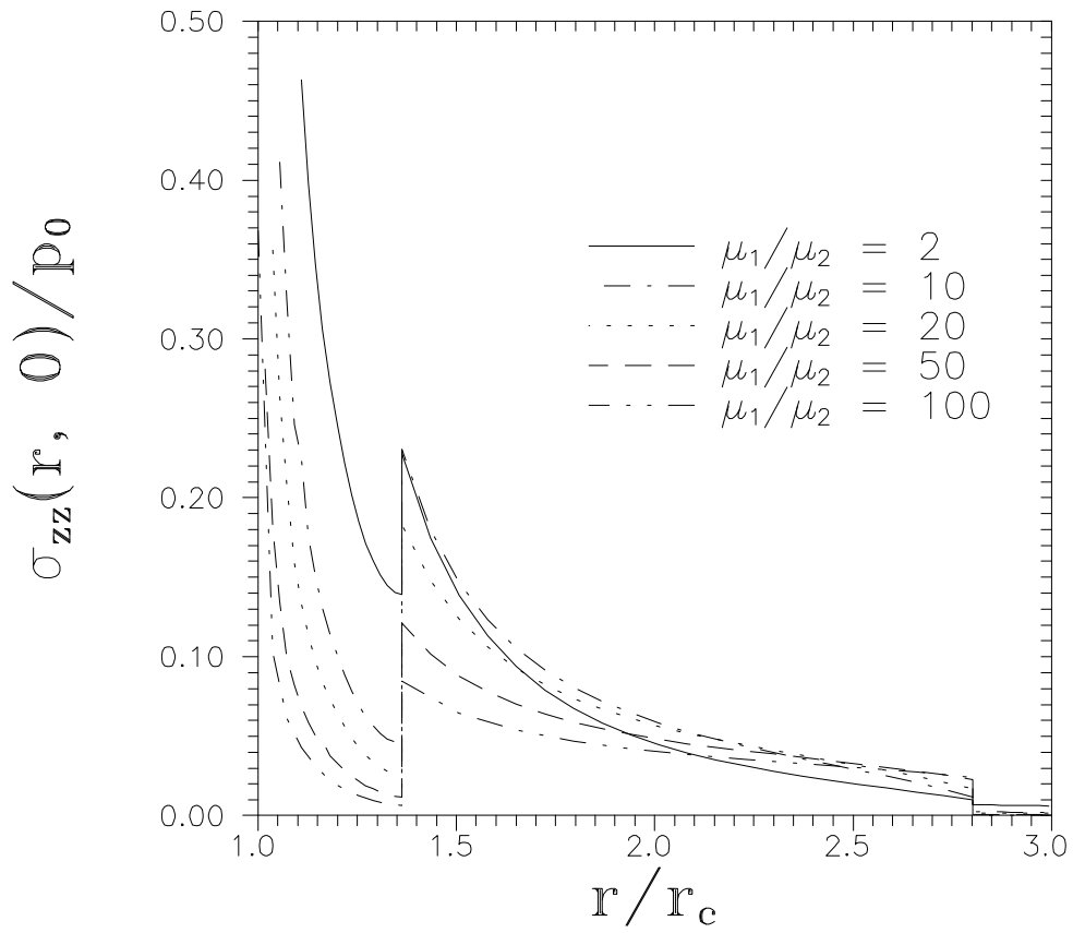
Figure 2.9. Variation of the \sigma_{zz}^{(i)}(r,0) stress (in the plane of the crack) for the three inner concentric cylinders ( i = 2, 3, 4 ).
