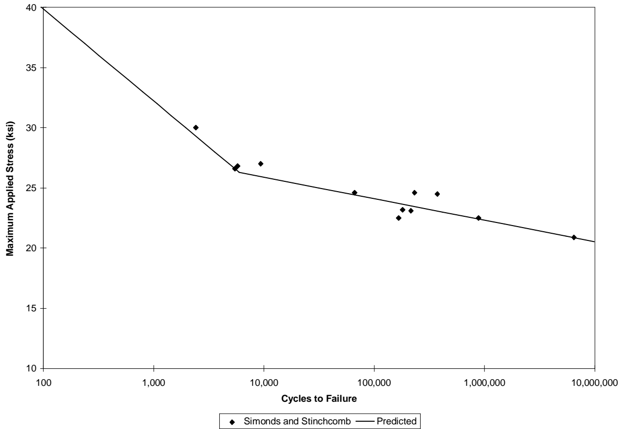
Figure 3.7. Comparison between predicted and measured fatigue lives for quasi-isotropic APC-2 based on the data of Simonds and Stinchcomb [56].
