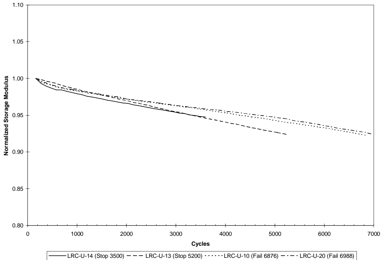
Figure 5.41. Normalized dynamic storage modulus measurements for 350°F (177°C) fatigue tests at 70% of ultimate strength for [45/0/-45/90]_{2s} IM7/K3B laminates without a center hole.
