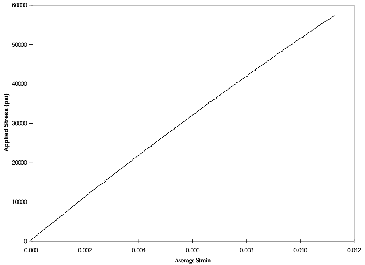
Figure 5.34. Representative stress-strain curve based on stroke measurements for 350°F (177°C) tests of [45/0/-45/90] 2s IM7/K3B laminates with a center hole.
