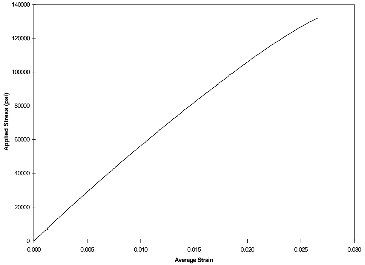
Figure 5.31. Representative stress-strain curve based on stroke measurements for 350°F (177°C) tests of [45/0/-45/90] 2s IM7/K3B laminates without a center hole.
