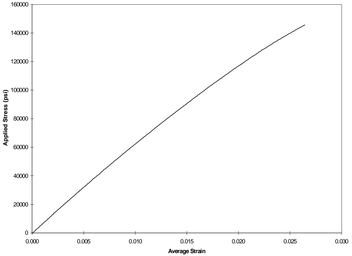
Figure 5.30. Representative stress-strain curve based on stroke measurements for room temperature tests [45/0/-45/90]_{2s} IM7/K3B laminates without a center hole.
