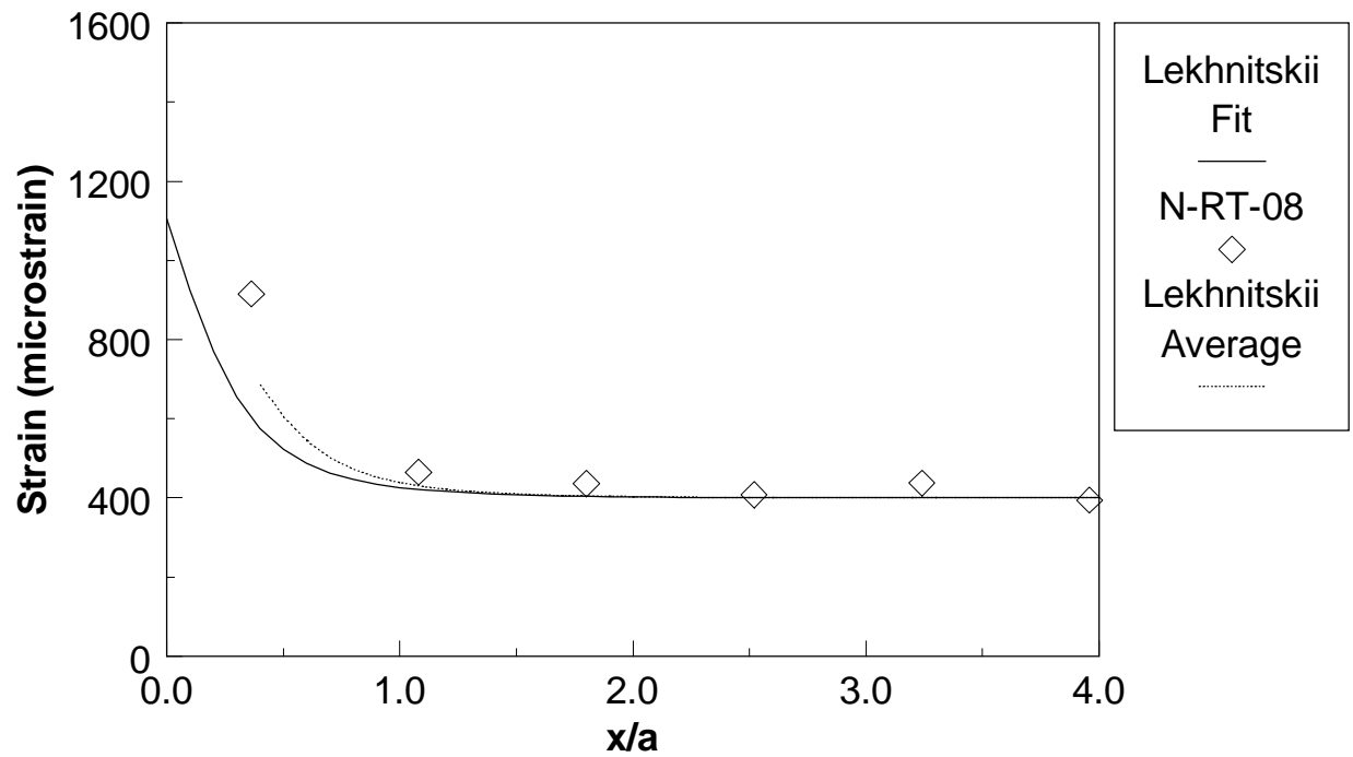
Figure 5.21. Comparison between the strip-strain gage measurements and the predictions based on the effective hole size for a specimen fatigued 10000 cycles at room temperature at 80% of ultimate strength.
