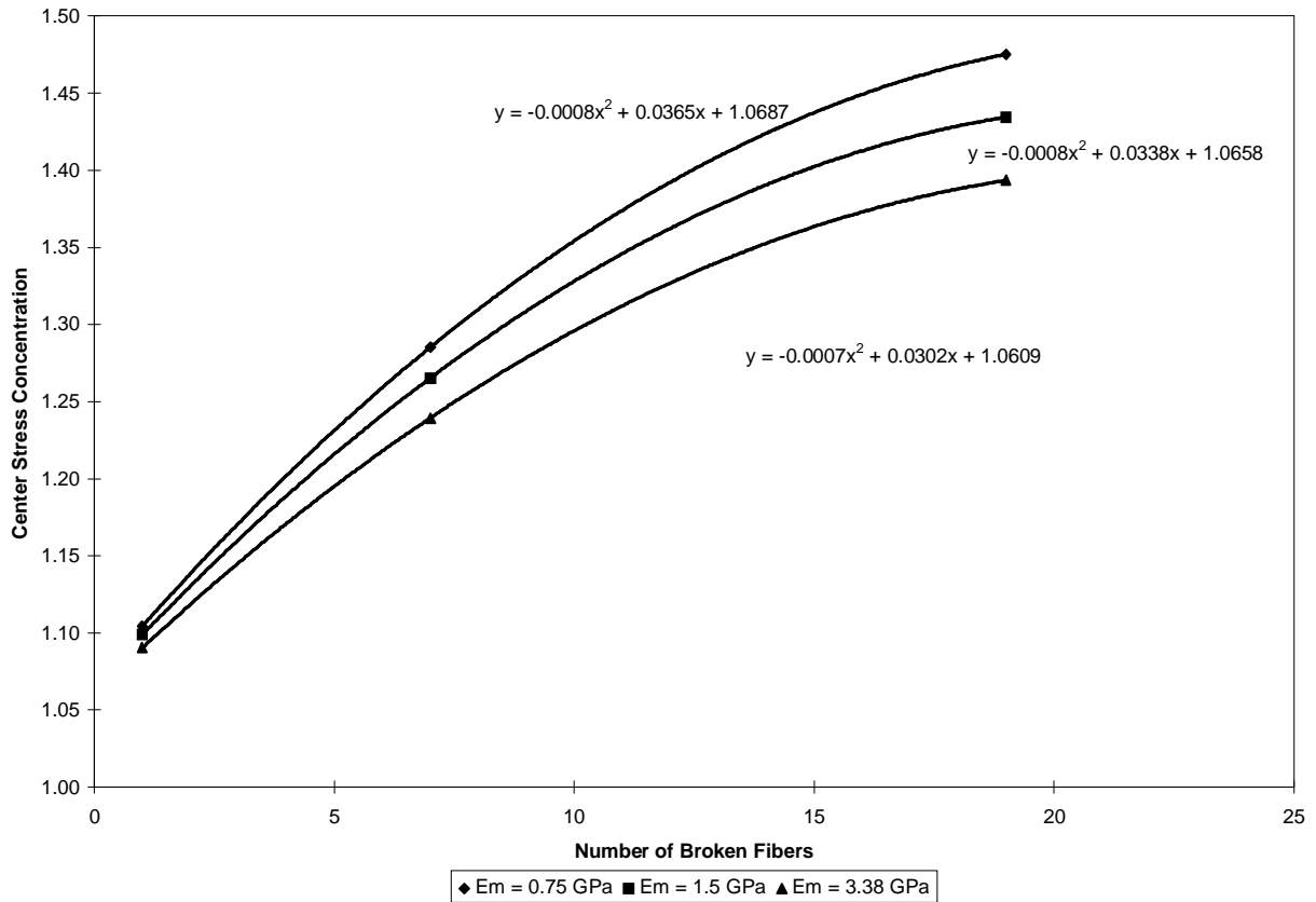
Figure 2.19. Center stress concentration on adjacent fibers as a function of number of broken fibers and matrix stiffness for a graphite/polymeric composite material.
