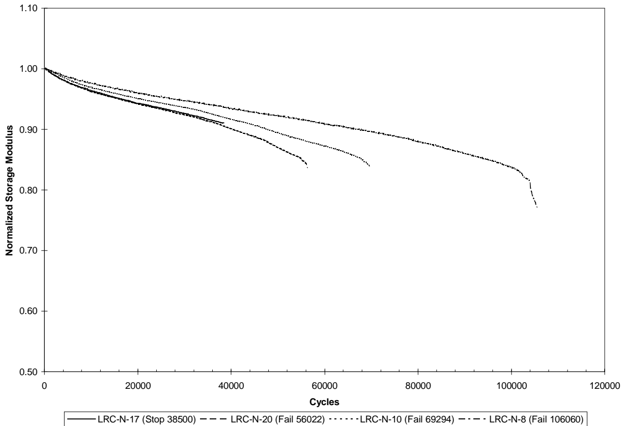
Figure 5.49. Normalized dynamic storage modulus measurements for 350°F (177°C) fatigue tests at 80% of ultimate strength for [45/0/-45/90]_{2s} IM7/K3B laminates with a center hole.
