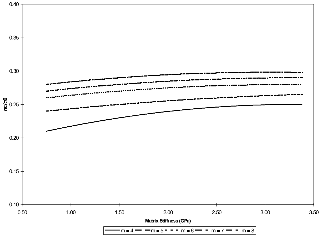
Figure 2.22. Predicted composite strength based on maximum stress concentration as a function of matrix stiffness and fiber Weibull modulus for a 60% fiber volume fraction graphite/polymeric composite material.
