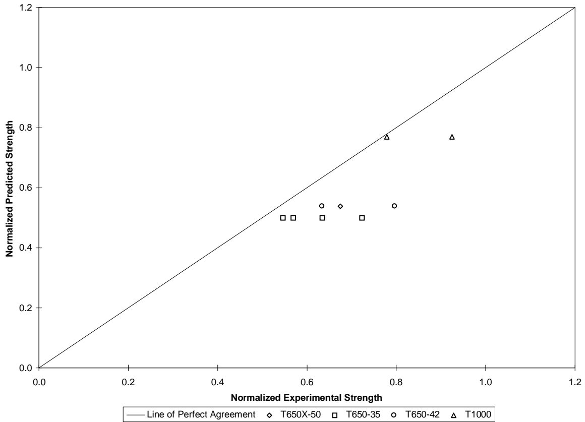
Figure 2.24. Comparison of predicted strength based on maximum stress concentration and experimentally measured values for composites containing four different graphite fibers.
