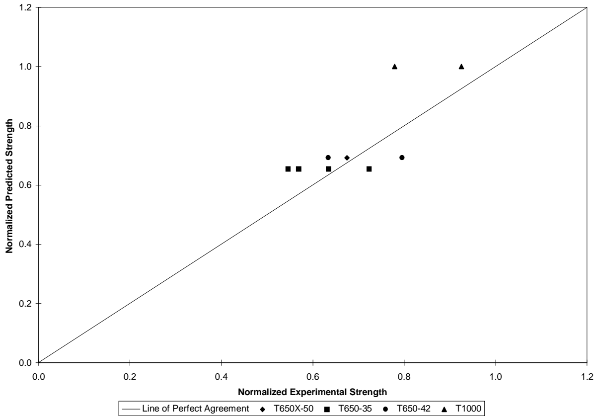
Figure 2.25. Comparison of predicted strength based on center stress concentration and experimentally measured values for composites containing four different graphite fibers.
