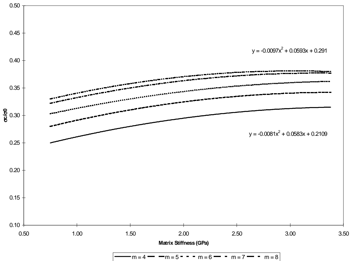
Figure 2.23. Predicted composite strength based on center stress concentration as a function of matrix stiffness and fiber Weibull modulus for a 60% fiber volume fraction graphite/polymeric composite material.
