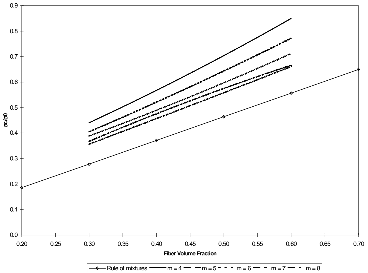
Figure 2.16. Predicted composite strengths as a function of fiber volume fraction and Weibull modulus using the center stress concentration values.
