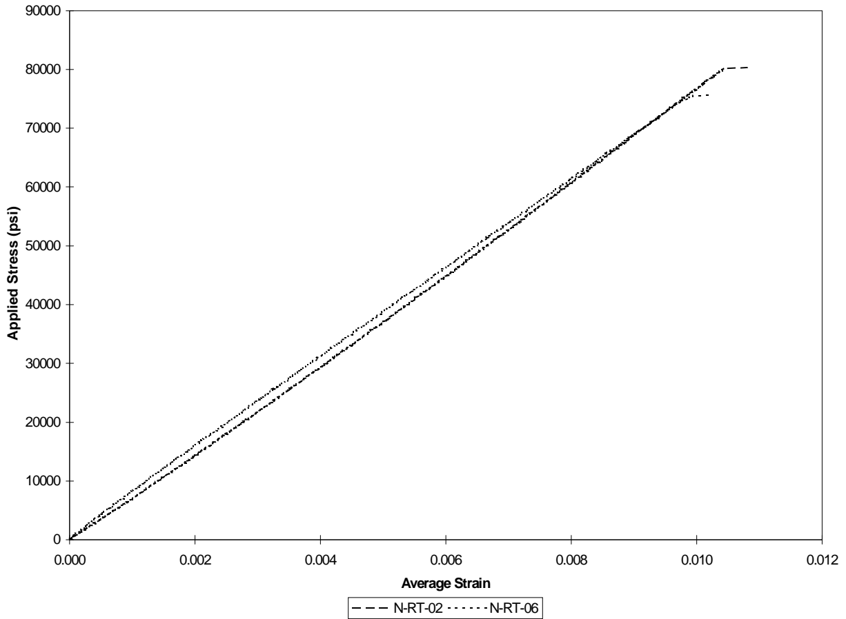
Figure 5.9. Stress-strain curves based on extensometer measurements for room temperature [0/\pm 45]_{2s} IM7/K3B laminates containing a center hole.
