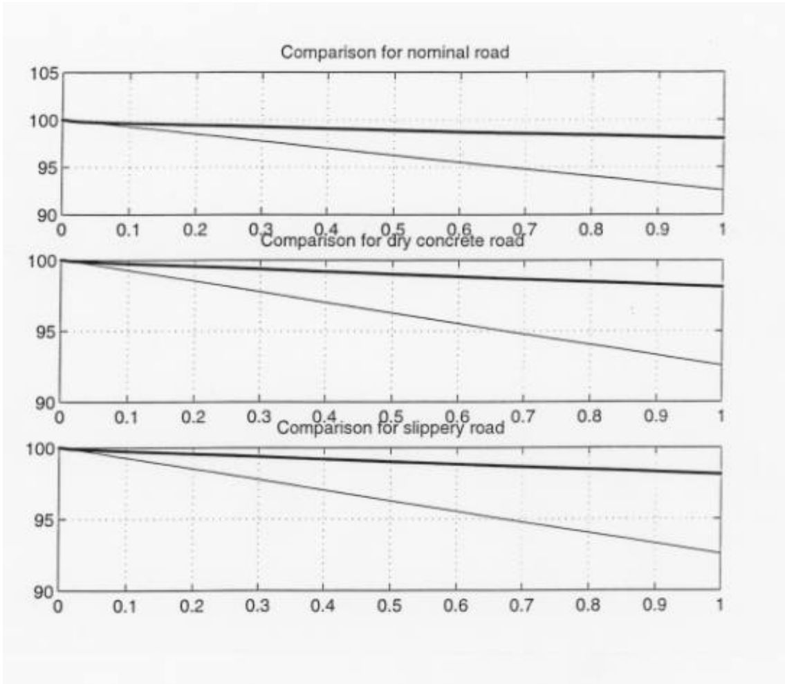
Figure 6.7. Comparison of Simulation Results between Systems with and without Wheel Slip Control
