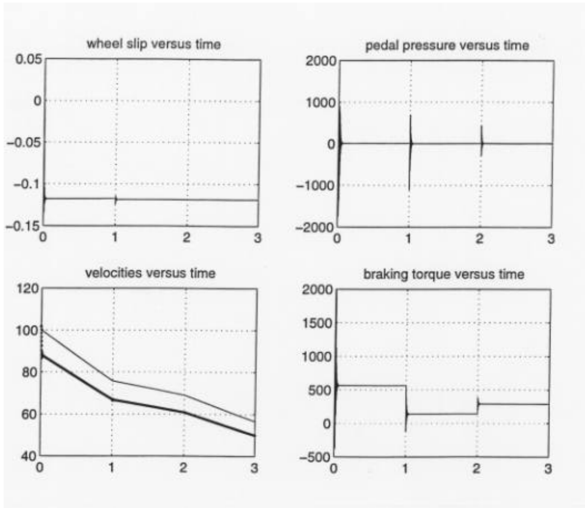
Figure 6.6. Simulation Result on changing road surface
