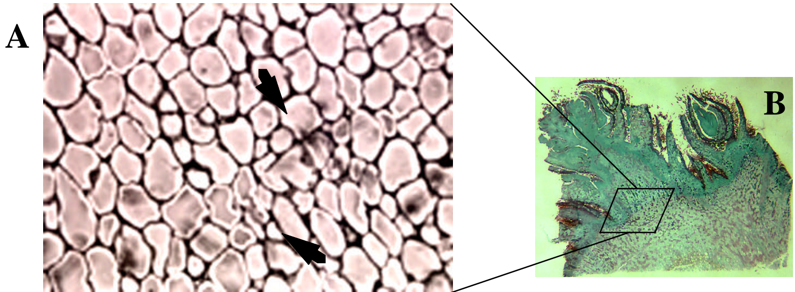
Fig. 3.2. A) Distorted and compressed zone of cells (40X) first appeared at 66 days after budbreak on 20 June, 1994 at the base of the primary bud axis of 'Riesling' buds from Somerset Vineyard, Virginia. B) A section of 'Riesling' bud with primary bud axis and two secondary bud axes.
