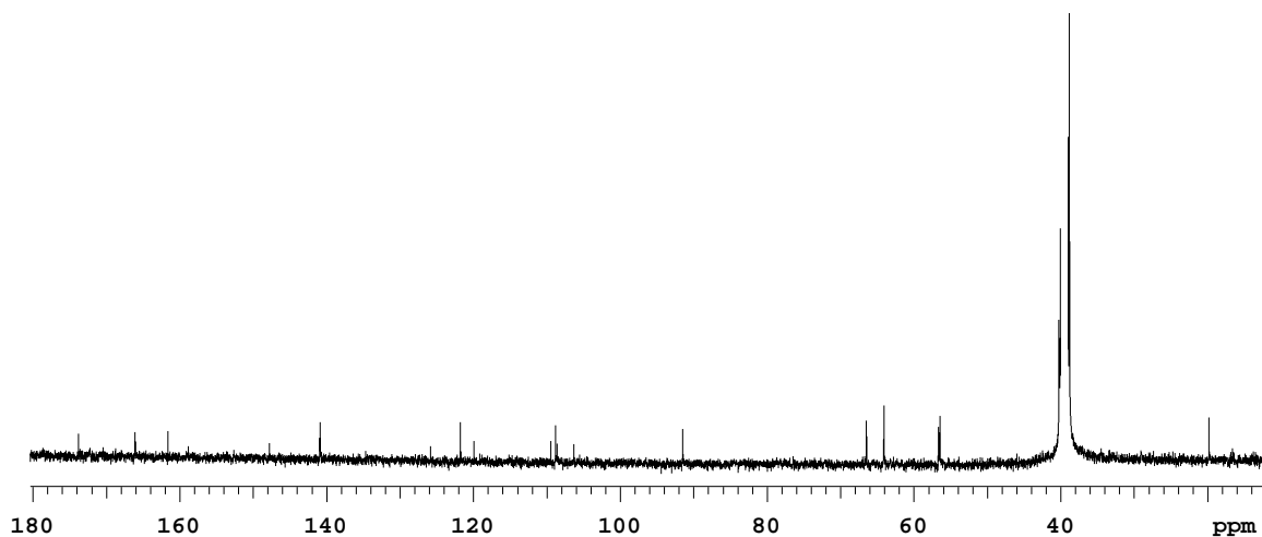
13 C-NMR Spectrum of Compound 3.58
