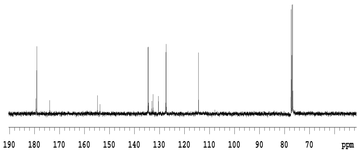
^{13}\text{C} -NMR Spectrum of Compound 3.33
