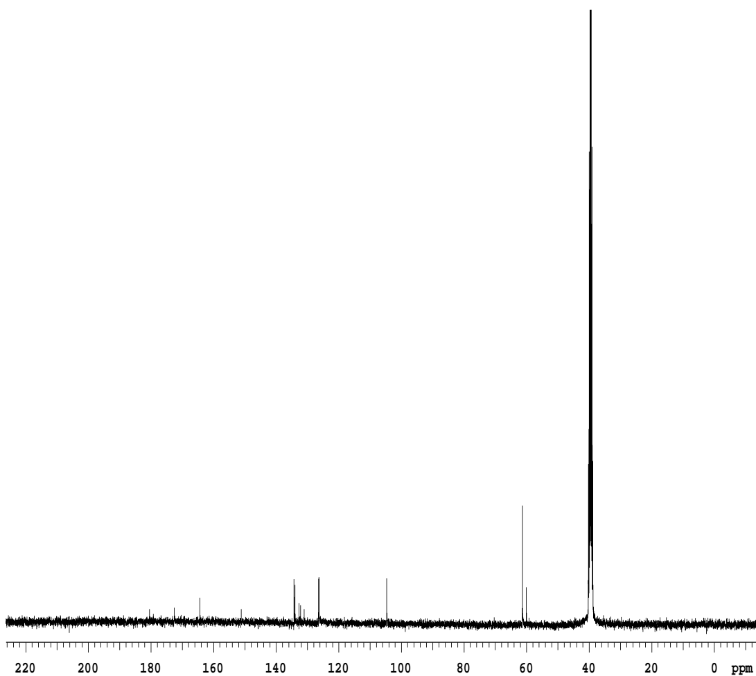
^{13}\text{C} -NMR Spectrum of Compound 3.35
