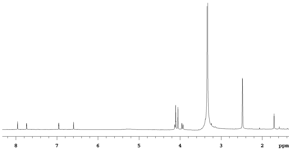
1 H-NMR Spectrum of Compound 3.58
