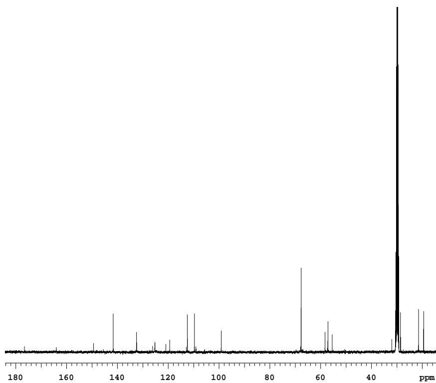
^{13}\text{C} -NMR Spectrum of Compound 3.52 (assignments on p.93)
