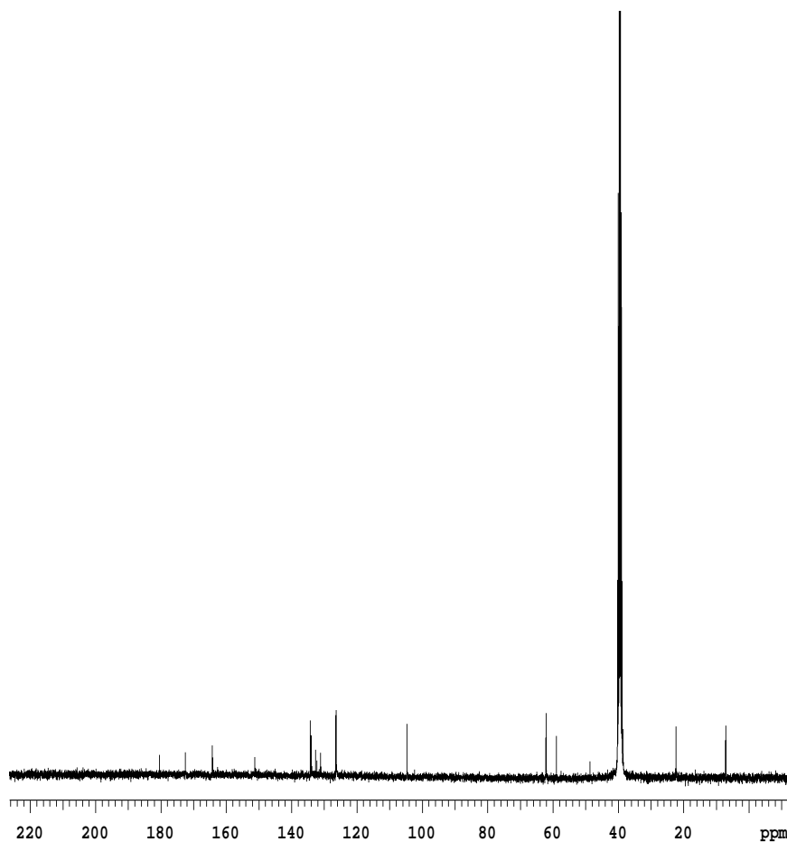
^{13}\text{C} -NMR Spectrum of Compound 3.36
