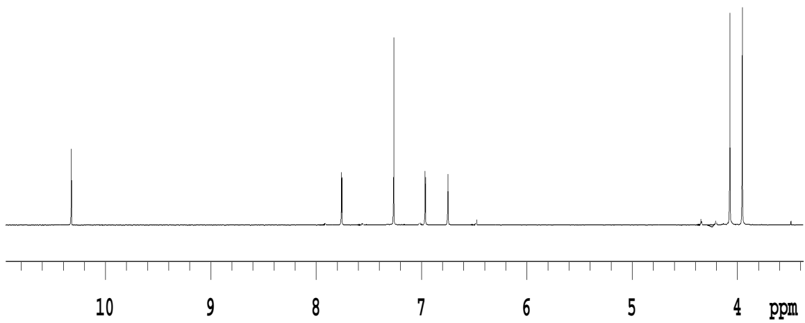
1 H-NMR Spectrum of Compound 3.56
