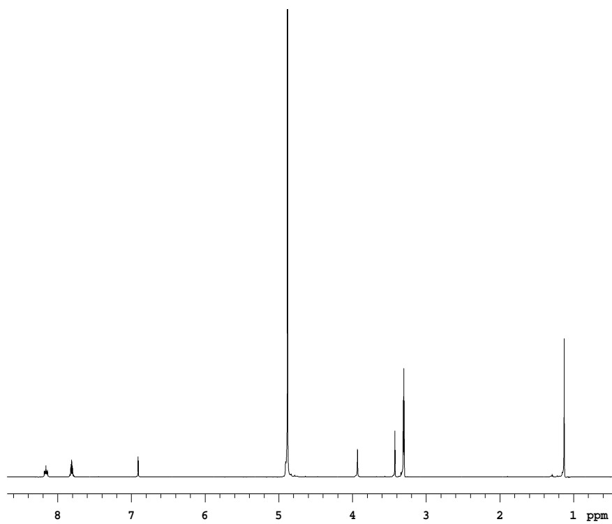
1 H-NMR Spectrum of Compound 3.34
