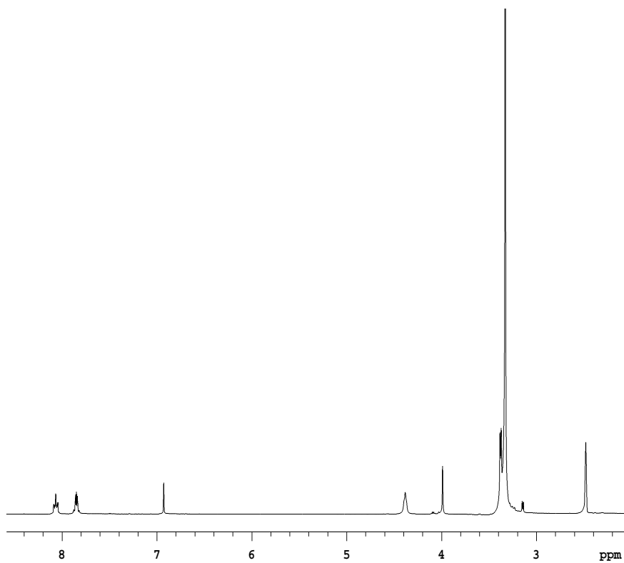
1 H-NMR Spectrum of Compound 3.35
