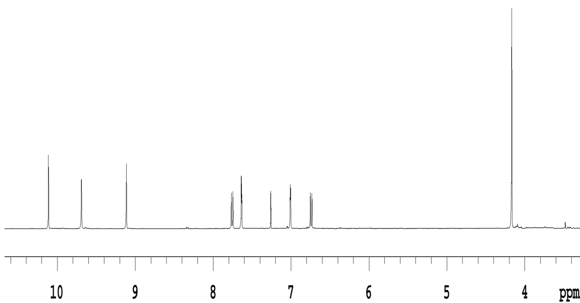
^1\text{H-NMR} Spectrum of Compound 3.44
