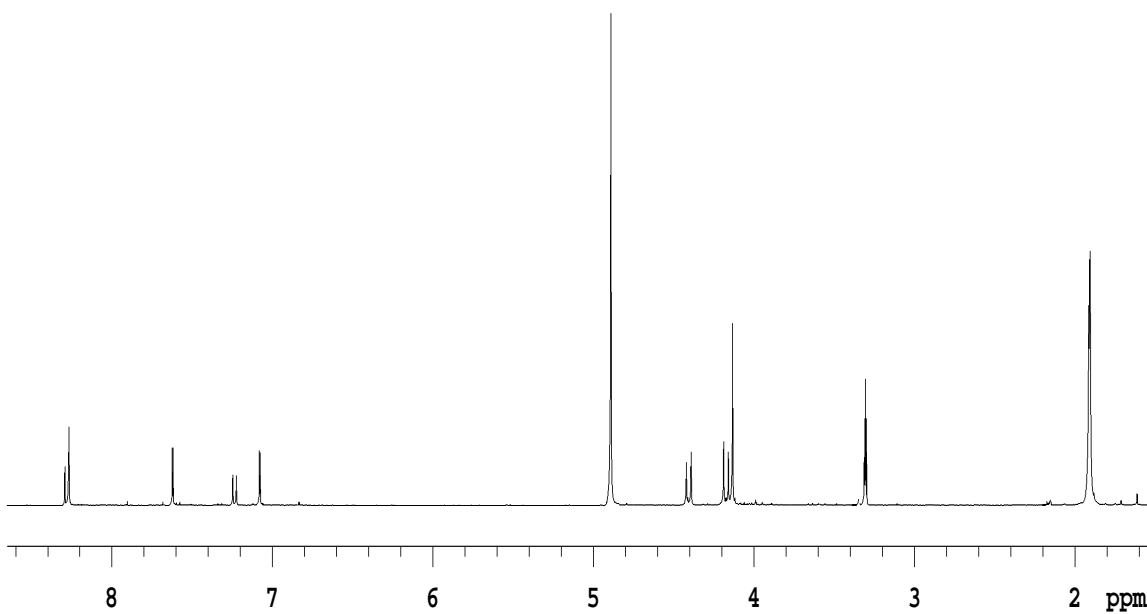
1 H-NMR Spectrum of Compound 3.54
