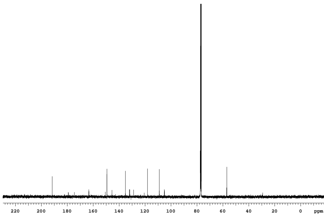
13 C-NMR Spectrum of Compound 3.45
