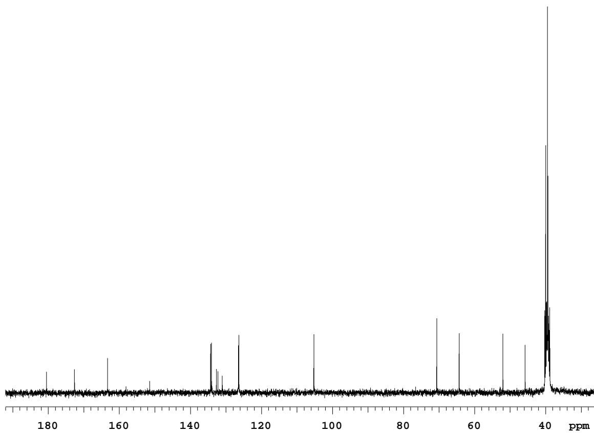
13 C-NMR Spectrum of Compound 3.37
