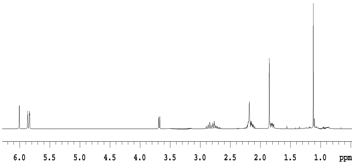
1 H-NMR Spectrum of Compound 2.31 (assignments on p.33)
