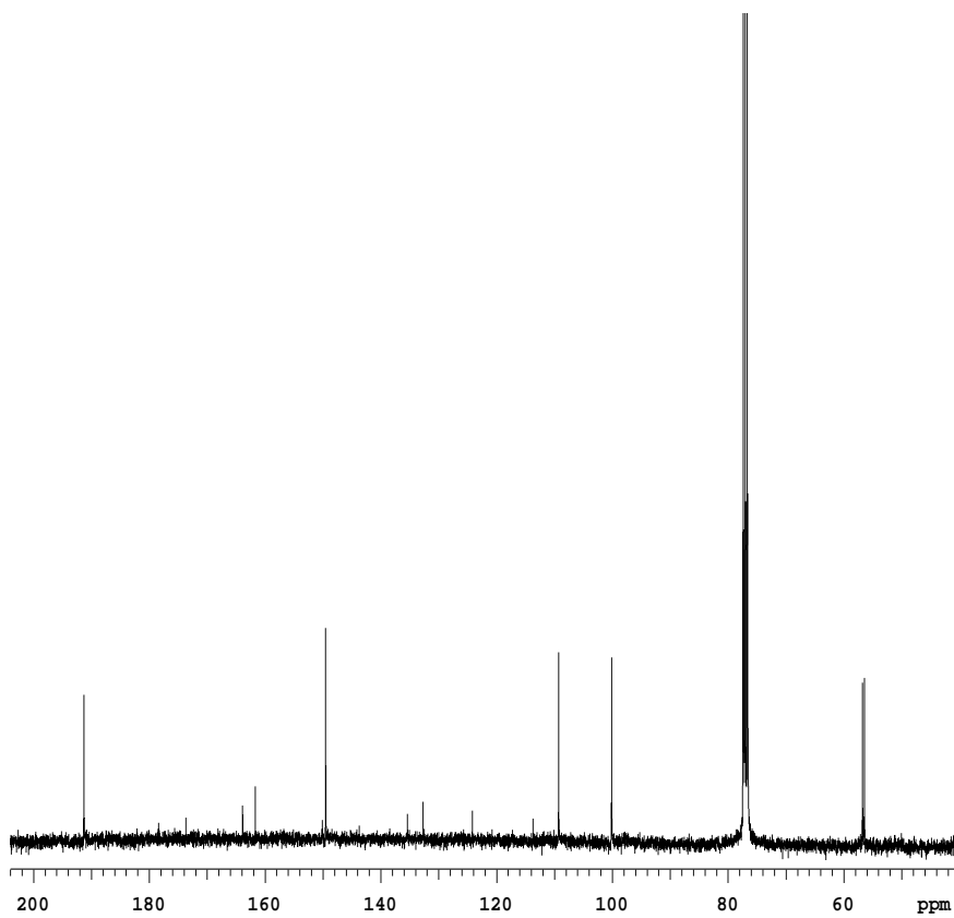
^{13}\text{C} -NMR Spectrum of Compound 3.56
