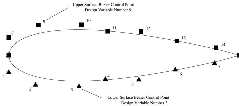
(b) Bezier curve parameterization with 14 design variables.
