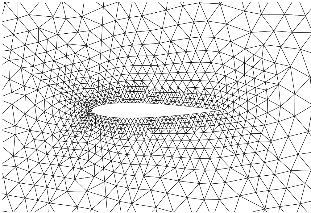
(a) Unstructured grid with 1,578 nodes and 3,044 triangular cells.
