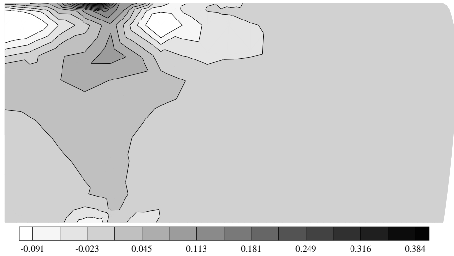
(b) Upper-surface sensitivity of pressure contours p/b_1 .
