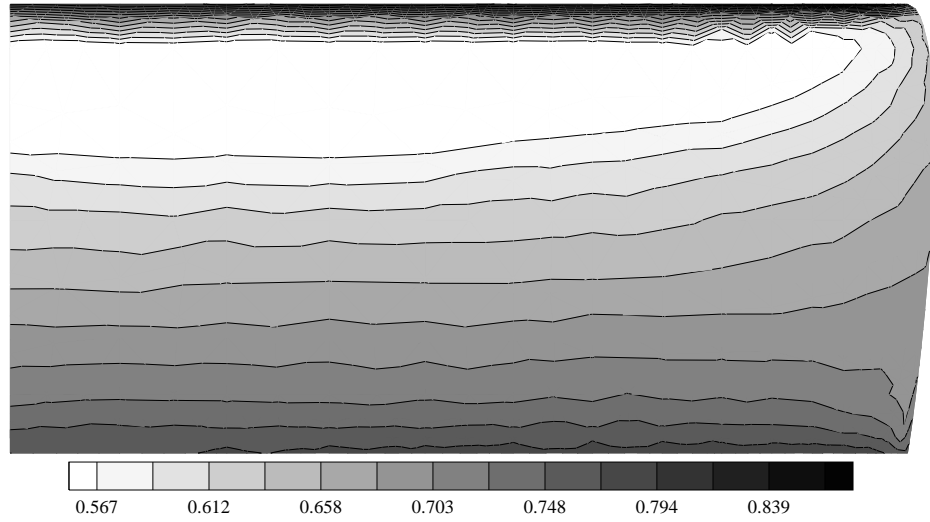
(a) Upper-surface pressure contours.
