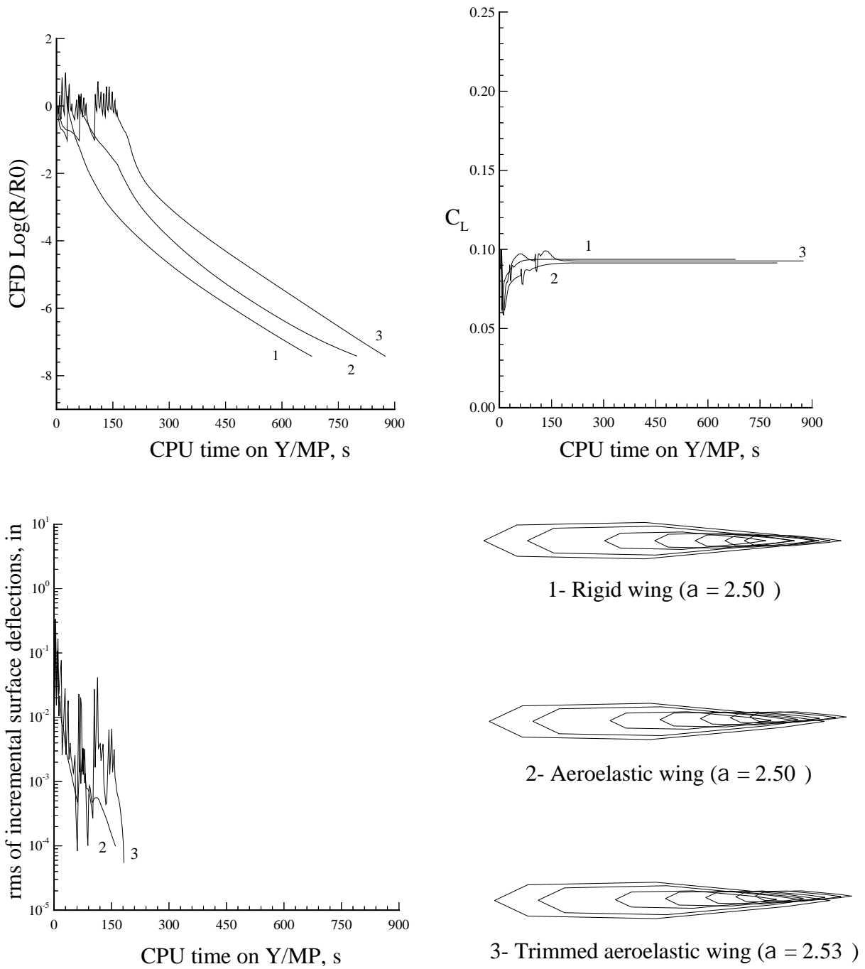
Figure 6.20: Aerodynamic and structural analysis interaction histories for low subsonic wing flow ( M_\infty = 0.3 , altitude = 35,000 ft).
