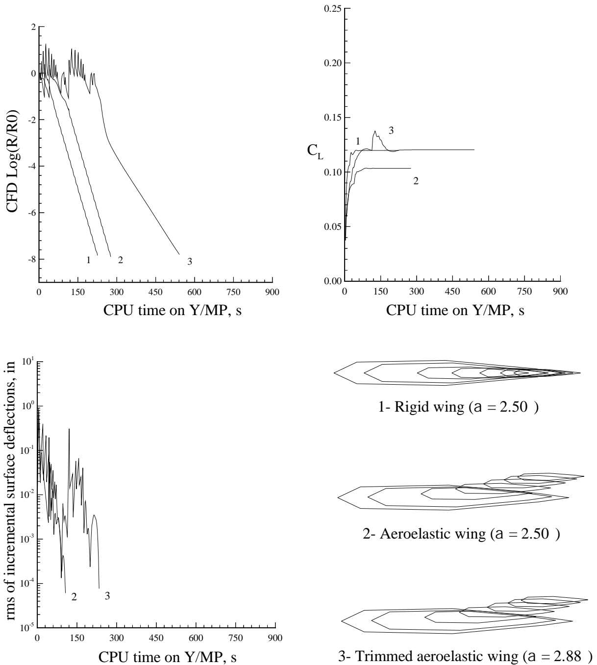
Figure 6.21: Aerodynamic and structural analysis interaction histories for subcritical wing flow ( M_\infty = 0.7 , altitude = 35,000 ft).
