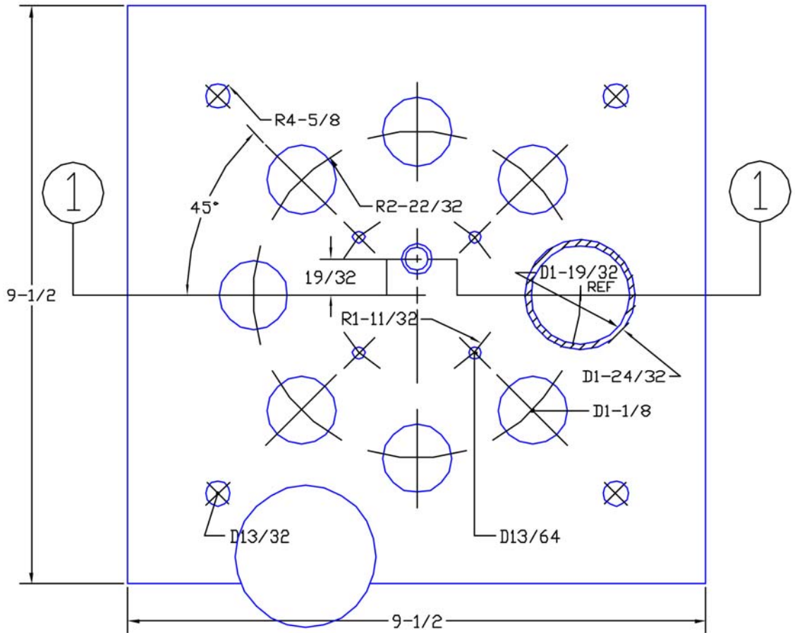
Cover Top View
