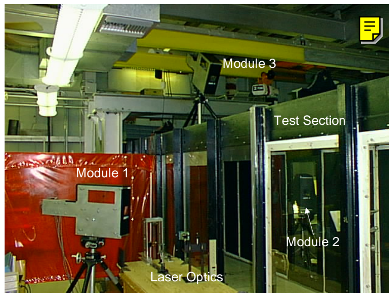
Figure 5.5: View from tunnel control room showing the DGV module positions
