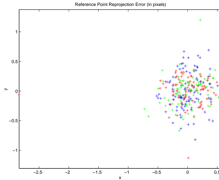
Figure B.1: Error, in pixels, of the analytical reprojection procedure using the calculated camera orientations, Camera 1 error=blue, Camera 2 error=red, Camera 3 error=green
