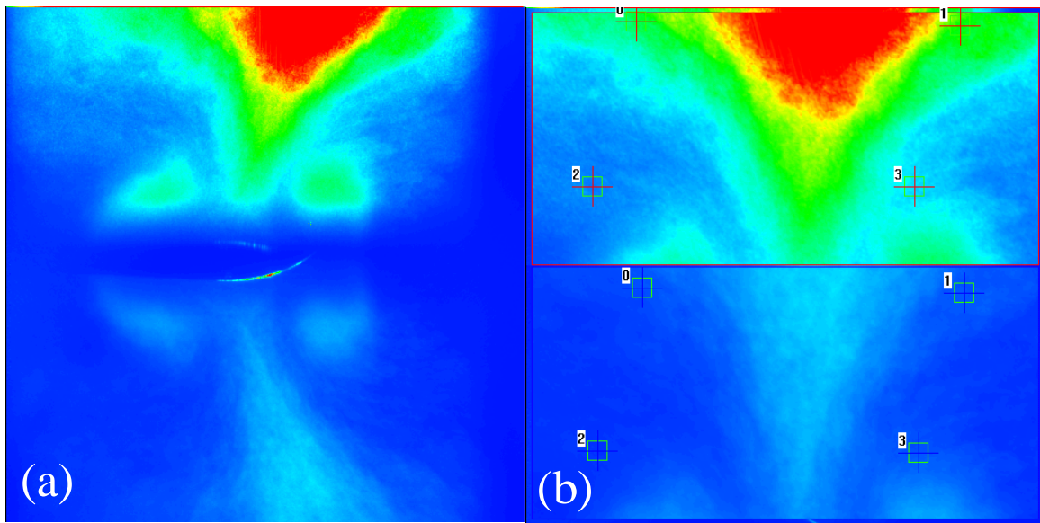
Figure 5.17: Module 2 views of prolate spheroid wake flow (a) raw data images (b) dewarped for processing
