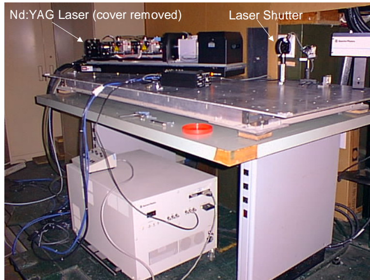
Figure 5.6: Nd:YAG laser system mounted below the Stability Tunnel test section
