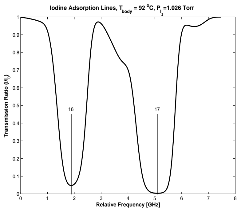
Figure 1.1: Example iodine transmission lines in the vicinity of 532\text{ nm} (output from a program by Forkey [37])
