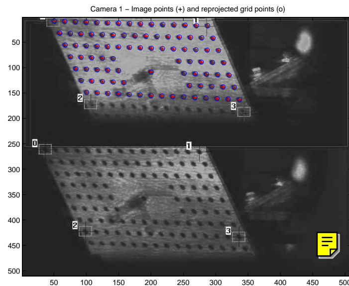
Figure B.2: Predicted reprojection points over the original input image points for Camera 1
