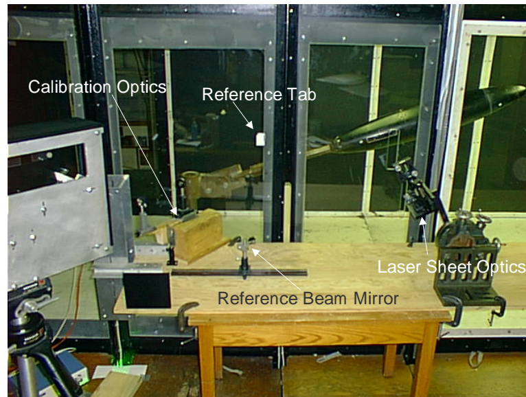
Figure 5.8: Control room view of laser optics, mounted prolate spheroid model and camera module 1
