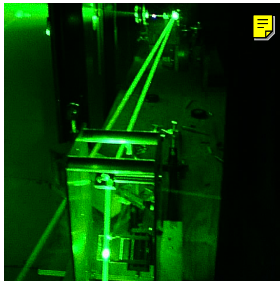
Figure 5.9: Picture of the laser optics during a test, from over the periscope (note the back reflection from the laser sheet mirror)
