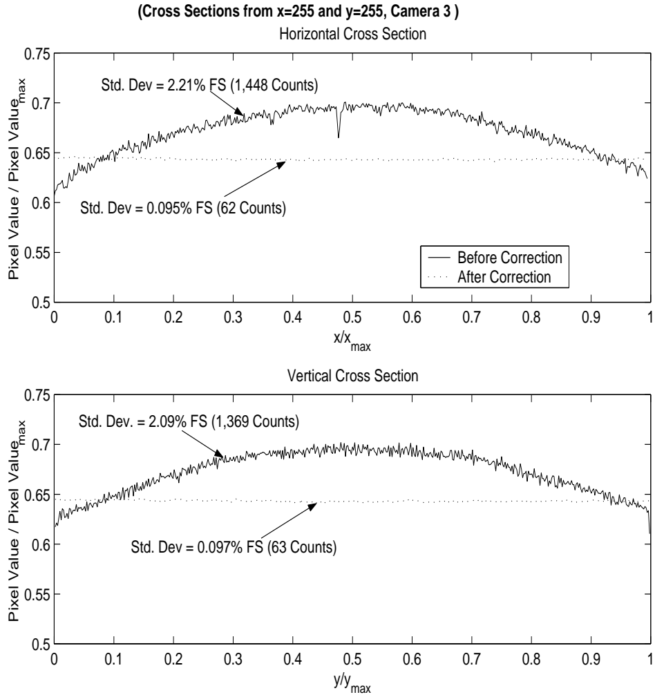
Figure 4.4: Horizontal and vertical mid-image cross sections showing the effectiveness of pixel sensitivity correction
