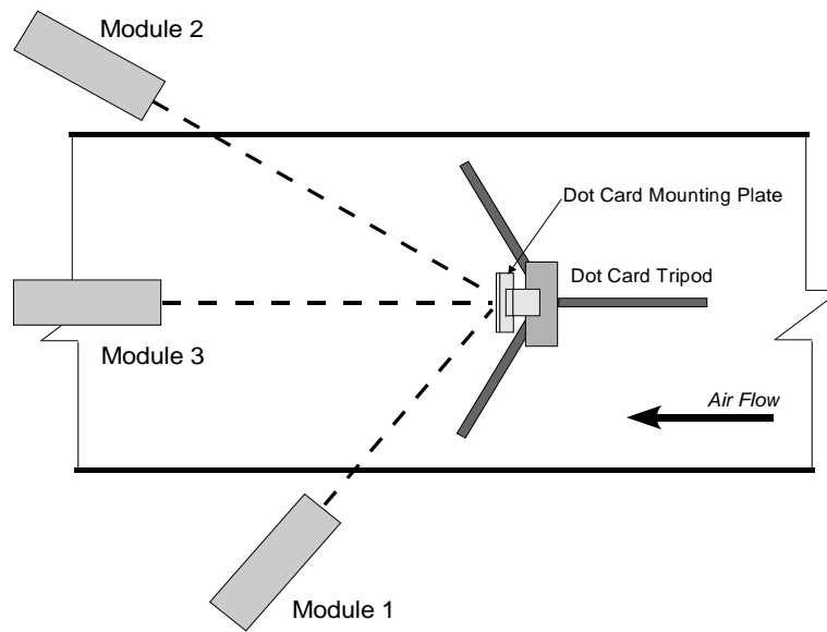
Figure 5.4: Top view of DGV module positions
