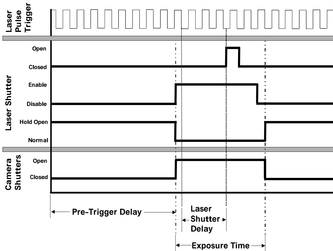
Figure 3.11: Virginia Tech DGV Control program steady measurement timing diagram. Note the laser pulses are not to drawn to scale for clarity. Typical time values are: Pre-Trigger Delay = 2000ms, Laser Shutter Delay = 500ms and Exposure Time = 3000ms (laser shutter always remains open for 100ms)
