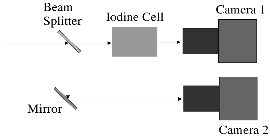
Figure 3.4: Schematic of a two-camera DGV measurement component used by Meyers [15]
