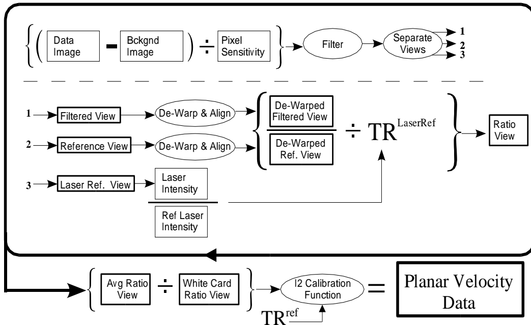
Figure 4.3: Diagram of DGV data reduction procedure
