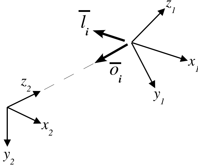
Figure A.1: Definition of primary and observer coordinate systems
