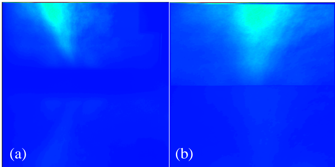
Figure 5.16: Module 1 views of prolate spheroid wake flow (a) raw data images (b) dewarped for processing
