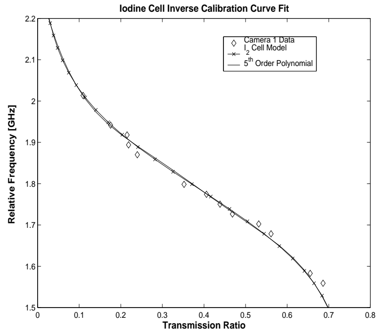
Figure 4.11: DGV velocity calculation iodine calibration function
