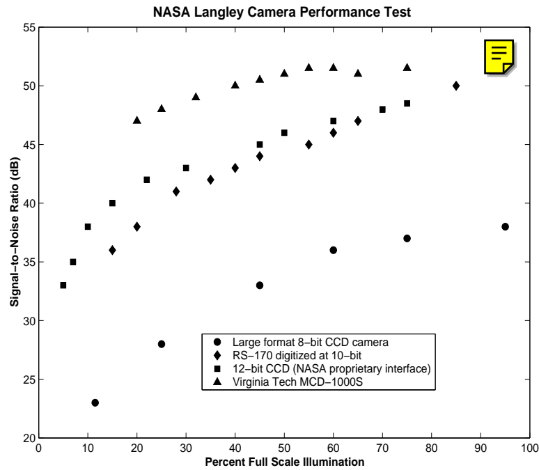
Figure 3.2: Camera performance comparison from NASA Langley tests conducted by G. Fleming [33] (exact model names of other tested systems were withheld)
