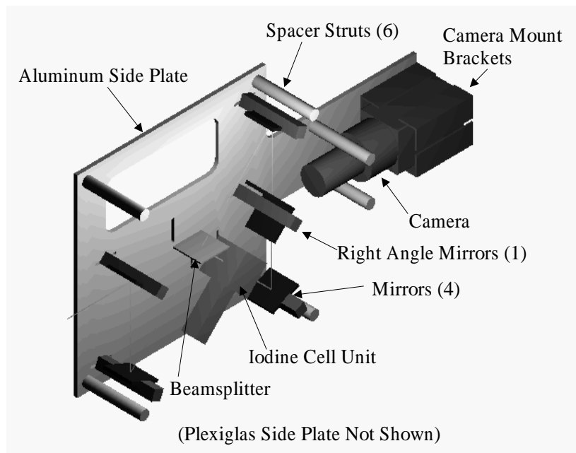
Figure 3.7: Virginia Tech DGV module design features
