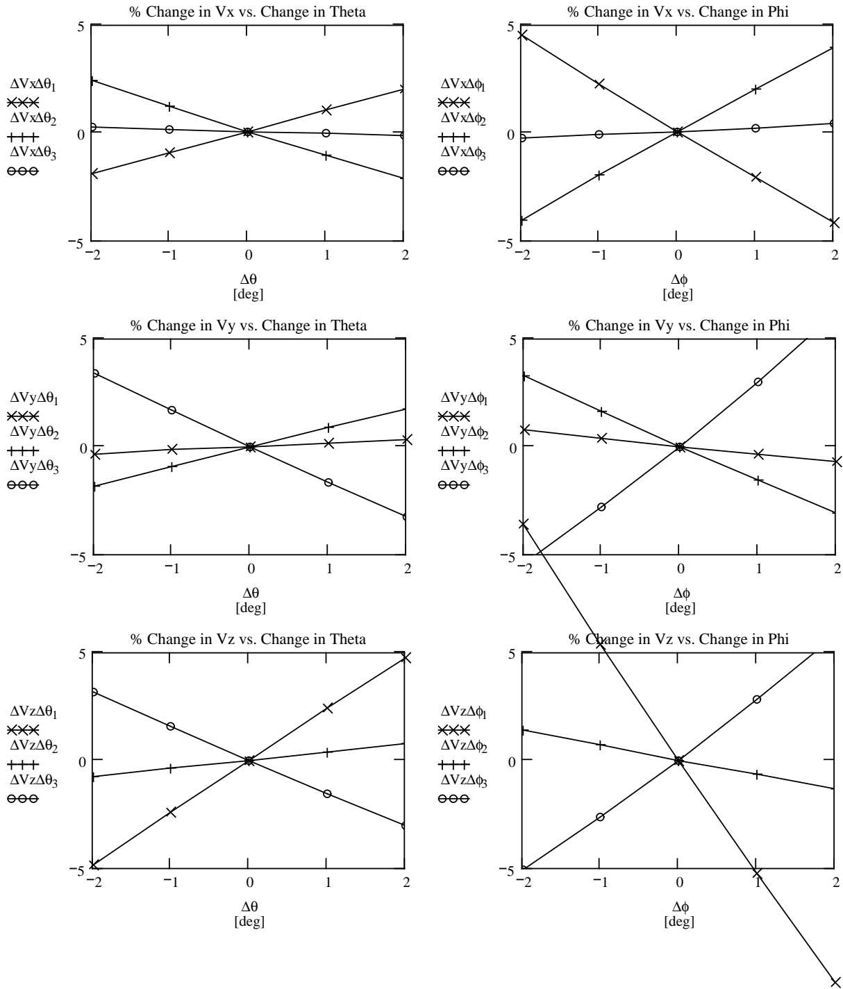
Figure C.2: Velocity component sensitivity with changes in Euler rotation angles
