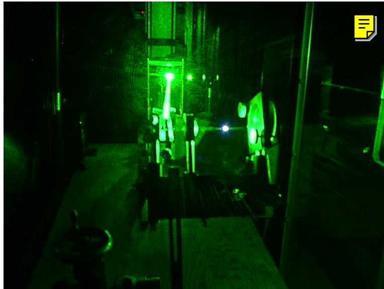
Figure 5.10: Close up of laser sheet optics during a test (note the cutout in the Plexiglas window for laser sheet)
