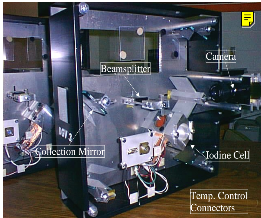
Figure 3.8: Completed Virginia Tech DGV module (close-up)
