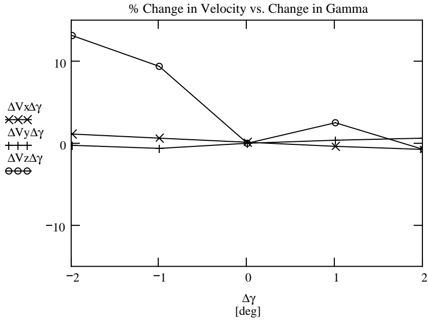
Figure C.3: Velocity component sensitivity with changes in the laser plane horizontal angle
