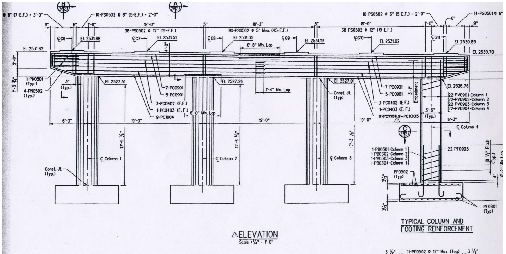
Figure 4.6. The East Bound Pier Elevation [Brown, 1993].
