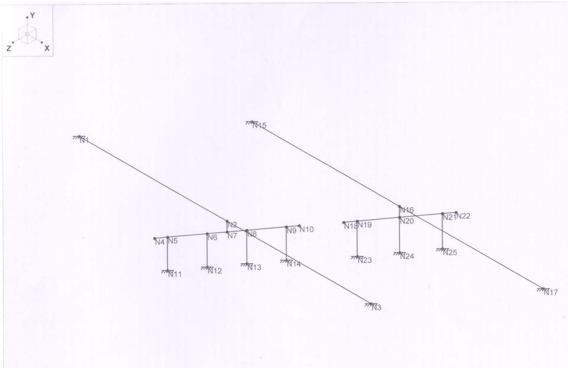
Figure 4.7. The RISA 3D model of the WB bridge (left) and EB bridge (right).
