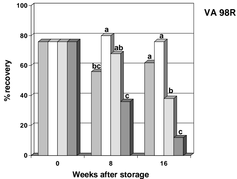
Fig. 1. Recovery of Cylindrocladium parasiticum from speckled peanut seed of NC-V 11 and VA 98R during winter seed storage. Seeds were assayed on a selective medium at 0, 8, 16, and 24 weeks after storage. Bars from left to right for each time interval reflect storage at -13 , 4 , 15^{\circ}\text{C} , and ambient temperatures in an unheated building. Bars with the same letter or no letters are not significantly different according to Duncan's new multiple range test ( P=0.05 ).
