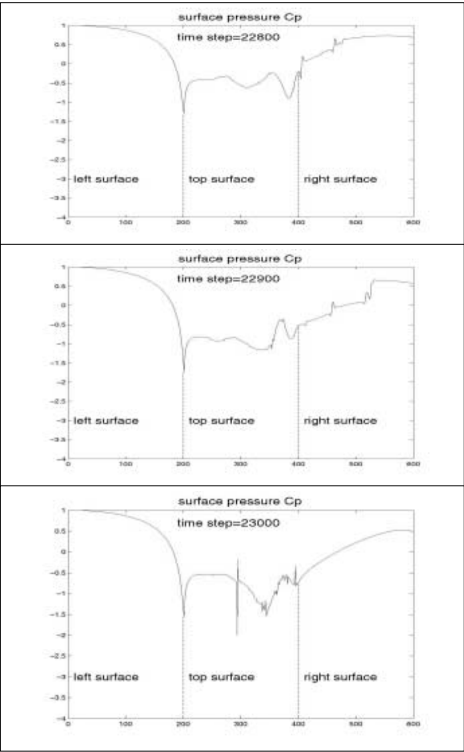
Fig. 4.25 Surface pressure C_p
