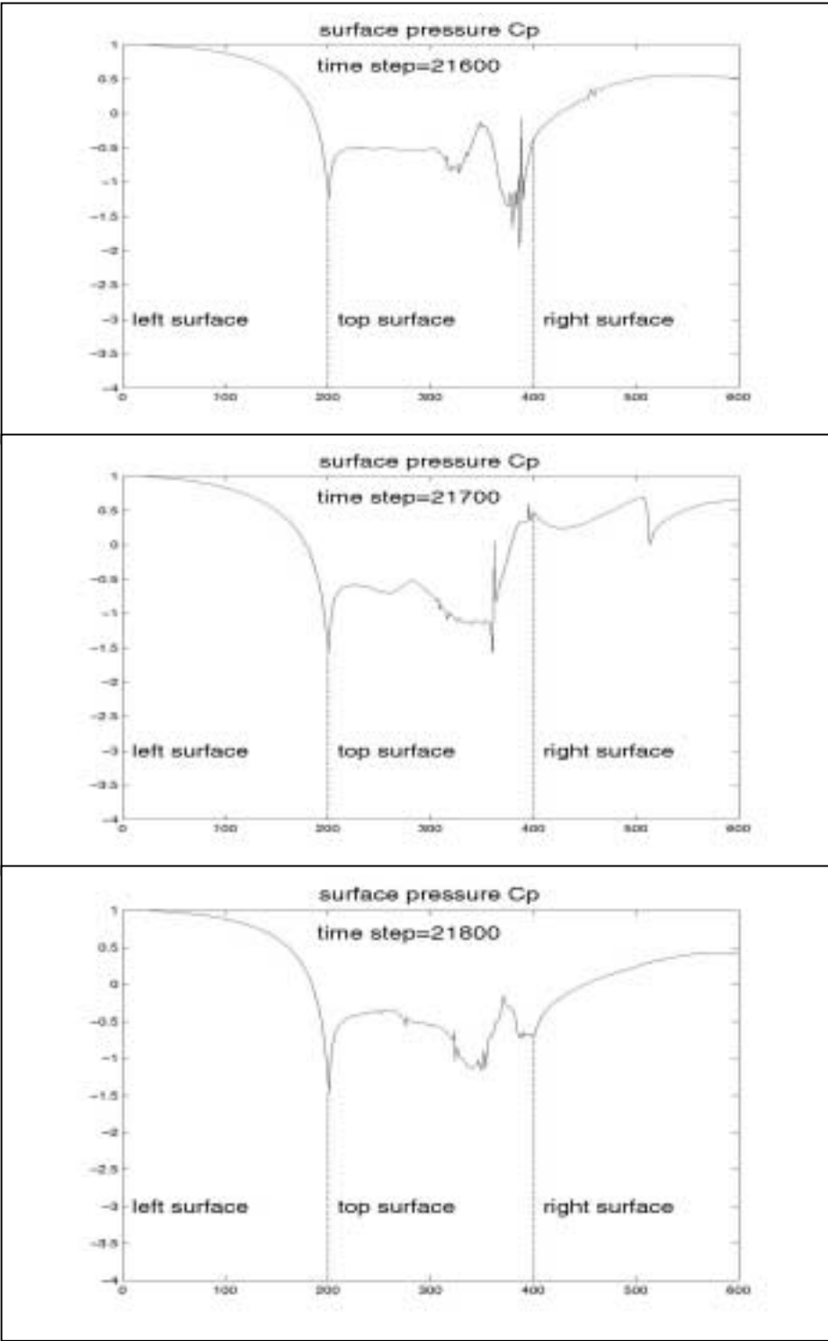
Fig. 4.21 Surface pressure C_p
