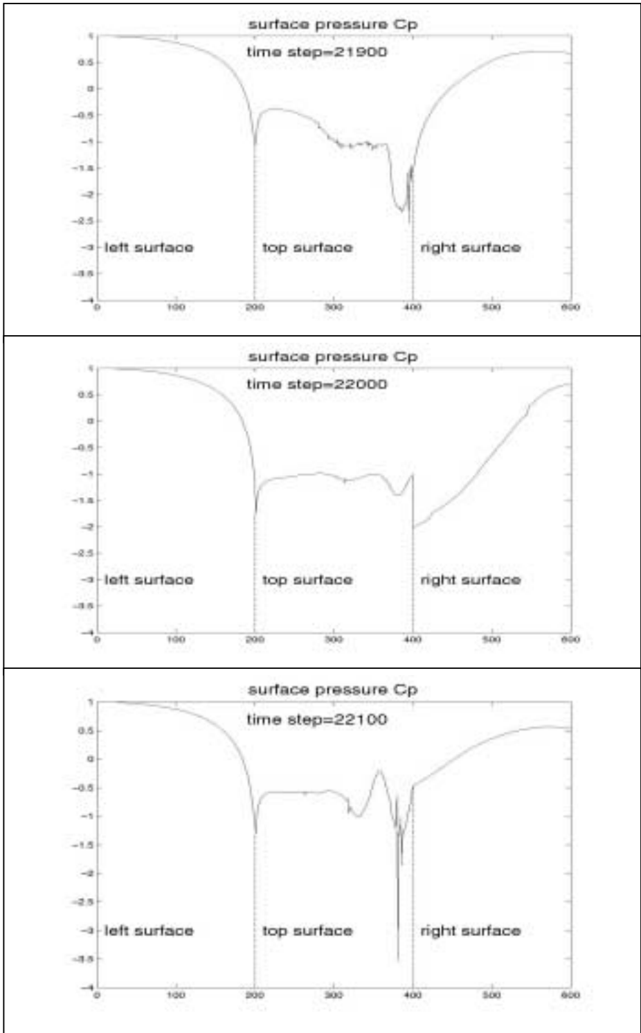
Fig. 4.22 Surface pressure C_p
