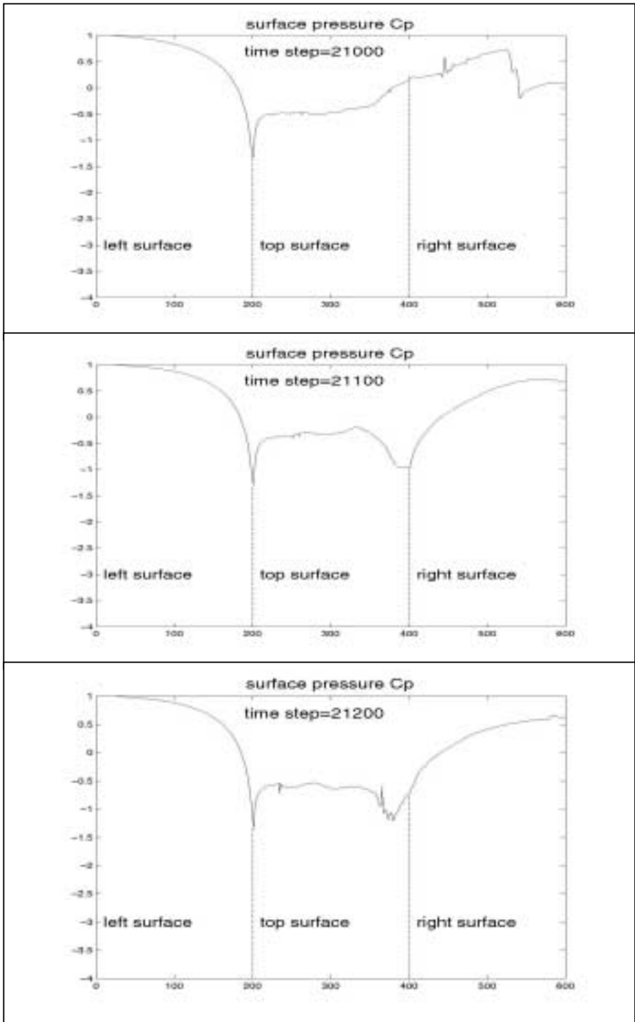
Fig. 4.19 Surface pressure C_p
