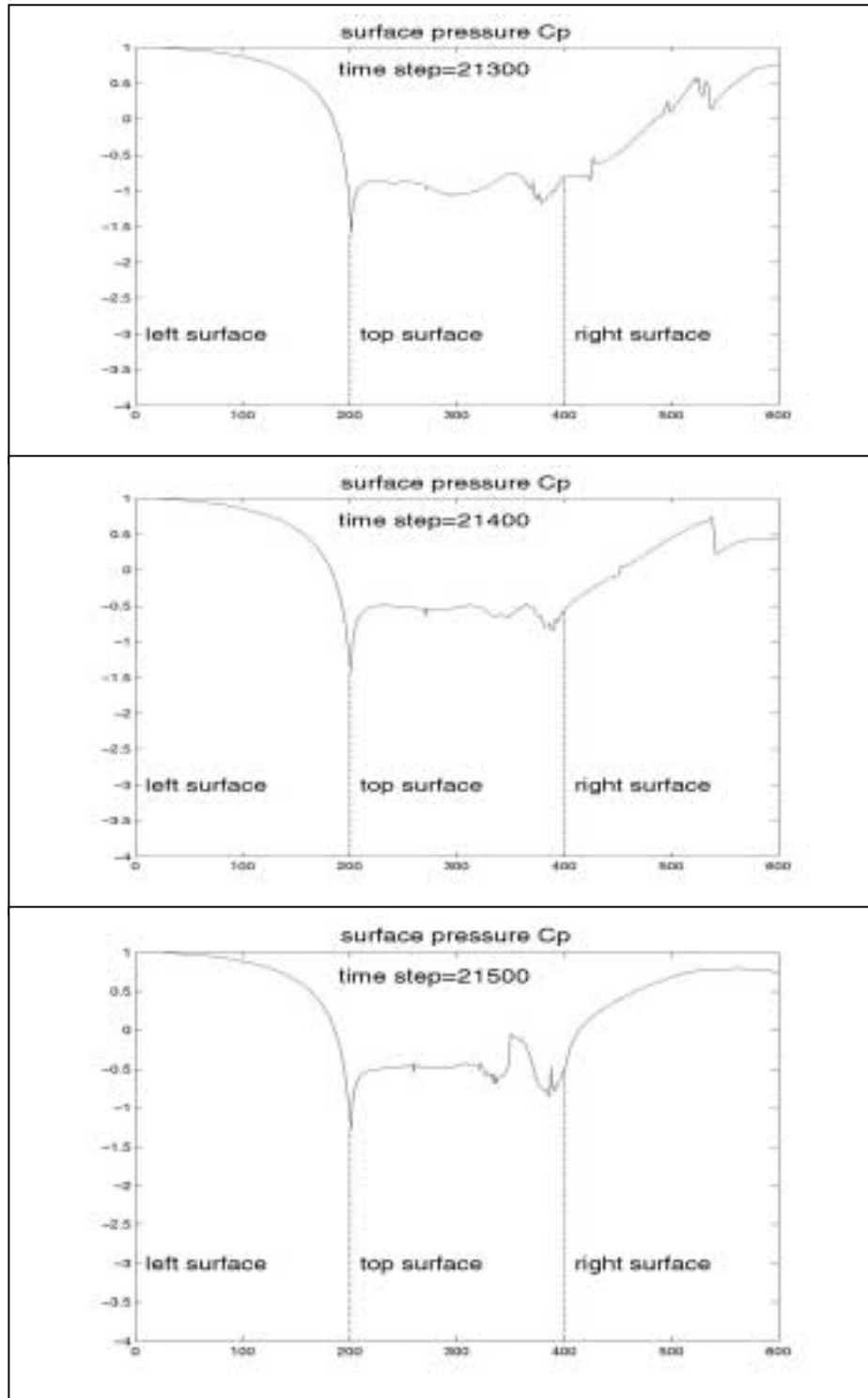
Fig. 4.20 Surface pressure C_p
