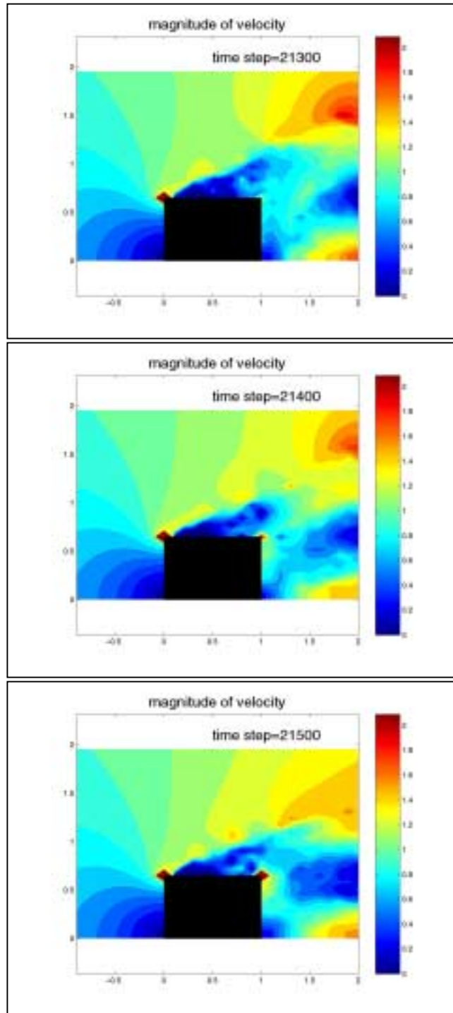
Fig. 4.6 Velocity magnitude
