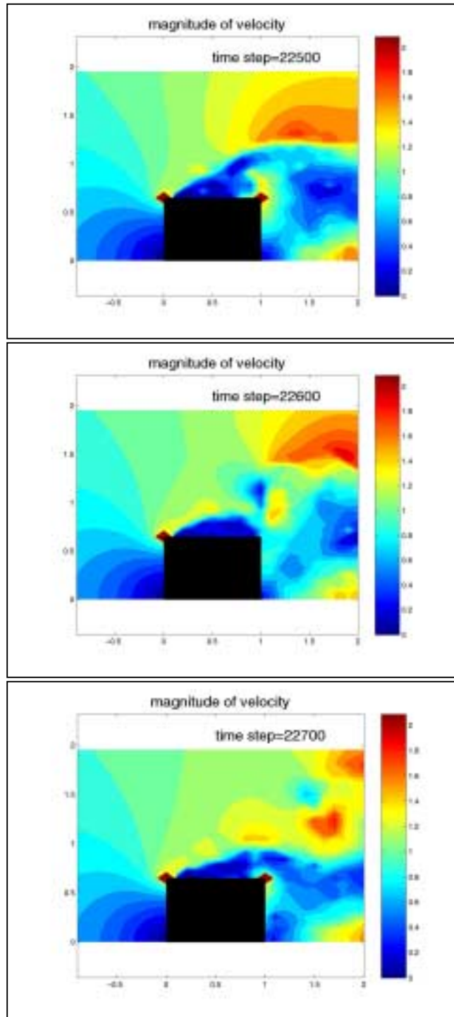
Fig. 4.10 Velocity magnitude
