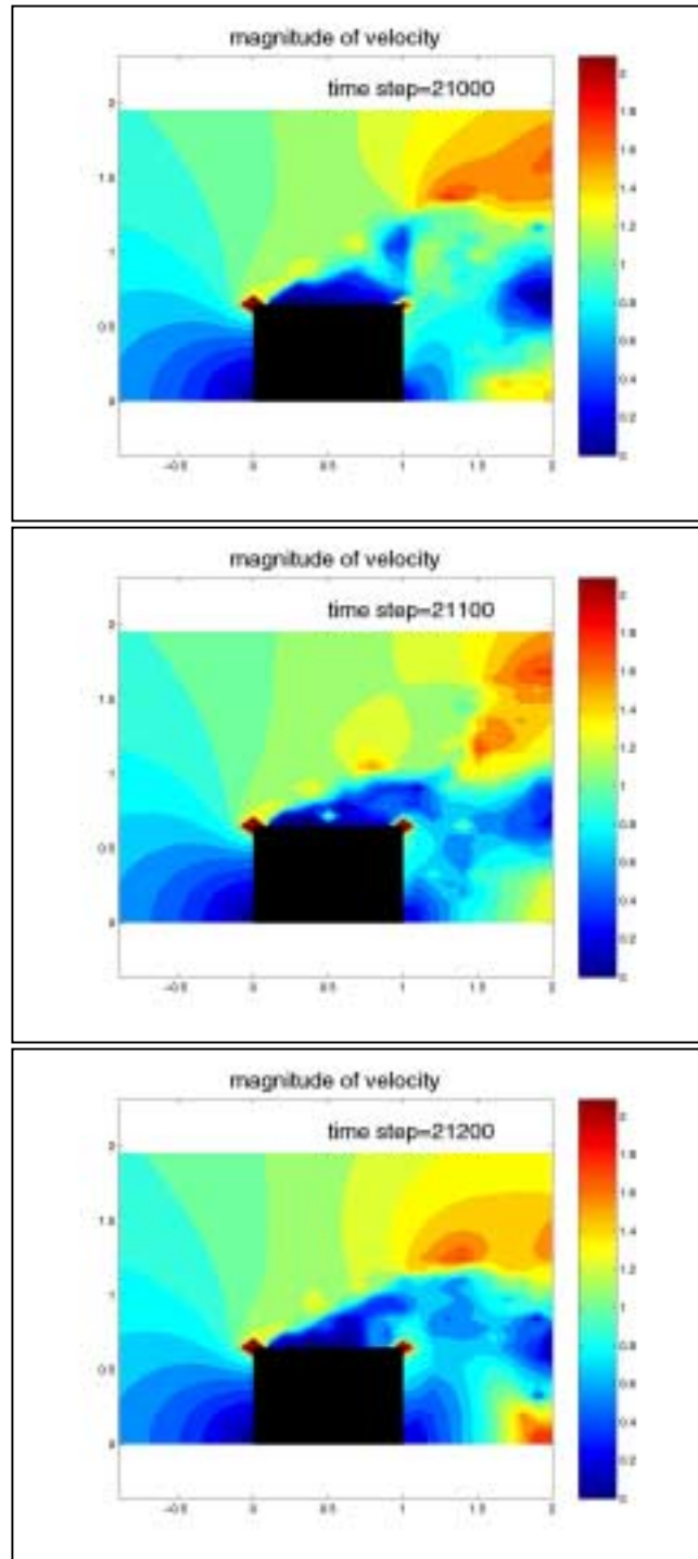
Fig. 4.5 Velocity magnitude
