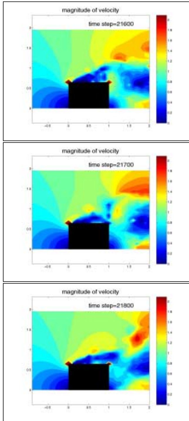
Fig. 4.7 Velocity magnitude
