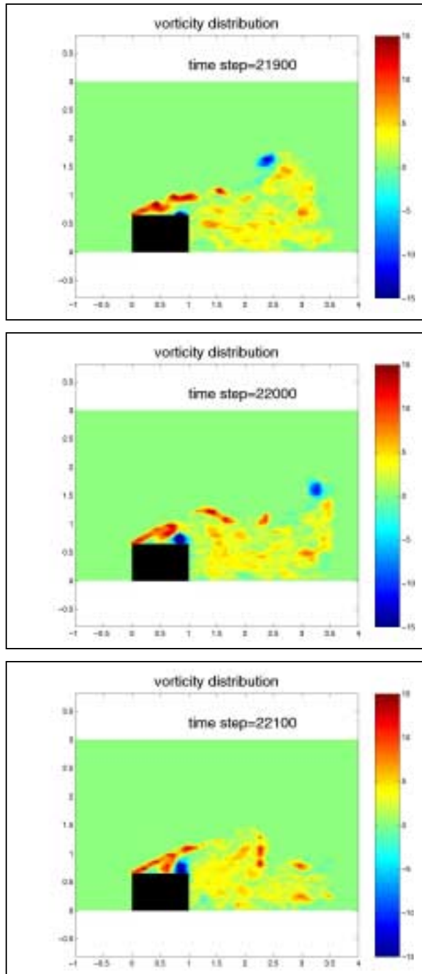
Fig. 4.15 Vorticity
