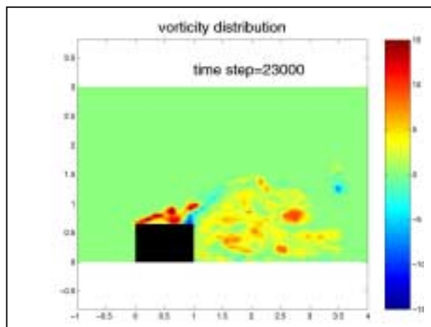
Fig. 4.18 Vorticity
