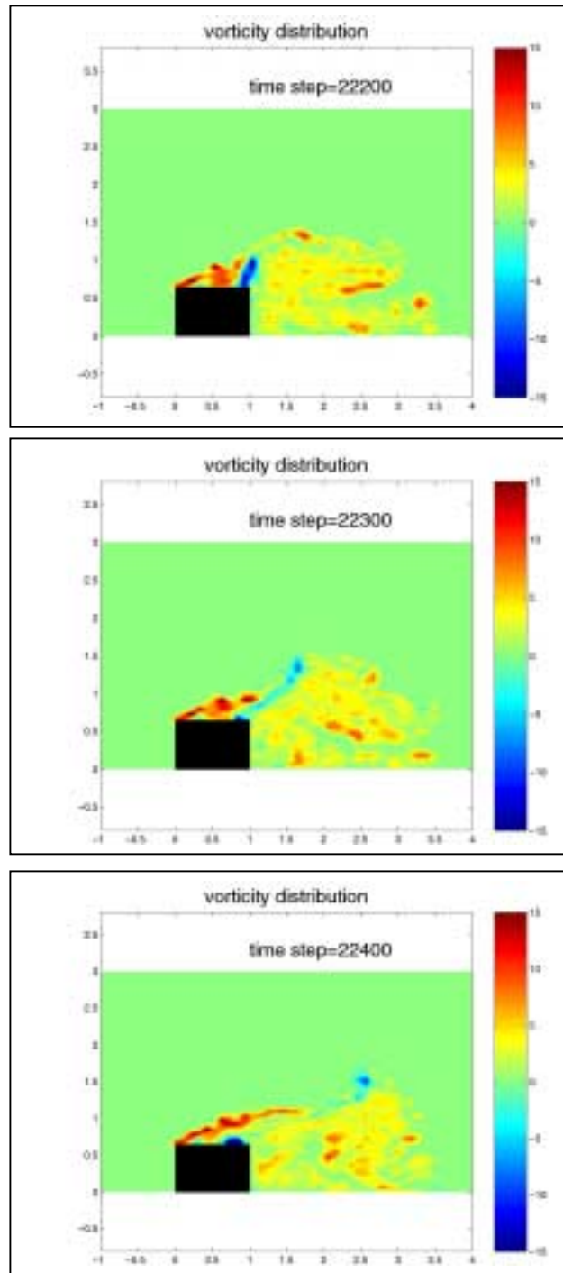
Fig. 4.16 Vorticity
