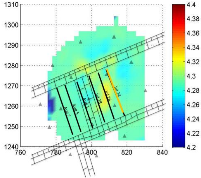
Figure C.2.3: TomoDD Tomogram from 7/24/1997
