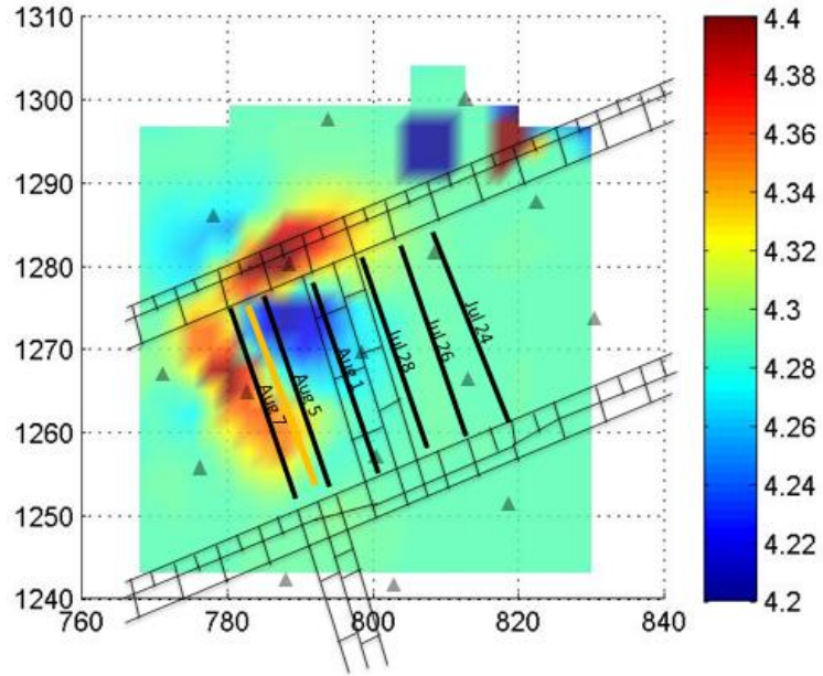
Figure C.2.13: TomoDD Tomogram from 8/6/1997
