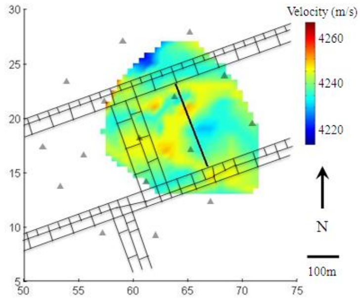
Figure C.1.3:SIMULPS Tomogram from 7/24/1997
