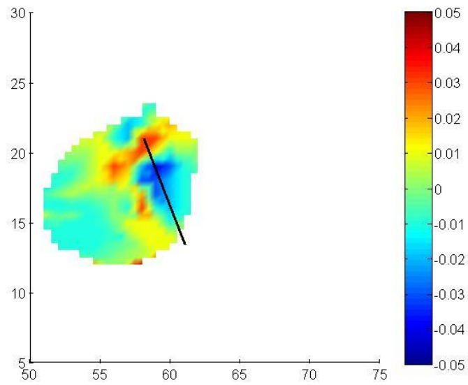
Figure C.1.8: SIMULPS Tomogram from 8/2/1997
