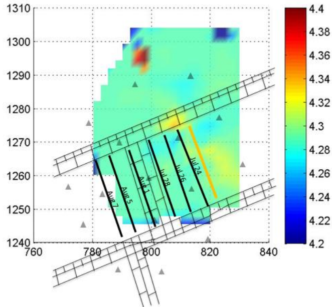
Figure C.2.1: TomoDD Tomogram from 7/21/1997
