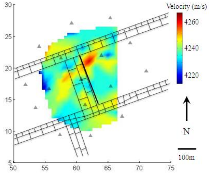
Figure C.1.5:SIMULPS Tomogram from 7/28/1997
