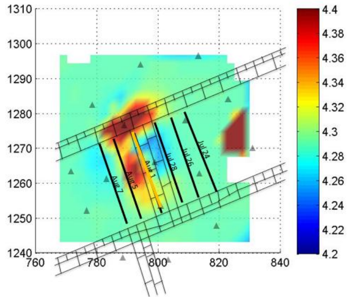
Figure C.2.8: TomoDD Tomogram from 8/1/1997
