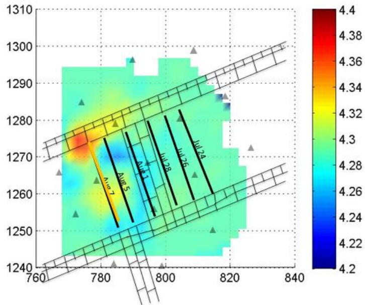
Figure C.2.14: TomoDD Tomogram from 8/7/1997
