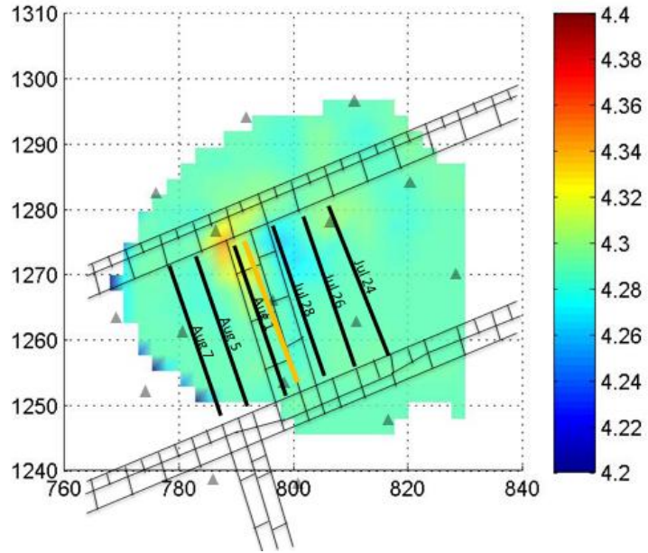
Figure C.2.7: TomoDD Tomogram from 7/31/1997
