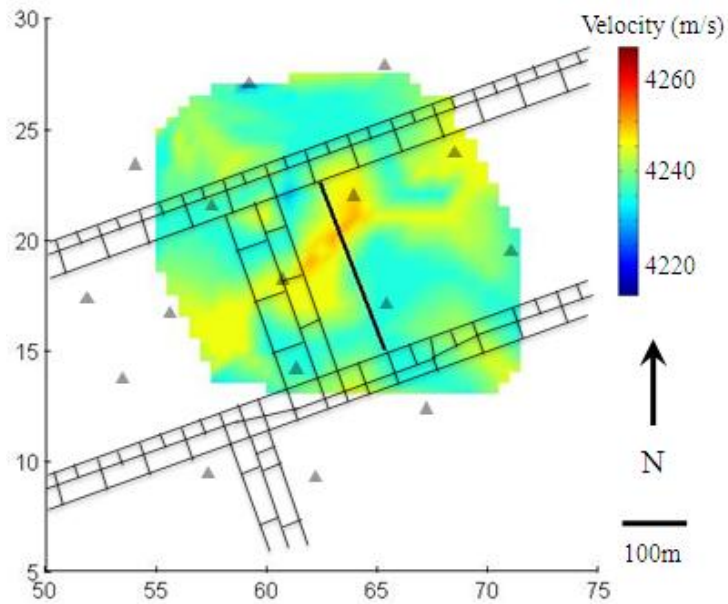
Figure C.1.4:SIMULPS Tomogram from 7/26/1997
