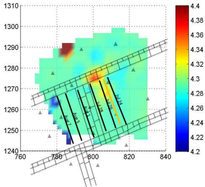
Figure C.2.4: TomoDD Tomogram from 7/26/1997
