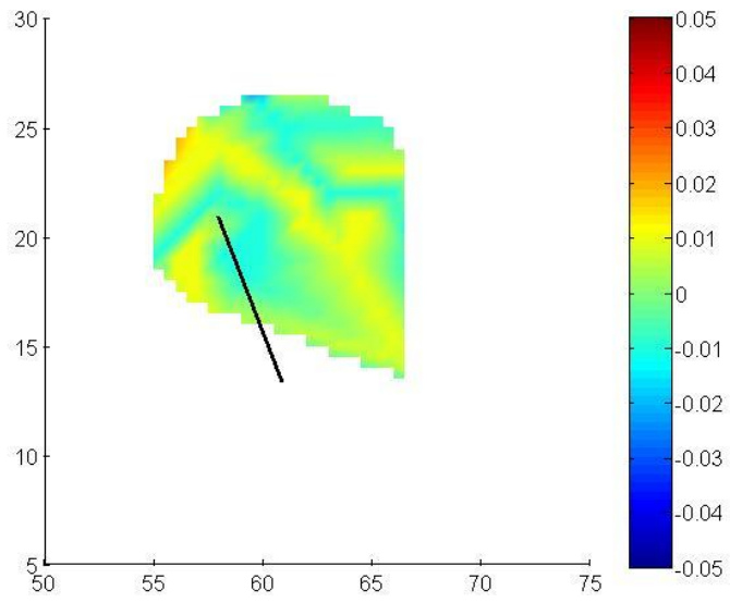
Figure C.1.9: SIMULPS Tomogram from 8/3/1997
