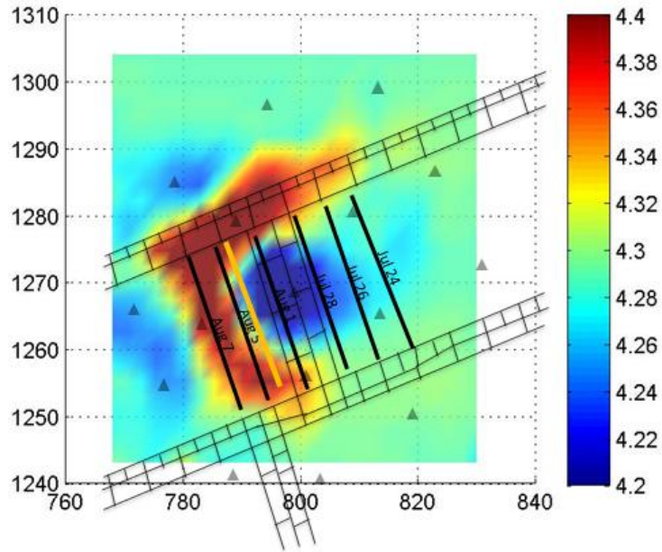
Figure C.2.11: TomoDD Tomogram from 8/4/1997
