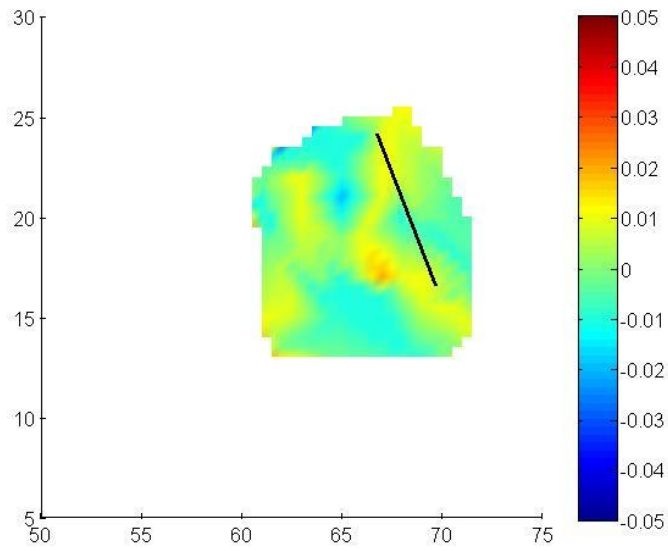
Figure C.1.1: SIMULPS Tomogram from 7/21/1997
