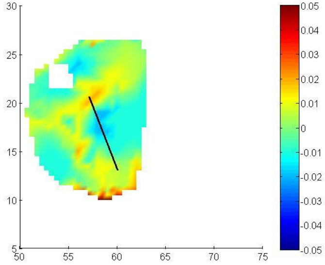
Figure C.1.10: SIMULPS Tomogram from 8/4/1997
