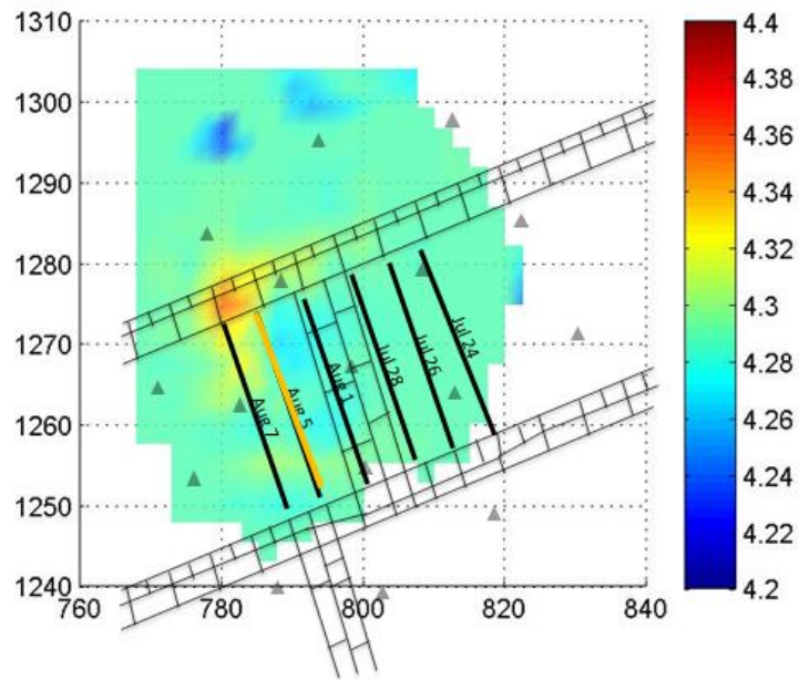
Figure C.2.12: TomoDD Tomogram from 8/5/1997
