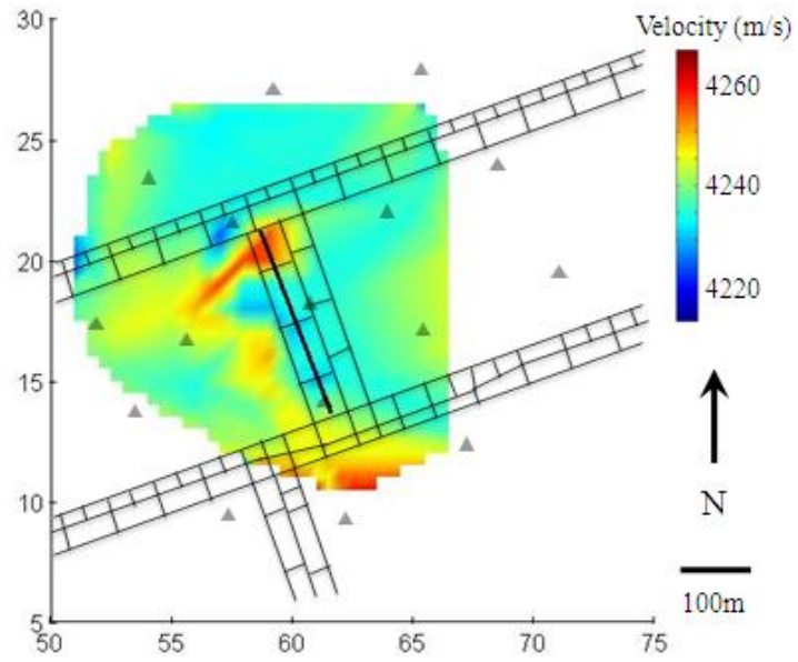
Figure C.1.7: SIMULPS Tomogram from 8/1/1997
