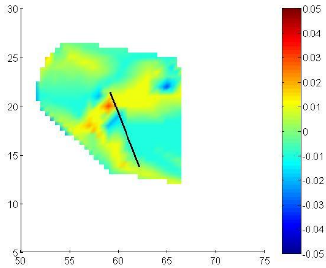
Figure C.1.6: SIMULPS Tomogram from 7/31/1997
