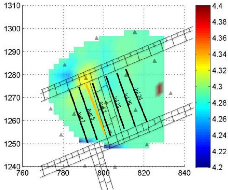
Figure C.2.10: TomoDD Tomogram from 8/3/1997
