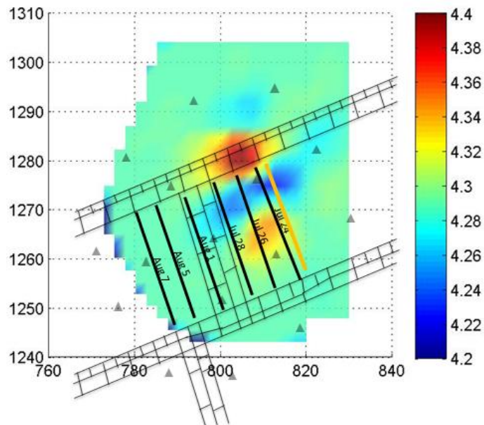
Figure C.2.2: TomoDD Tomogram from 7/23/1997
