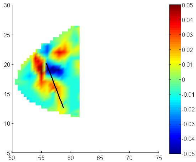
Figure C.1.12: SIMULPS Tomogram from 8/6/1997
