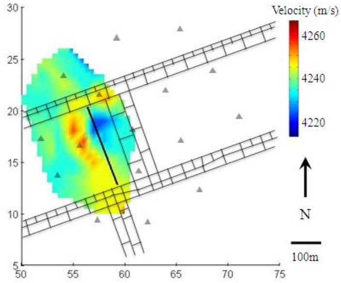
Figure C.1.11: SIMULPS Tomogram from 8/5/1997
