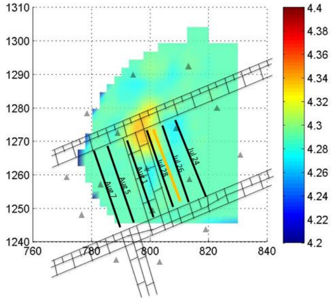
Figure C.2.5: TomoDD Tomogram from 7/27/1997
