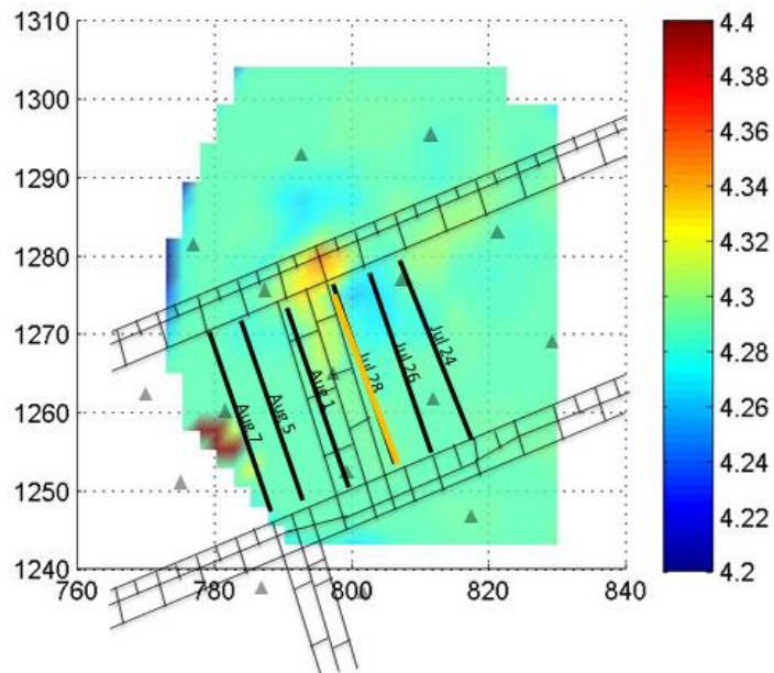
Figure C.2.6: TomoDD Tomogram from 7/28/1997
