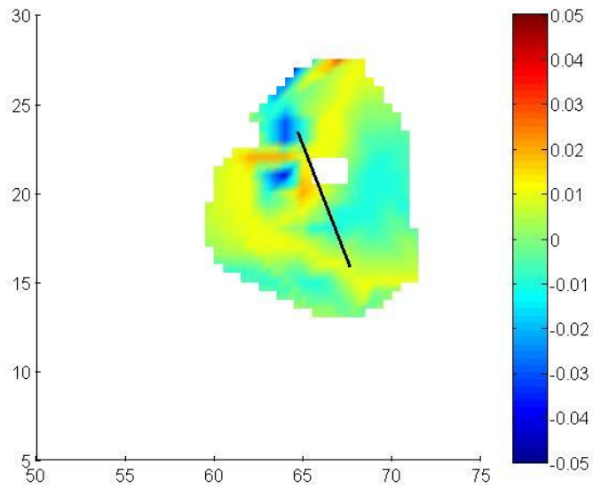
Figure C.1.2: SIMULPS Tomogram from 7/23/1997
