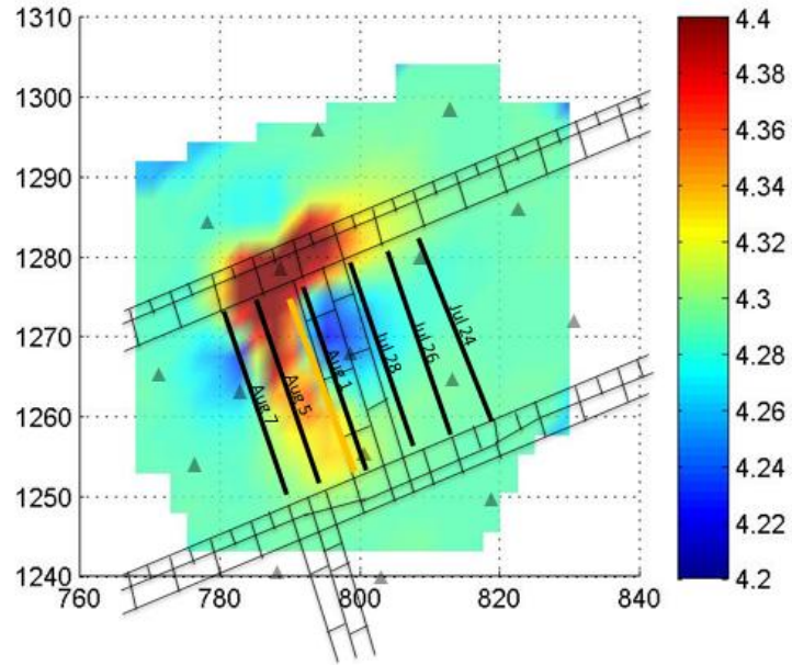
Figure C.2.9: TomoDD Tomogram from 8/2/1997
