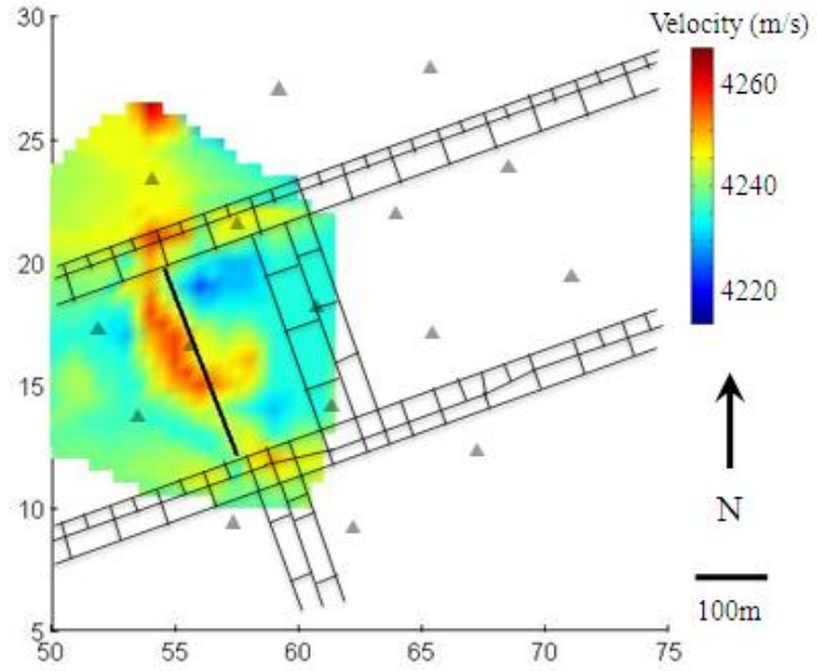
Figure C.1.13: SIMULPS Tomogram from 8/7/1997
