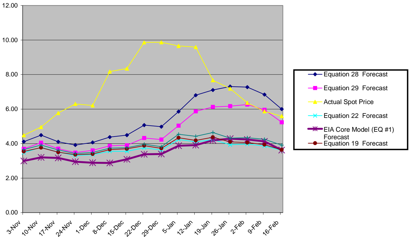
Figure 5 - Forecast Results using the Best 5 In-Sample Equations vs EIA Core Model and Actual Spot Price
