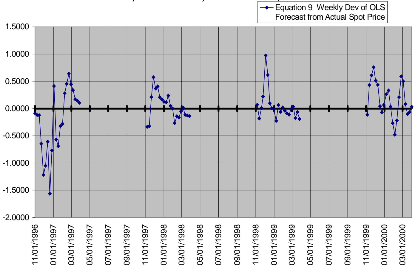
Figure F - 21 Equation 9 using Variables SP[-4], F2LAG4, SPOILL4, WTTEDL4,STORDEV
