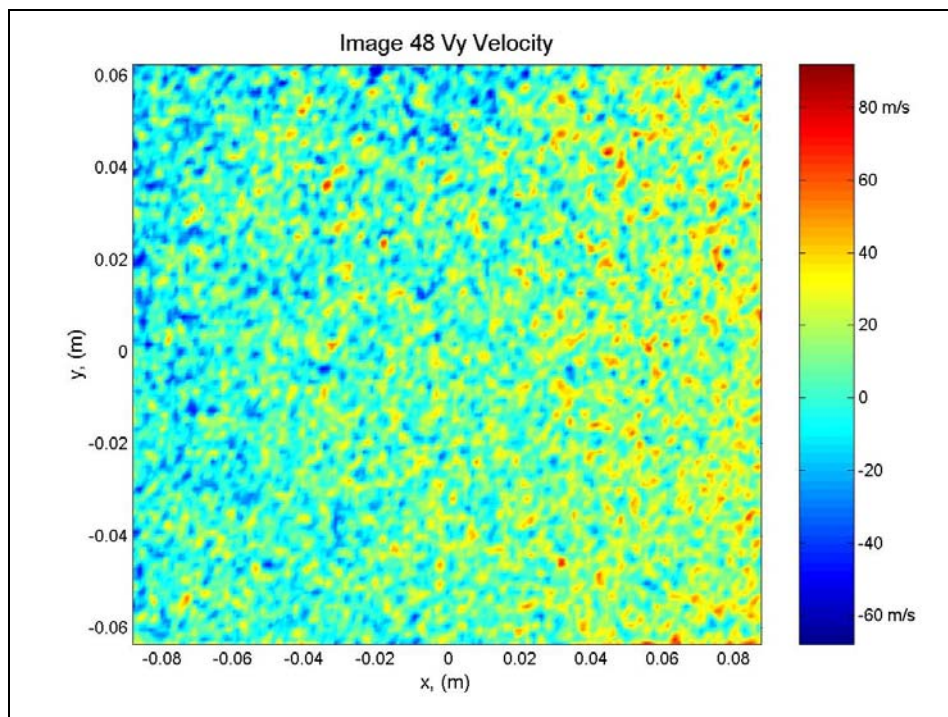
Figure A.20: Contour plot of y velocity components calculated from image 48.
