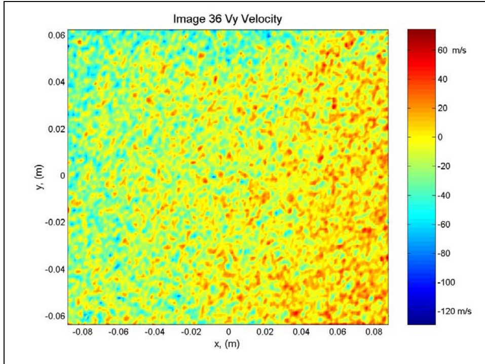
Figure A.11: Contour plot of y velocity components calculated from image 36.
