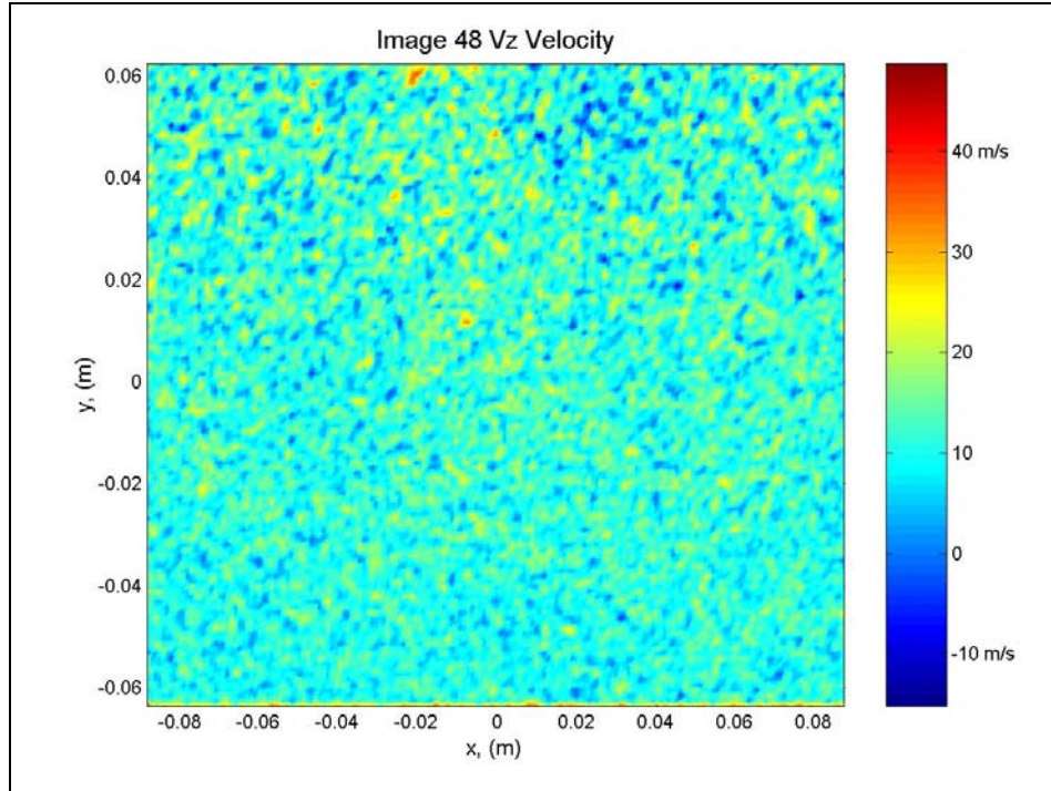
Figure A.21: Contour plot of z velocity components calculated from image 48.
