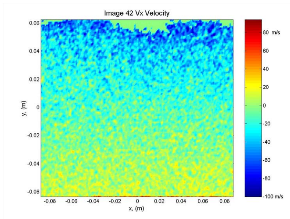
Figure A.16: Contour plot of x velocity components calculated from image 42.
