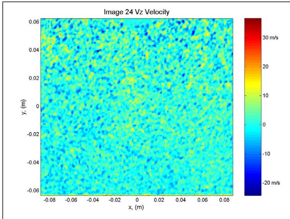
Figure A.9: Contour plot of z velocity components calculated from image 24.
