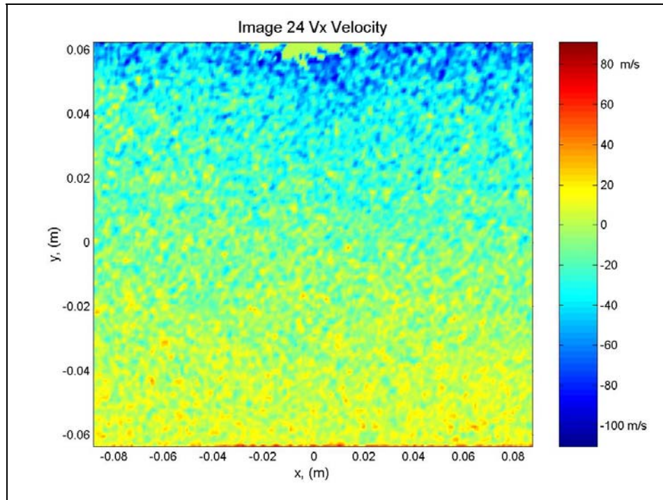
Figure A.7: Contour plot of x velocity components calculated from image 24.
