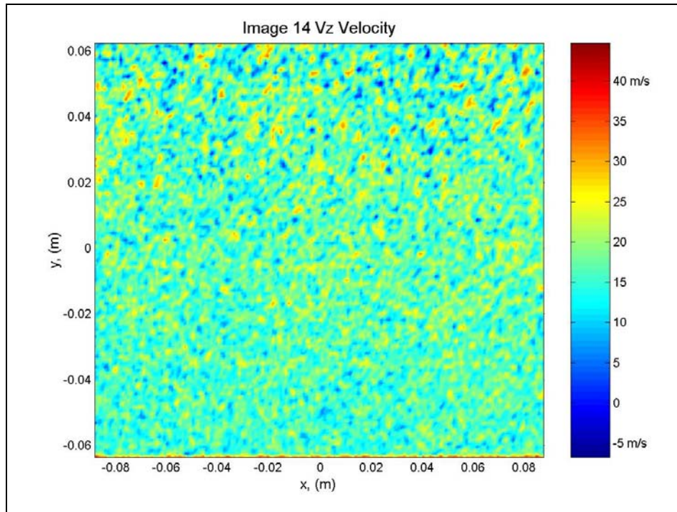
Figure A.3: Contour plot of z velocity components calculated from image 14.
