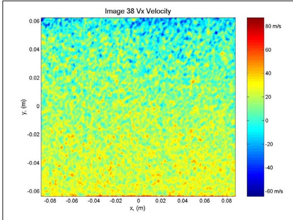
Figure A.13: Contour plot of x velocity components calculated from image 38.
