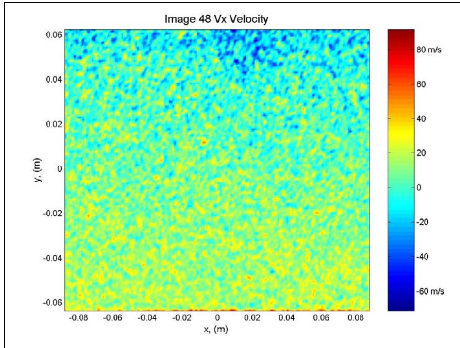
Figure A.19: Contour plot of x velocity components calculated from image 48.
