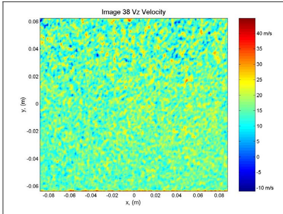
Figure A.15: Contour plot of z velocity components calculated from image 38.
