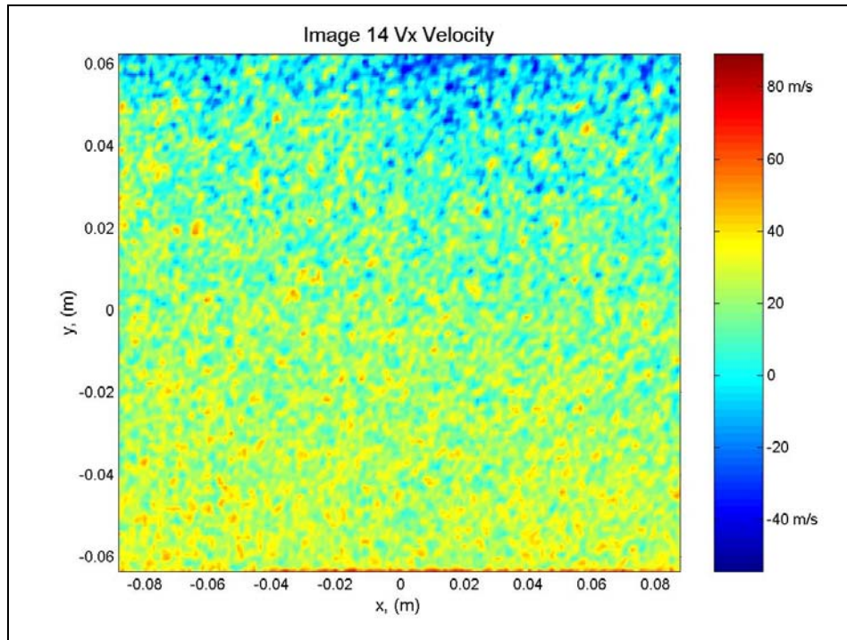
Figure A.1: Contour plot of x velocity components calculated from image 14.
