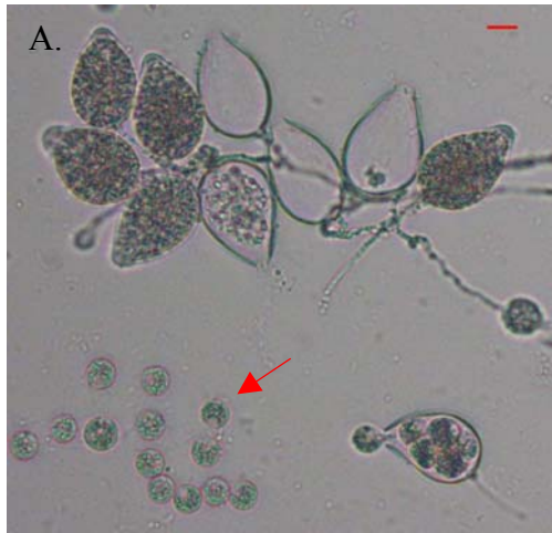
Fig. 21, A-D. Phytophthora citrophthora (103) recovered on non-hymexazol-amended medium in filtering assay from nursery effluent in July 2000. Bar = 10 \mu\text{m} . A. Sporangia on sporangiophores; note encysted zoospores (arrow). B. Papillate sporangium and empty sporangia. C. Papillate sporangium. D. Papillate sporangium with off-center pedicel.
