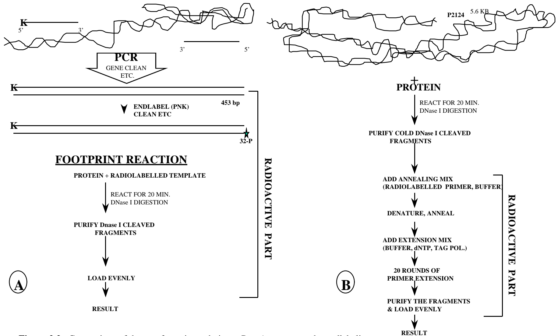
Figure 2.2. Comparison of the two footprint techniques. Part A represents the endlabeling footprint technique and part B shows the primer extension footprinting.
