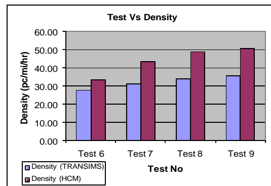
Figure 39: Comparison of Densities for different Test Cases in HCM and TRANSIMS
