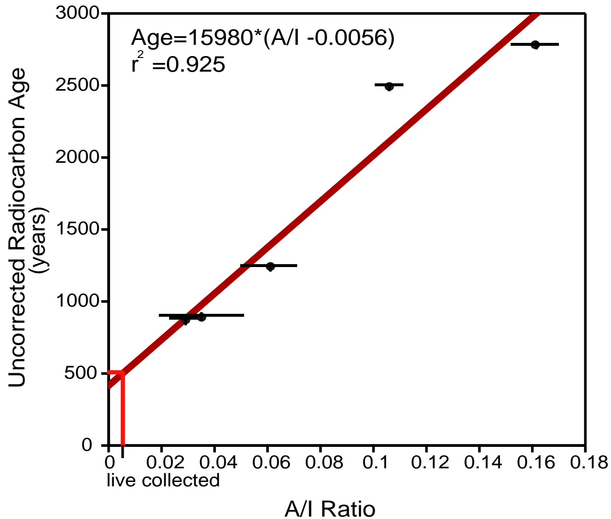
Figure 3.2. Plot of uncorrected radiocarbon age versus A/I ratio. The line represents the best fit correlation with a regression value of r^2=0.925 . Points are average values for shells with standard deviation based on reparations shown. The mean A/I value for live-collected specimens estimates the radiocarbon reservoir age (ca. 510 yr.)
