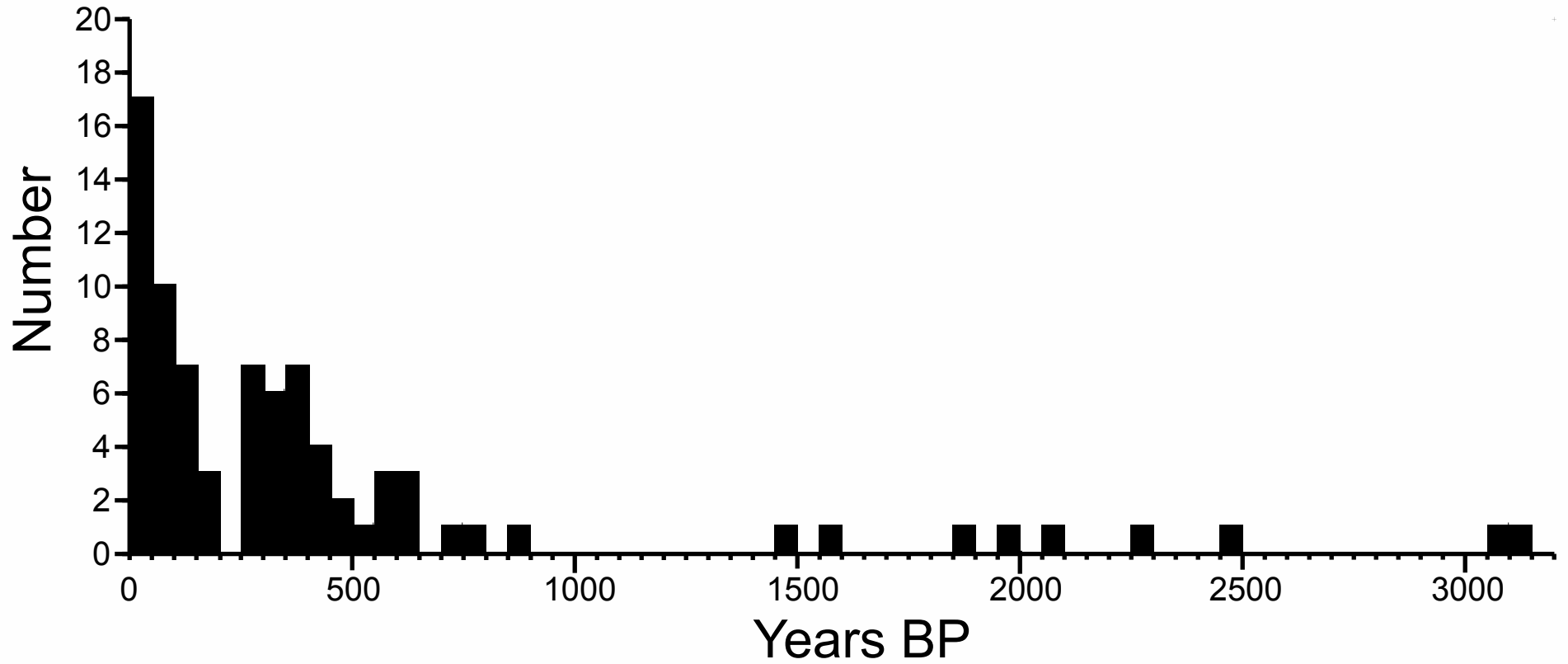
Figure 4.1. Age frequency distribution of brachiopod shells based on calibrated A/I ratios.
