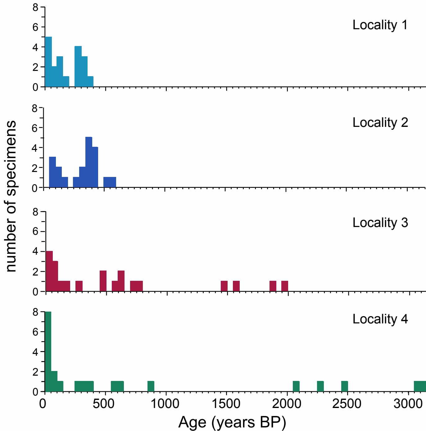
Figure 4.2. Age frequency distributions plotted by locality
