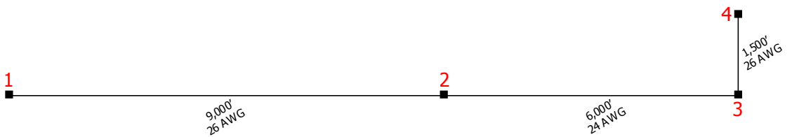
Figure A-3: ANSI Test Loops #1 to #5
