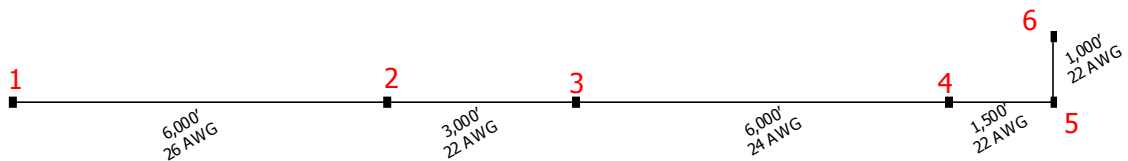
Figure A-4: ANSI Test Loops #6 to #10
