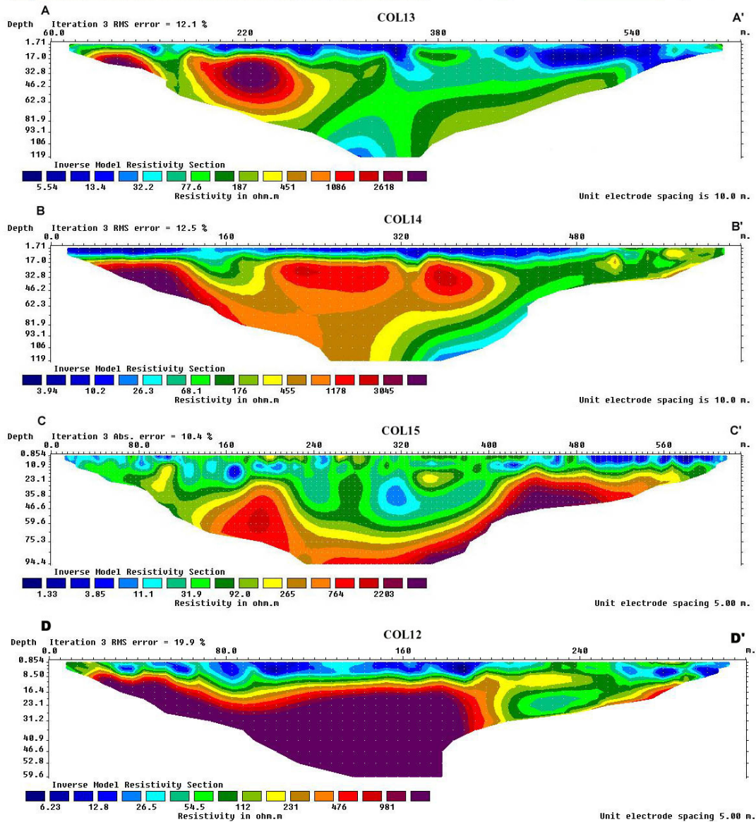
Figure 4.6: Locations and profiles of south spring study area resistivity transects.
