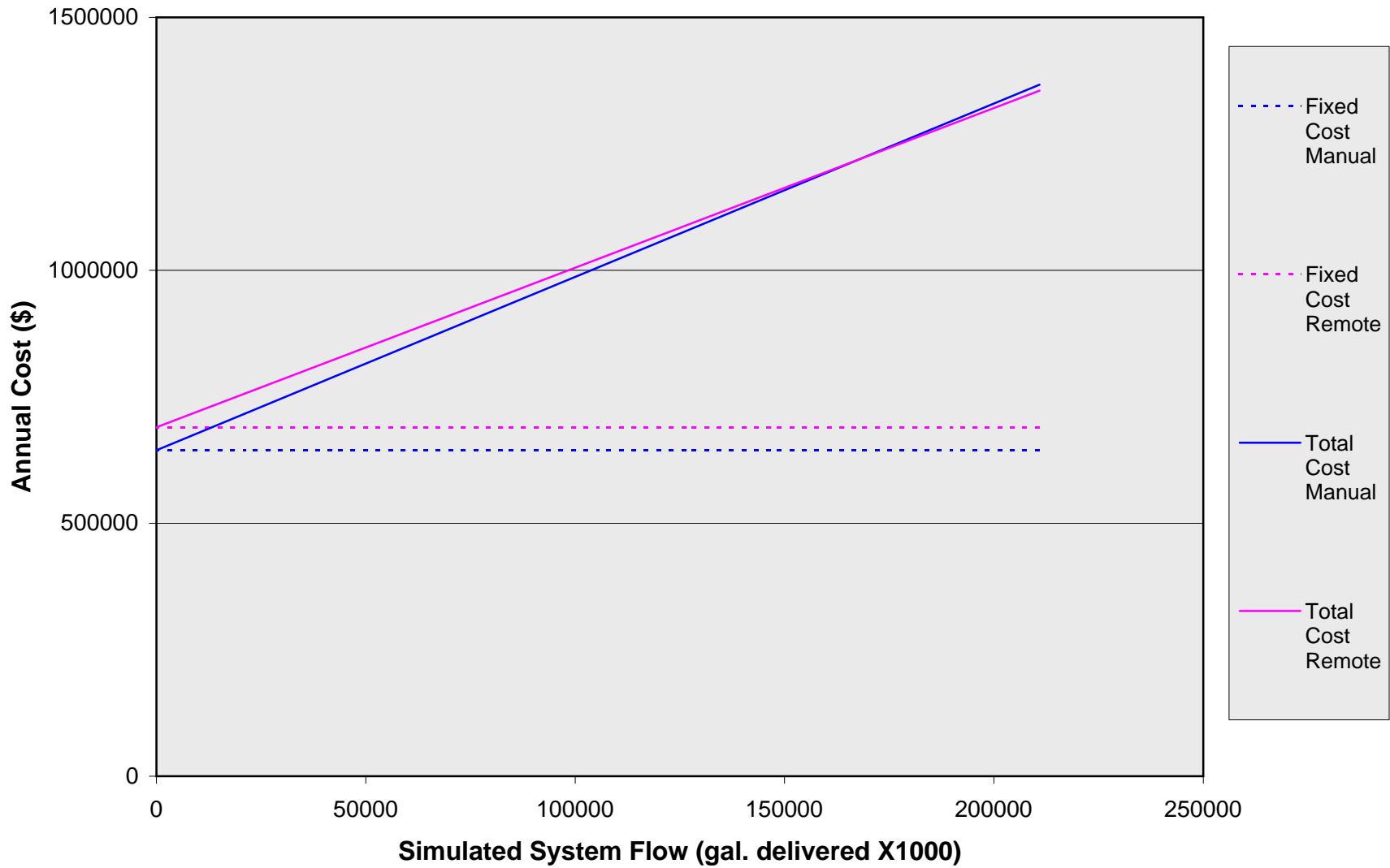
Exhibit 3.19. Sensitivity run 1 (FX = .2) break-even chart.
