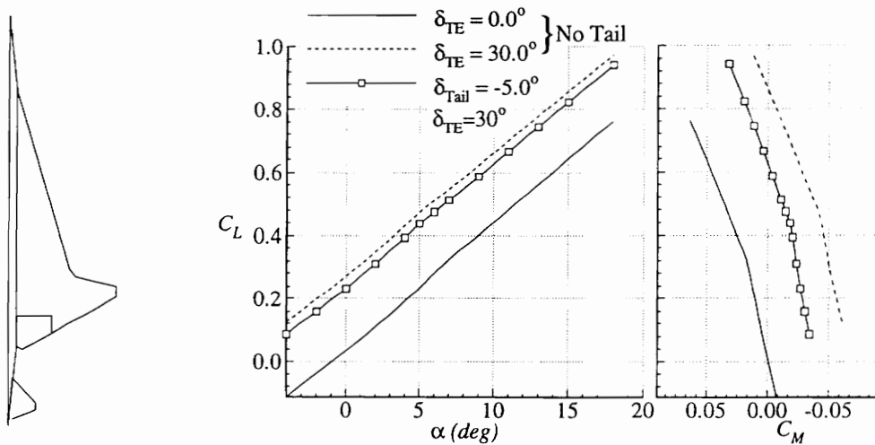
Figure 42. - Aerodynamic performance of a trailing edge flap and horizontal tail combination ( \delta_{Tail} = -5^\circ , \delta_{TE} = 30^\circ ) calculated with the APE method.
