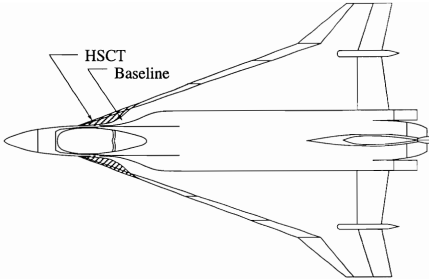
Figure 34. - F-16XL model shown with baseline and HSCT planform configurations.
