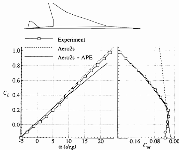
Figure 17. - Comparison of lift and pitching moment estimation methods for a 71^\circ/57^\circ sweep cambered and twisted cranked arrow wing ( \delta_{Tail} = 0^\circ ).
