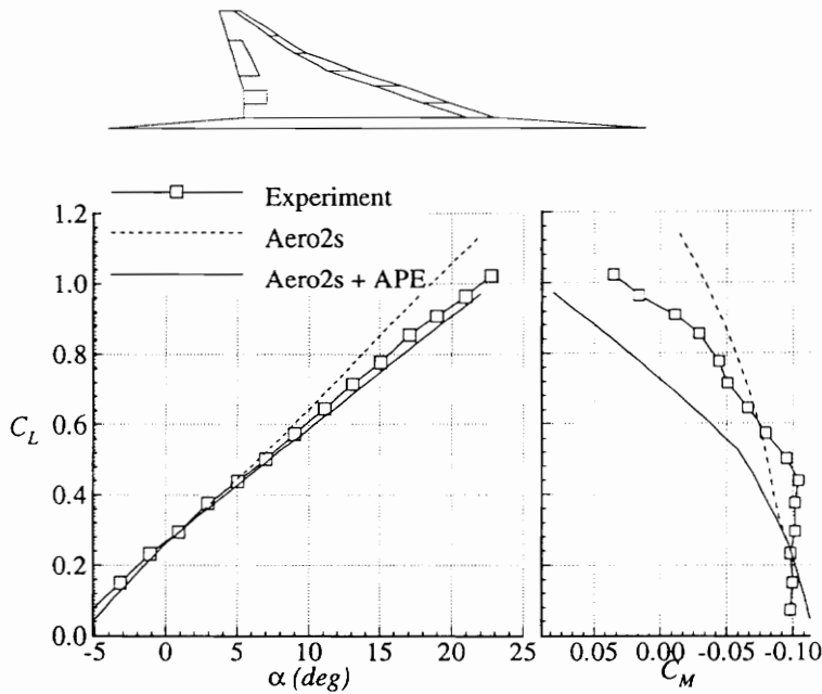
Figure 27. - Comparison of lift and pitching moment estimation methods for a 71^\circ/57^\circ sweep cambered and twisted cranked arrow wing with flaps deflected and tail removed ( \delta_{TE} = 30^\circ , \delta_{LE} = 13^\circ/34^\circ/35^\circ/35^\circ/19^\circ/29^\circ ).
