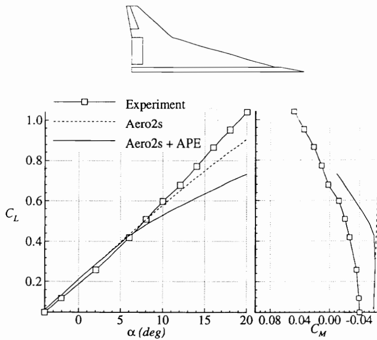
Figure 31. - 74^\circ/48^\circ sweep wing-body combination with trailing edge flaps deflected ( \delta_{TE} = 15^\circ ).
