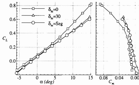
Figure 13. - Effects of a multi-segmented flap for a 74°/70.5°/60° sweep cambered and twisted cranked arrow wing planform (ref. 10).
