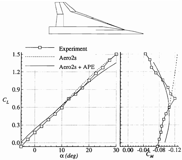
Figure 30. - Comparison of estimation methods for an F-16XL ( 70^\circ/50^\circ sweep) model test ( \delta_{LE} = 28^\circ/38^\circ/40^\circ/20^\circ , \delta_{TE} = 30^\circ/10^\circ ).
