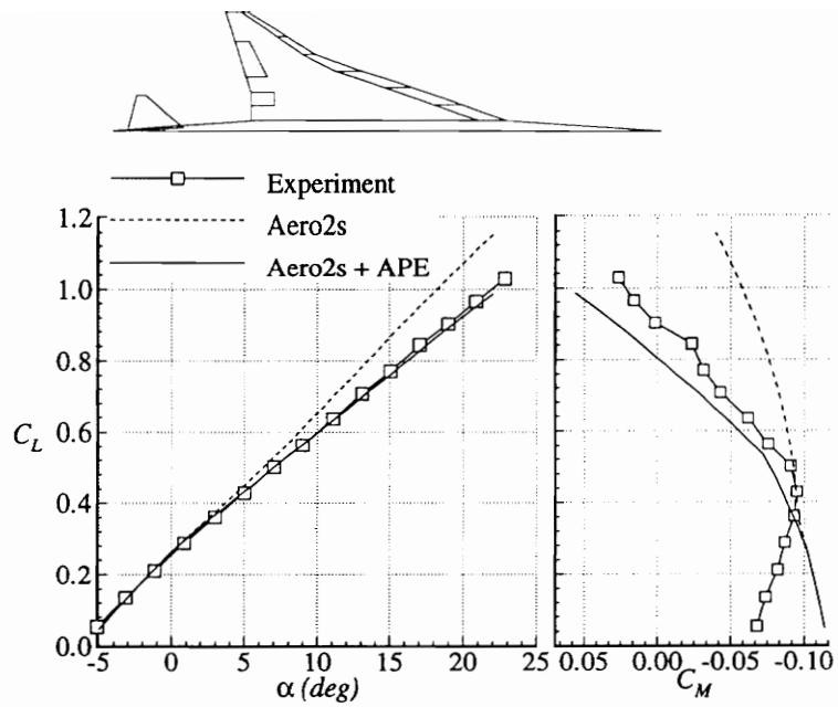
Figure 26. - Comparison of lift and pitching moment estimation methods for a 71^\circ/57^\circ sweep cambered and twisted cranked arrow wing with flaps deflected ( \delta_{Tail} = 0^\circ , \delta_{TE} = 30^\circ , \delta_{LE} = 13^\circ/34^\circ/35^\circ/35^\circ/19^\circ/29^\circ ).
