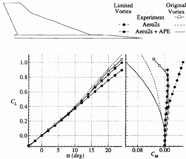
Figure 25. - Effects of limiting the vortex effects to the wing only for a 70°/48.8° sweep uncambered and untwisted cranked arrow wing. Limited vortex begins at wing root and does not to extend into fuselage region.
