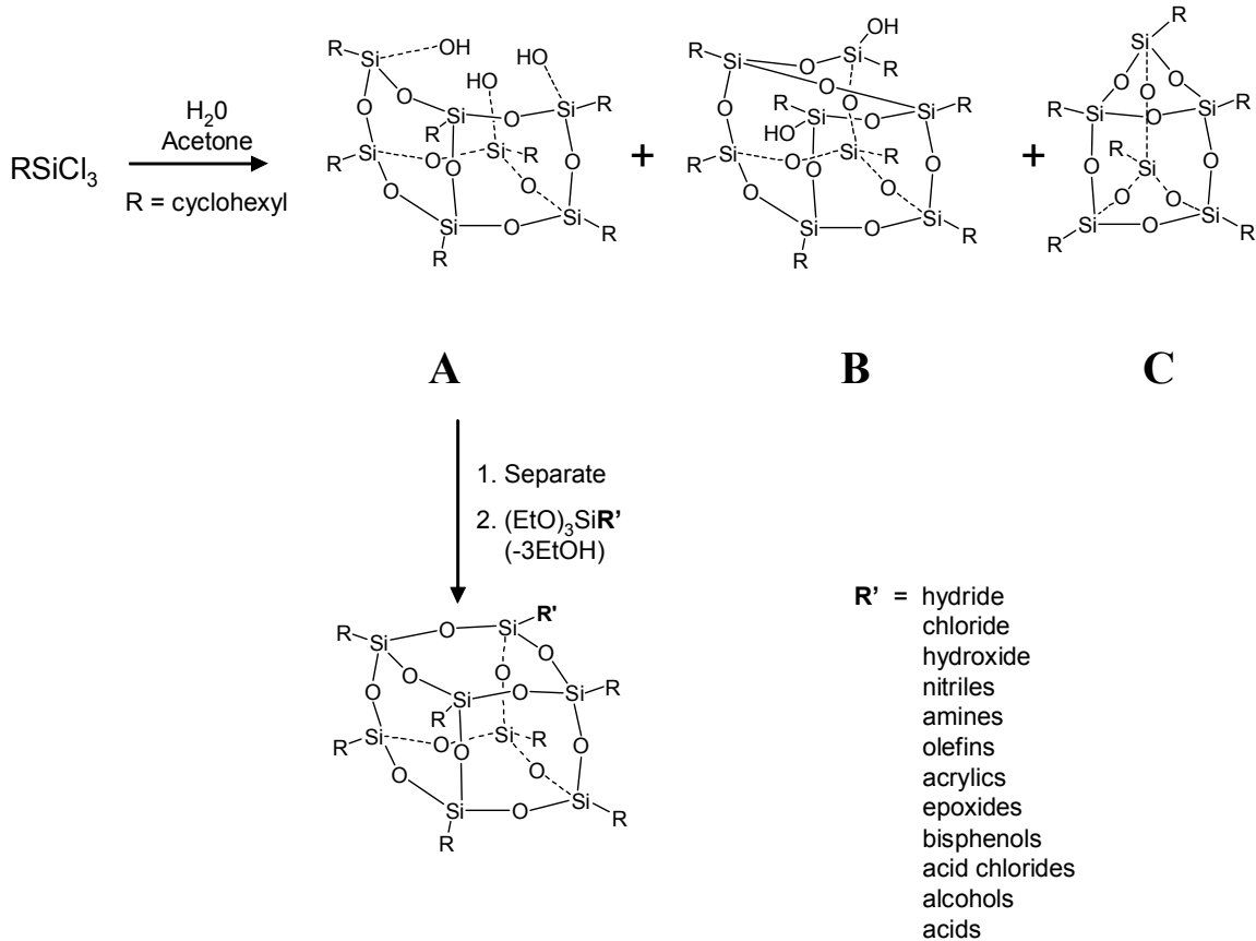
Figure 3.5 Synthesis of heptameric trisilanol (T 7 ) and POSS molecules: A) T 7 , used to create POSS molecules, B) the octameric silanol by-product, and C) the hexameric by-product. 100
