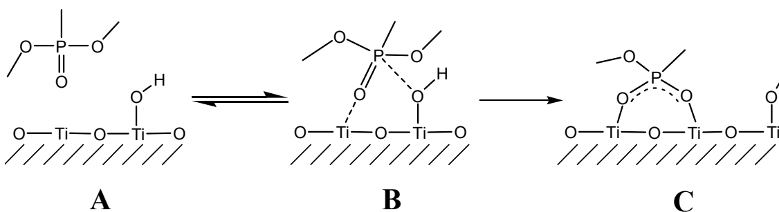
Figure 1.12 Adsorption and decomposition of DMMP onto TiO 2 . A) DMMP approaches the oxide surface. B) Below -73 °C, DMMP molecularly adsorbs to the surface. C) Above -59 °C, DMMP decomposes to form a bridged methylphosphonate species and surface methoxy groups. 30
