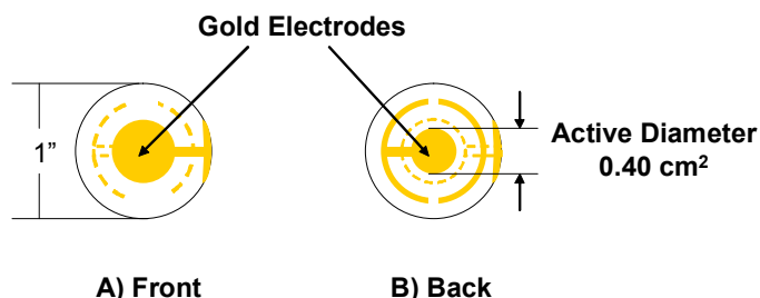
Figure 2.7 Representation of the quartz crystals used. Both sides of the crystal are coated with gold electrodes. A) The front faces the medium of interest. B) The back creates a seal with the crystal holder and is exposed to air.
