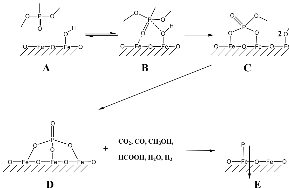
Figure 1.8 The adsorption and decomposition of DMMP on Fe 2 O 3 . A) DMMP approaches the oxide surface. B) At -103 °C, DMMP molecularly adsorbs to the surface. C) At -23 °C, the methyl group is oxidized and DMMP decomposes and bonds to the oxide. D) At 227 °C, the adduct further decomposes to form a tridentate species; all carbon-containing compounds are removed. E) Above 377 °C, phosphorus moves into the bulk, allowing further DMMP adsorption. 17
