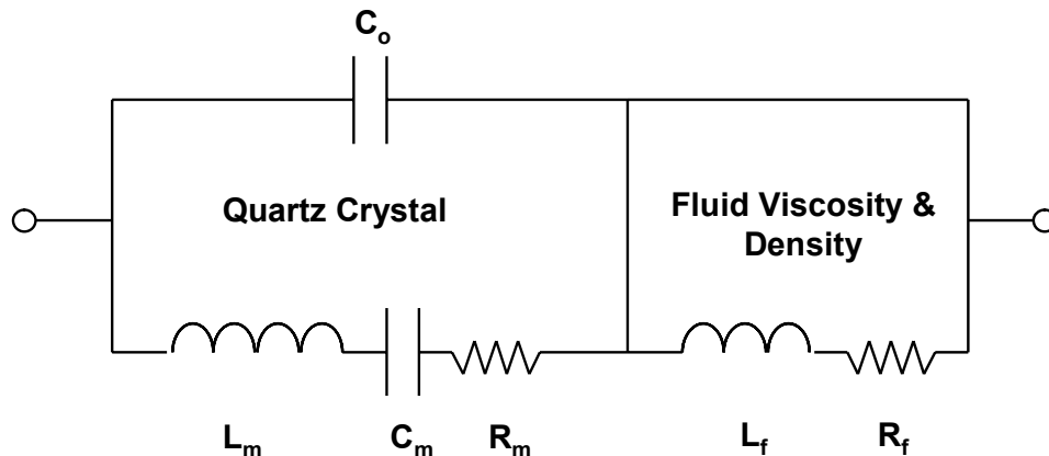
Figure 2.6 Butterworth-van Dyke electrical model for a quartz crystal oscillating near series resonance in a liquid. The density and viscosity of the fluid are accounted for by the addition of an inductor and resistor, respectively.
