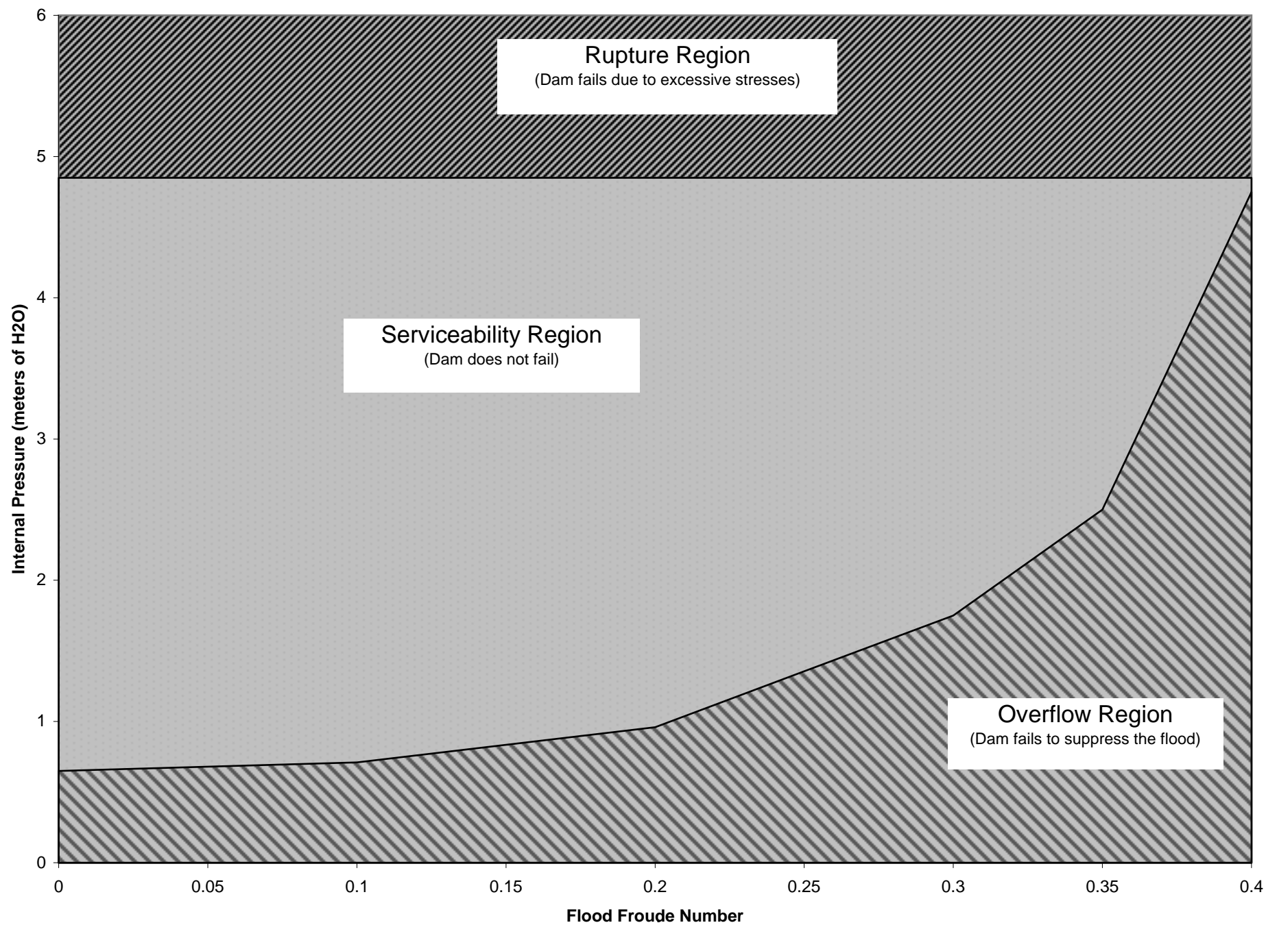
Figure I-15: Serviceability envelope of an inflatable dam subjected to a flood initially at a depth of 3.0 meters
