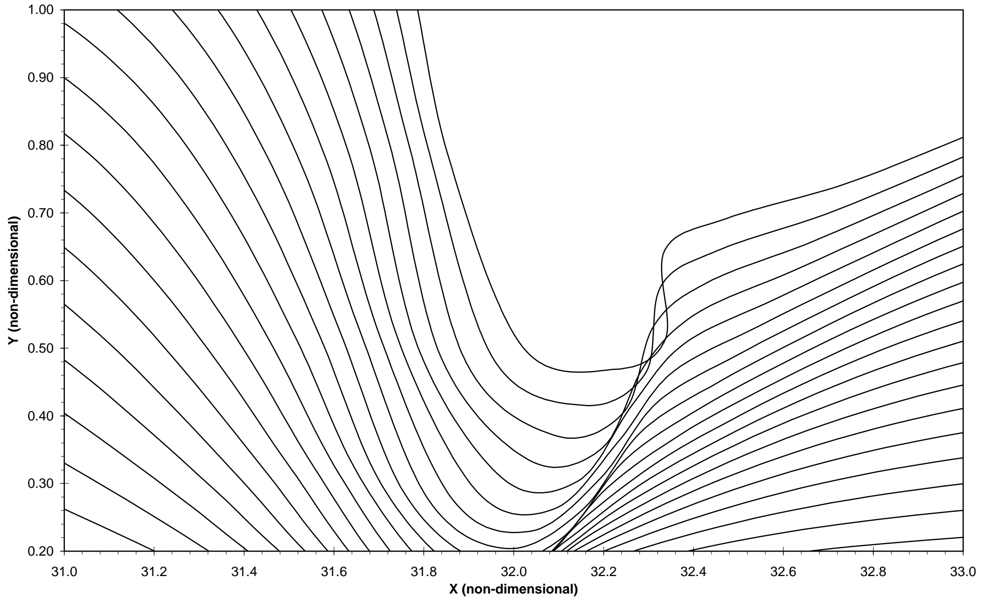
Figure II-10: Sample free surface profile for a surging type breaking wave.
