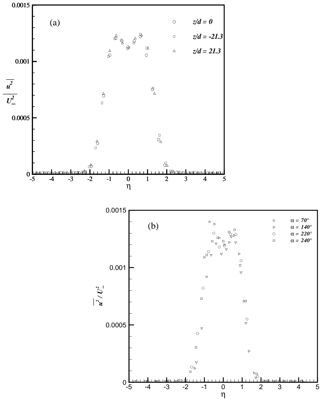
Figure 3.3 Mean-velocity deficit profiles for the plane (a) and ring (b) wakes at x/d = 126
