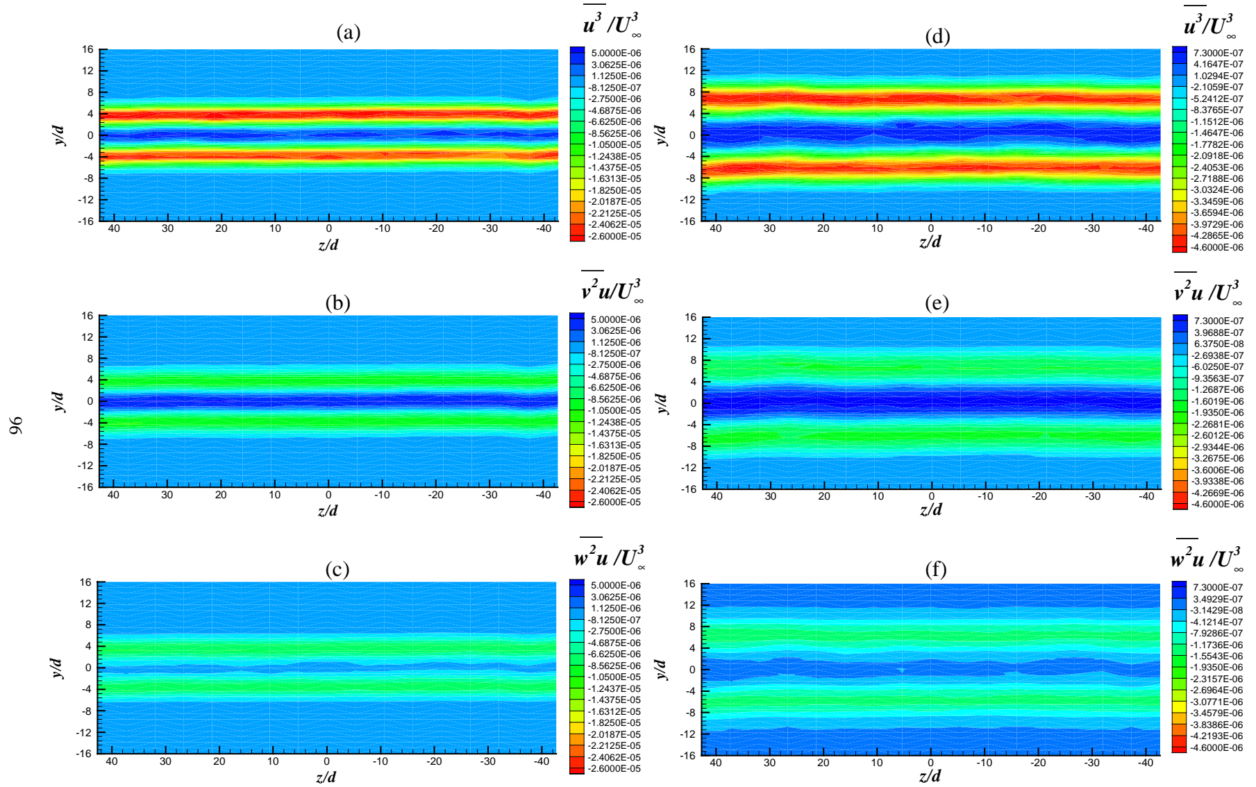
Figure 3.38 Contour plots of the triple turbulent products \overline{u^3}/U_\infty^3 , \overline{v^2u}/U_\infty^3 , and \overline{w^2u}/U_\infty^3 for the plane wake at x/d = 126 in (a), (b), & (c) and at x/d = 450 in (d), (e), & (f)
