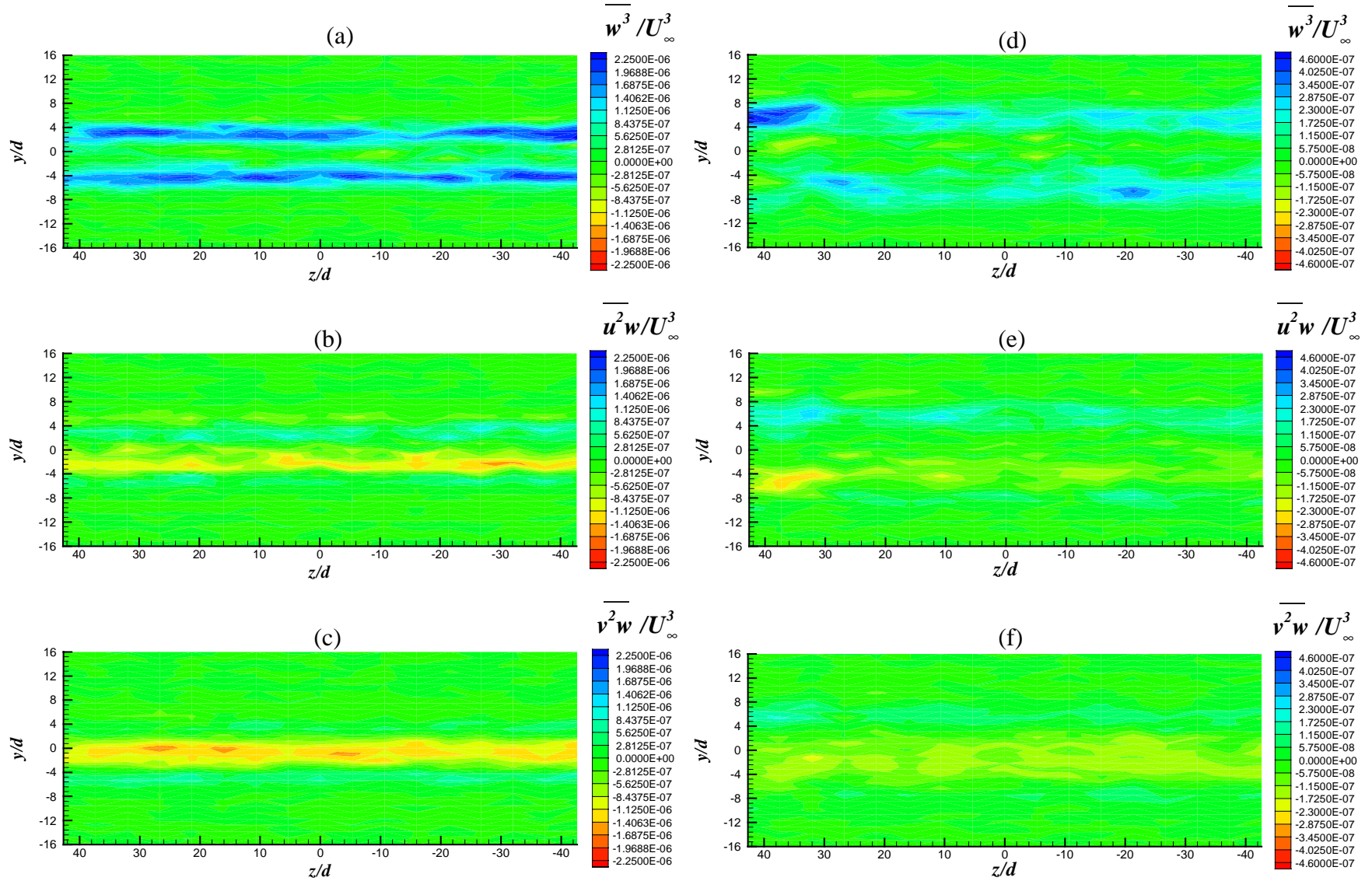
Figure 3.40 Contour plots of the triple turbulent products \overline{w^3}/U_\infty^3 , \overline{u^2 w}/U_\infty^3 , and \overline{v^2 w}/U_\infty^3 for the plane wake at x/d = 126 in (a), (b), & (c) and at x/d = 450 in (d), (e), & (f)
