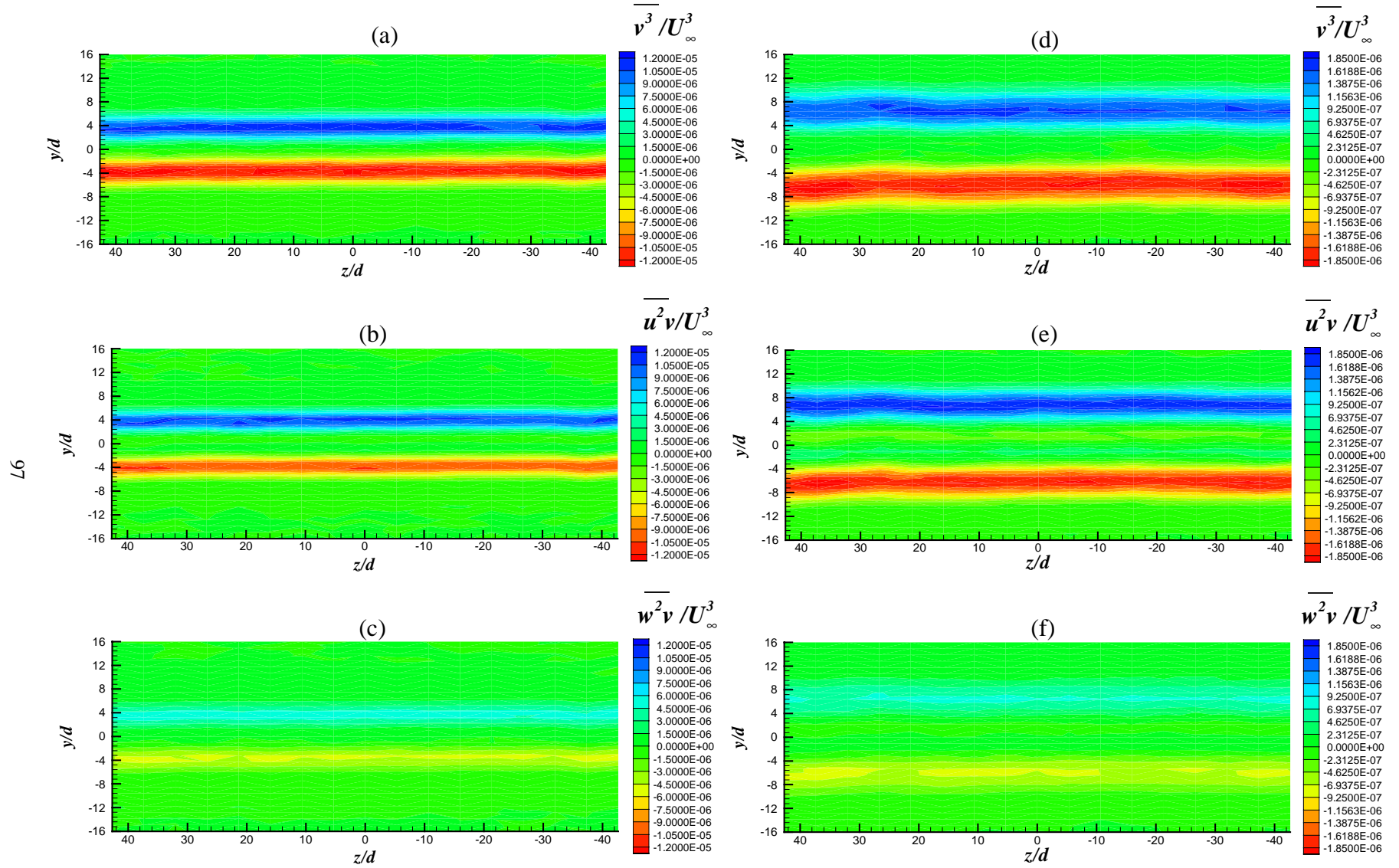
Figure 3.39 Contour plots of the triple turbulent products \overline{v^3}/U_\infty^3 , \overline{u^2v}/U_\infty^3 , and \overline{w^2v}/U_\infty^3 for the plane wake at x/d = 126 in (a), (b), & (c) and at x/d = 450 in (d), (e), & (f)
