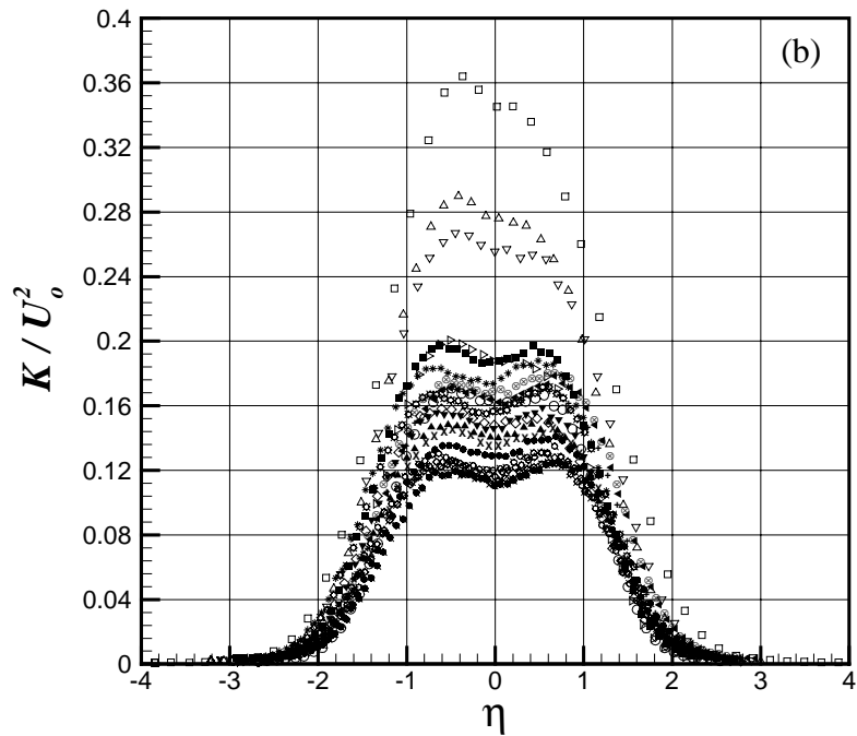
Figure 3.44 Turbulent kinetic energy K/U_0^2 across (a) the plane and (b) the ring wake for 50 \leq x/d < 500
